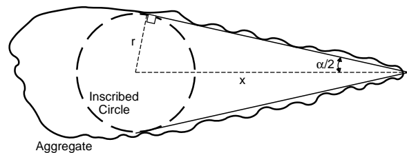
Figure 3. Parameters for determining the degree of angularity. (After Lees 1964.)
