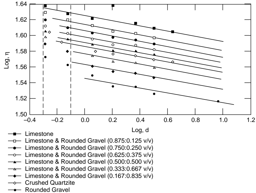
Figure 12. Relationship between mean aggregate diameter and porosity. (After Gupta 1985.)
