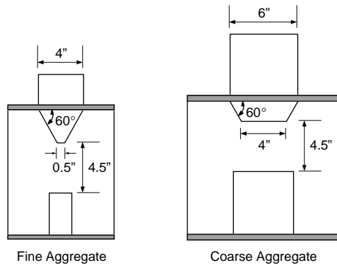
Figure 16. Test apparatus for ASTM C 1252 and modified ASTM C 1252. (After Aldrich 1996.)
