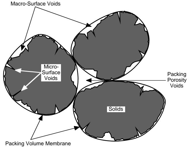
Figure 13. Packing volume, packing porosity, and geometric irregularity of aggregate particles. (After Ishai and Tons 1977.)
