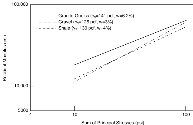
Figure 22. Influence of material type and state of stress on resilient modulus. (After Barksdale and Itani 1994.)
