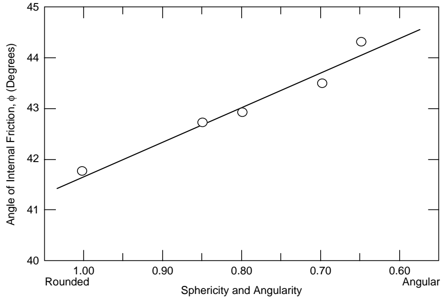
Figure 20. Effect of sphericity and angularity on the angle of internal friction. (After Holubec and Wilson 1970.)
