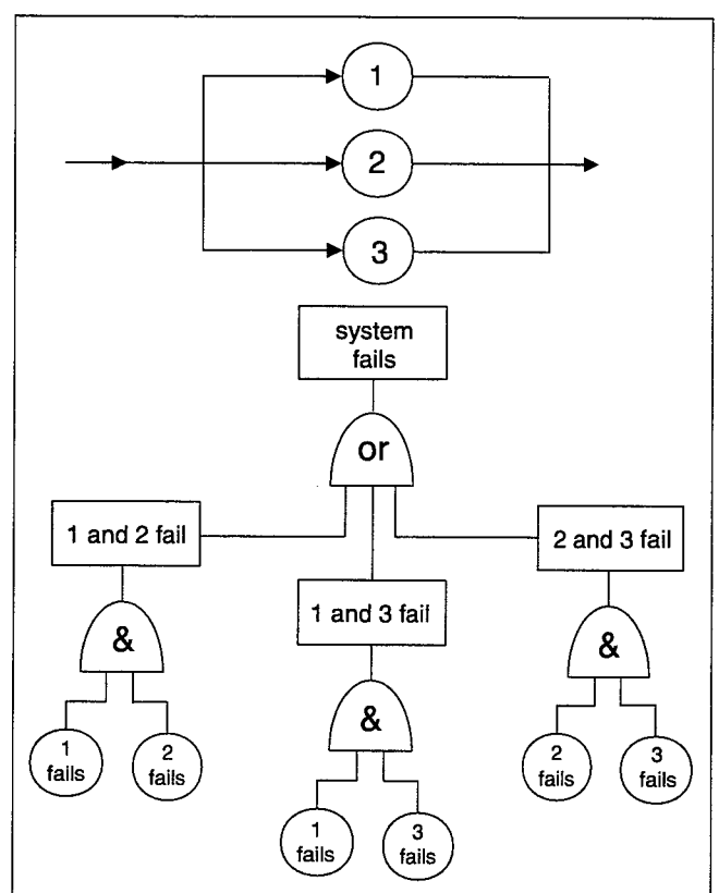
FIGURE E-4 Two-out-of-three system.
