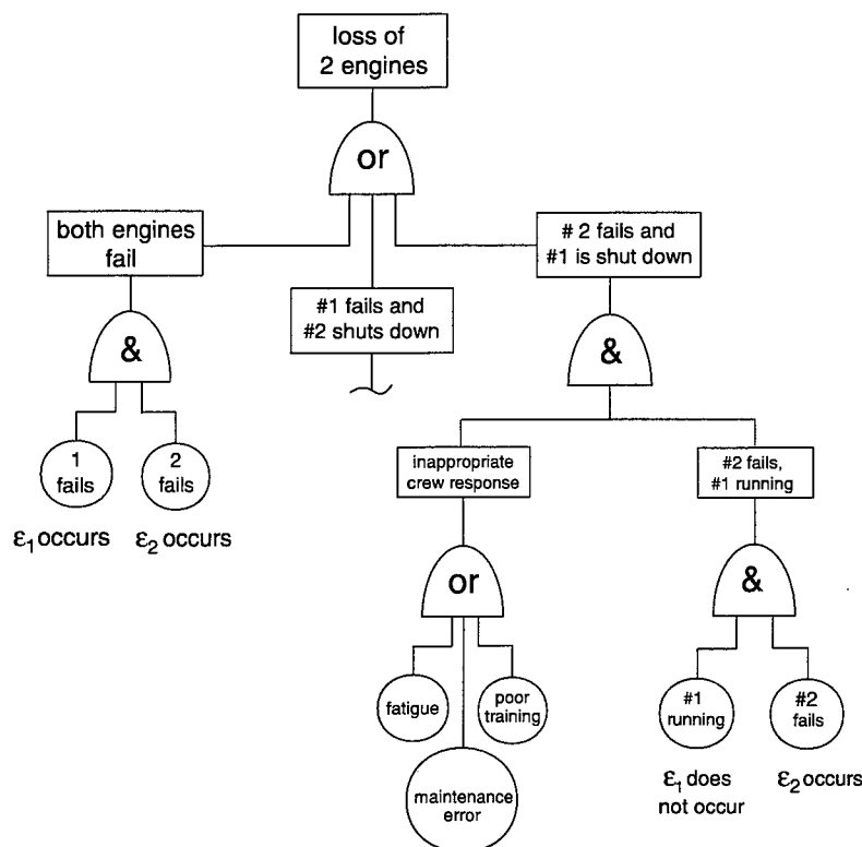
FIGURE E-5 Fault tree diagram of dual-engine failure.
