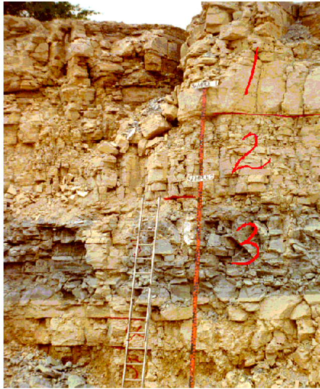
Figure 1. Typical Quarry Face Indicating Lithologic Ledges
