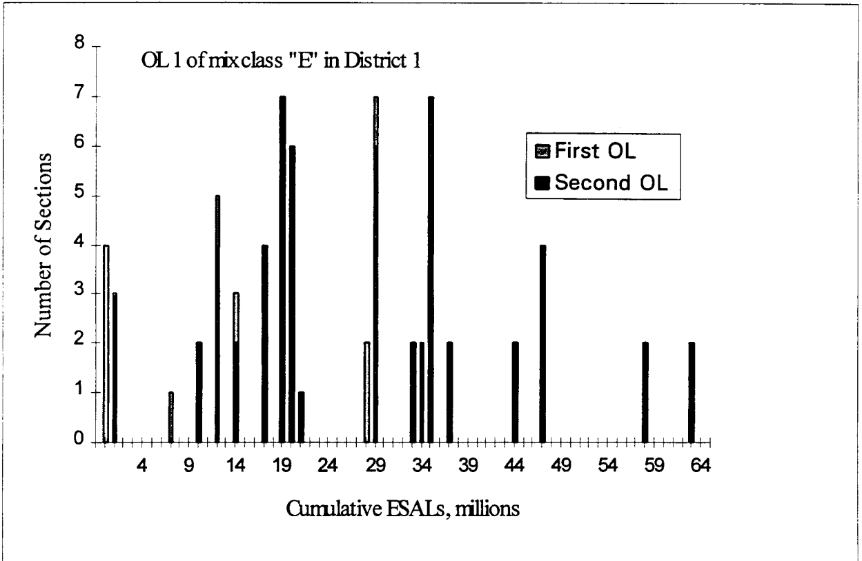
Figure 88. ESAL distribution of first overlays in District 1 with mixture type "E".
