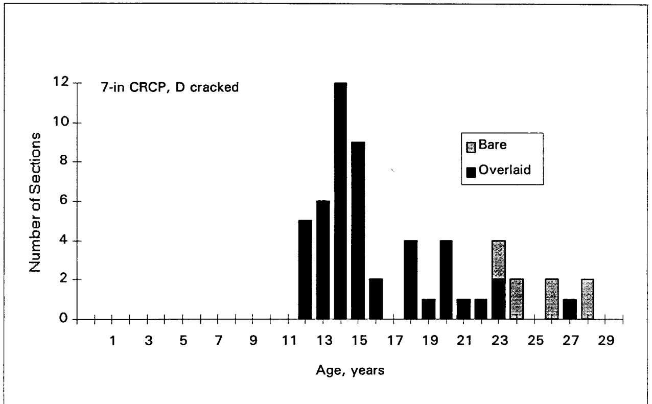
Figure 8. Age distribution of 7-in CRCP with D cracking.
