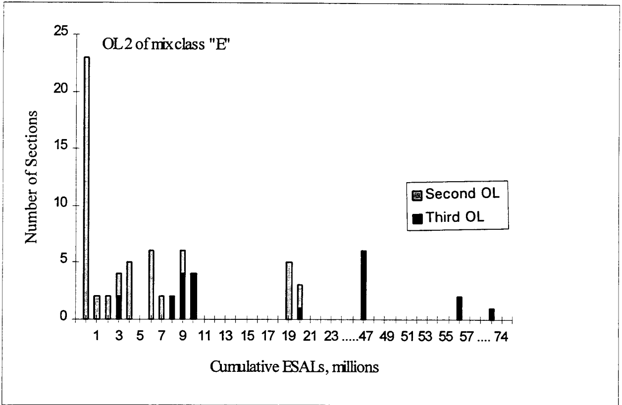
Figure 82. ESAL distribution of second overlays, in all districts, with mixture type "E".
