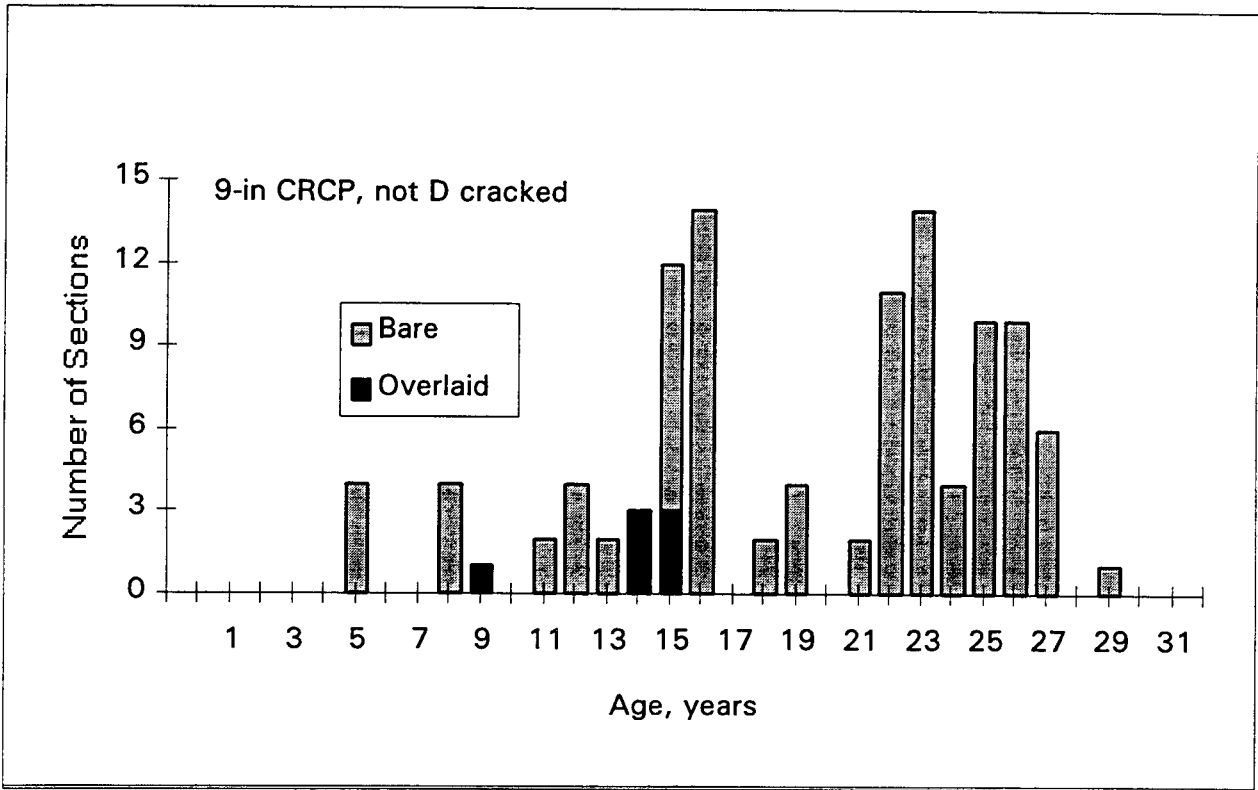
Figure 19. Age distribution of 9-in CRCP without D cracking.
