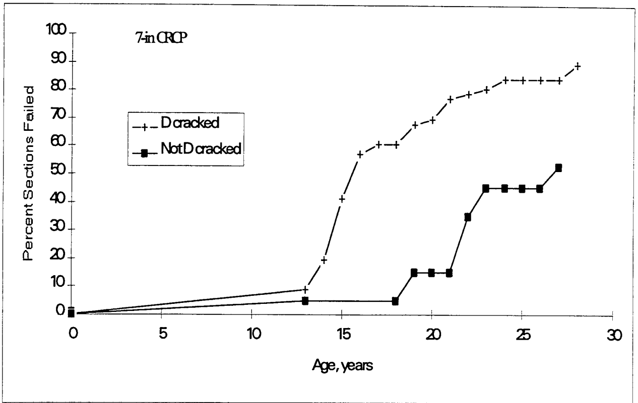
Figure 11. Age survival curves for 7-in CRCP.
