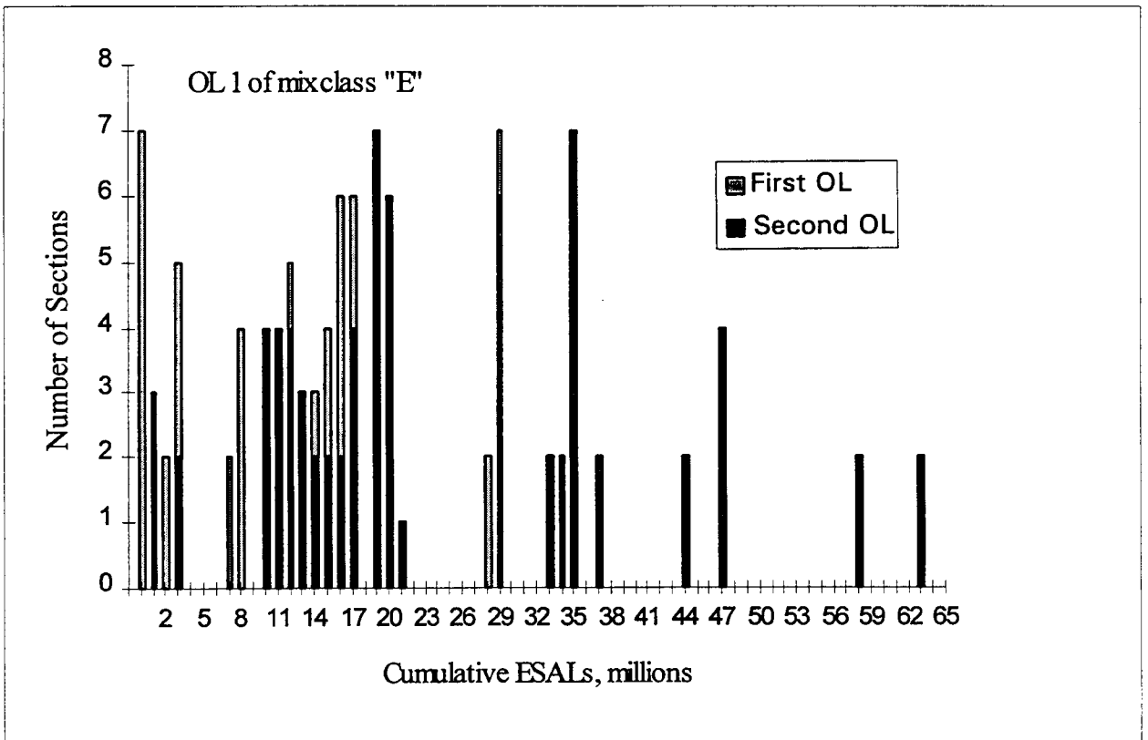
Figure 76. ESAL distribution of first overlays, in all districts, with mixture type "E".
