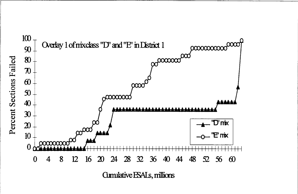
Figure 90. ESAL survival curves for first overlays in District 1 with mixture types "D" and "E".
