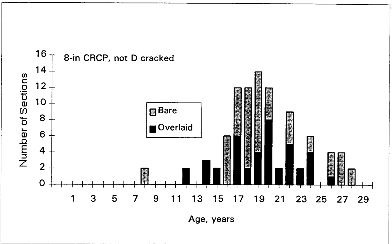
Figure 13. Age distribution of 8-in CRCP without D cracking.
