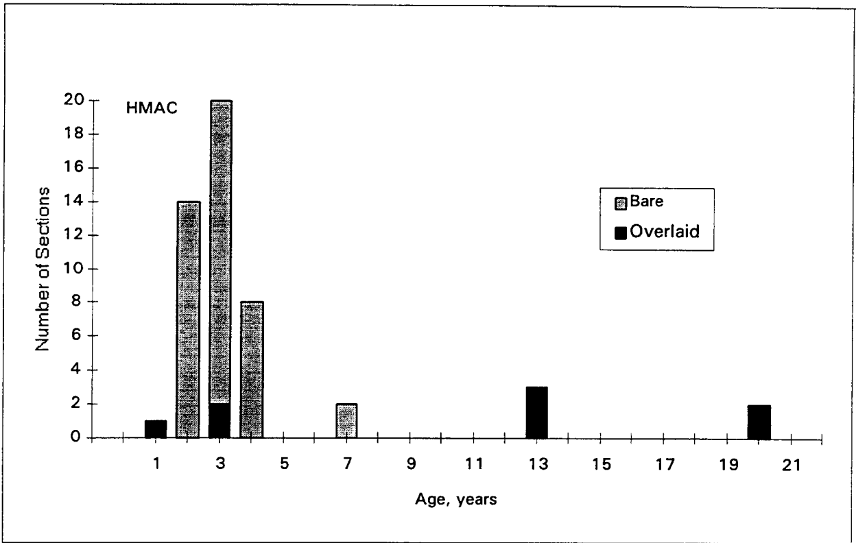
Figure 29. Age distribution of HMAC.
