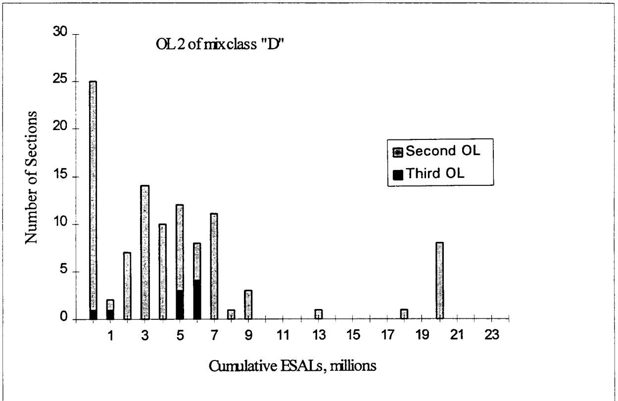
Figure 80. ESAL distribution of second overlays, in all districts, with mixture type "D".
