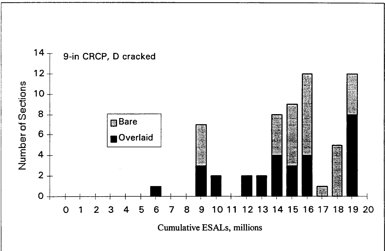
Figure 22. ESAL distribution of 9-in CRCP with D cracking.
