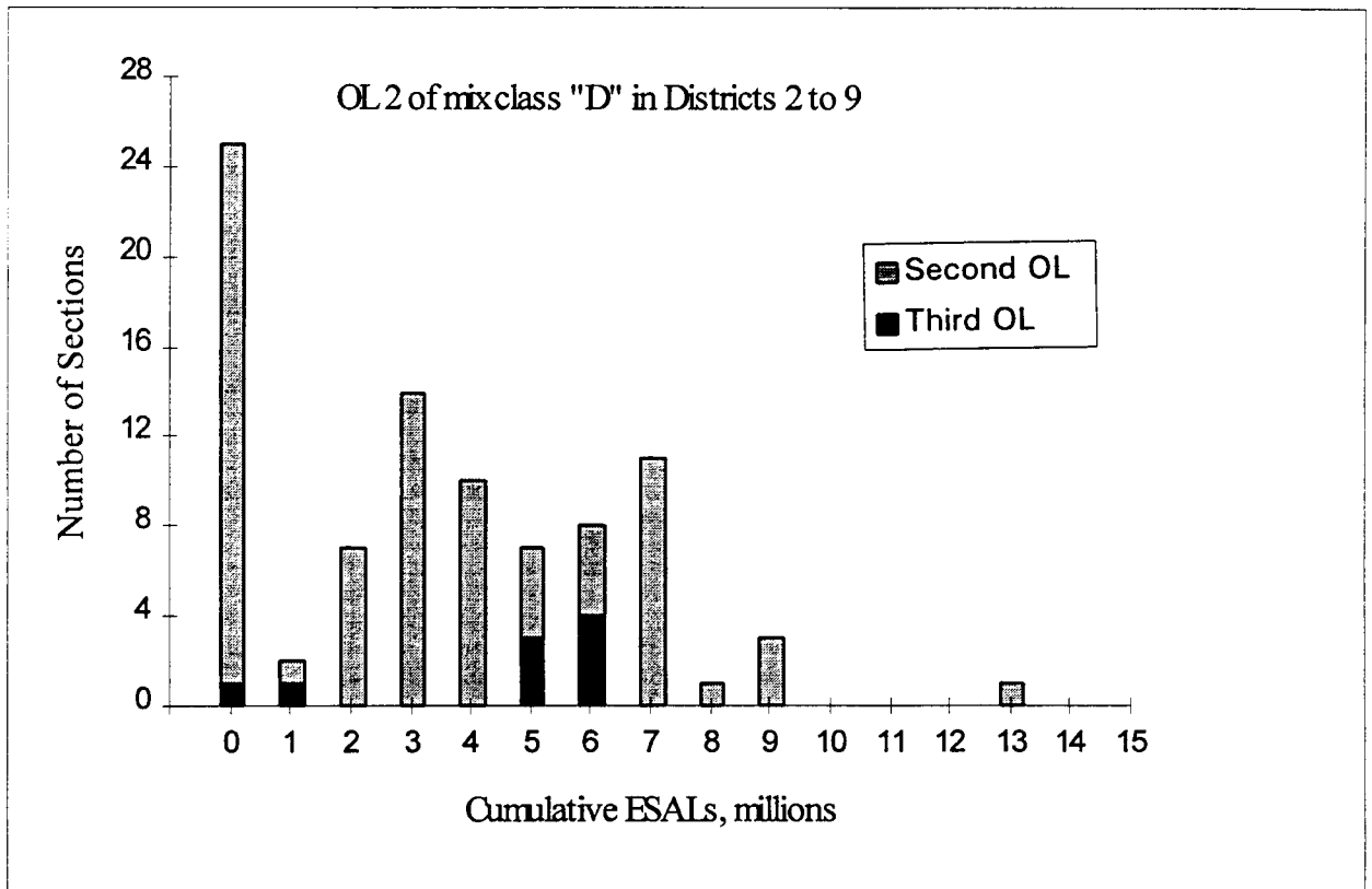
Figure 104. ESAL distribution for second overlays in districts 2 to 9 with mixture type "D".
