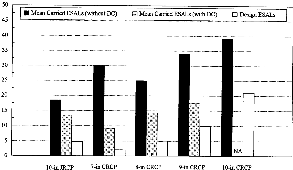
Figure 18. Mean carried ESALs versus design ESALs for original pavements.
