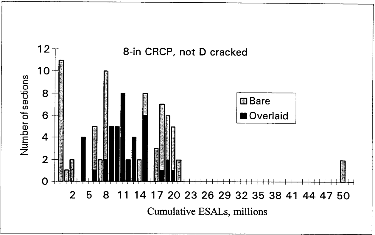
Figure 15. ESAL distribution of 8-in CRCP without D cracking.
