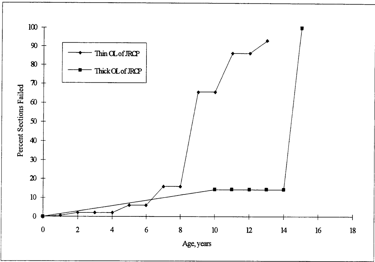
Figure 8. Age survival curve for thin AC overlays of JRCP (second overlay).
