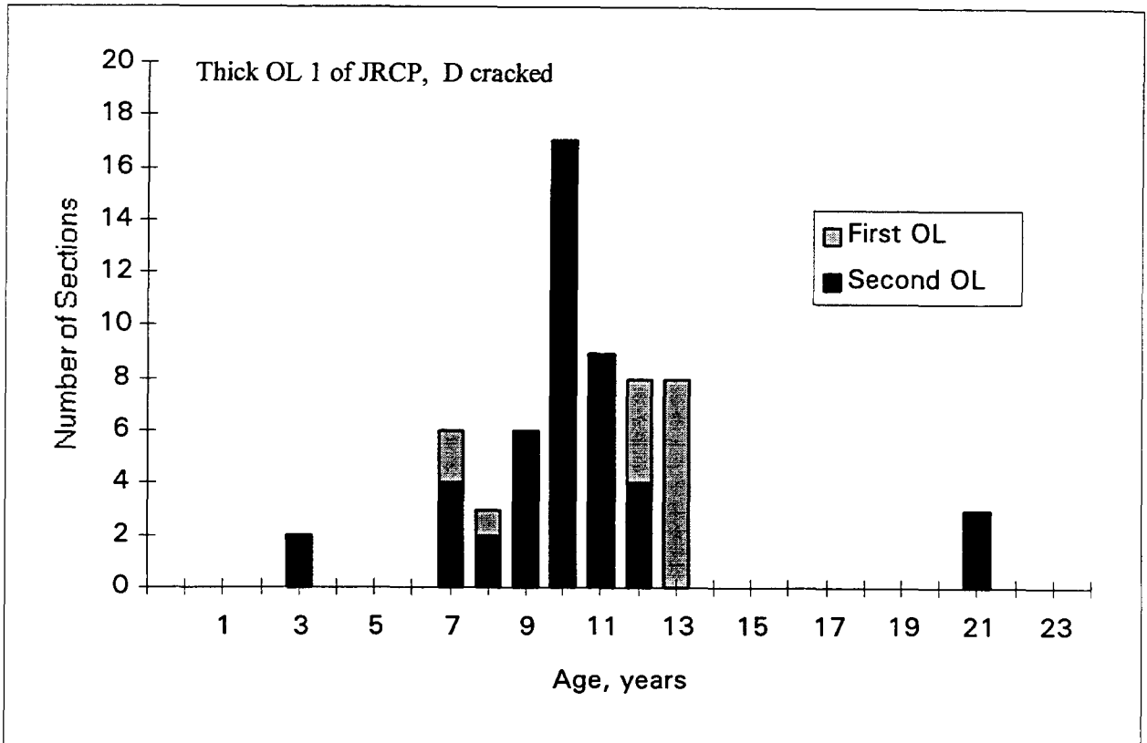
Figure 40. Age distribution for first (thick) AC overlays over JRCP, with D cracking.
