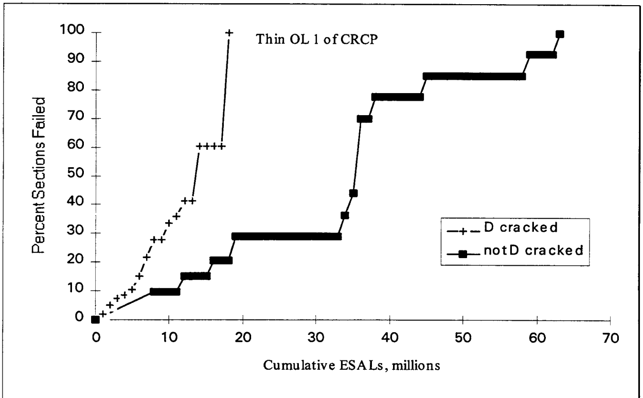
Figure 50. ESAL survival curves for first (thin) AC overlays over CRCP.
