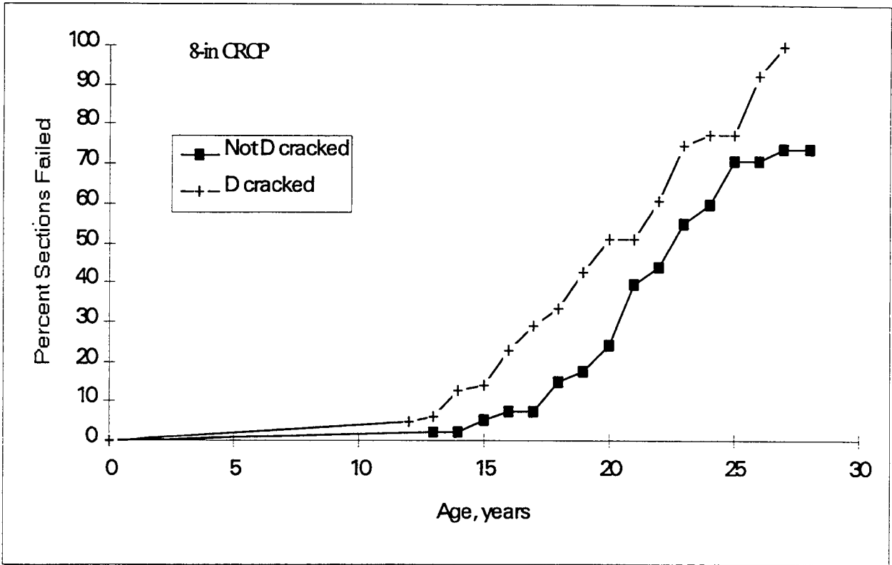
Figure 17. Age survival curves for 8-in CRCP.
