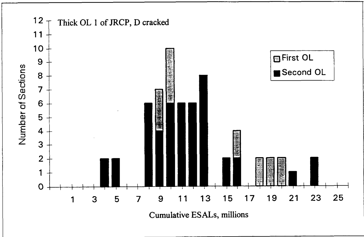
Figure 42. ESAL distribution for first (thick) AC overlays over JRCP, with D cracking.
