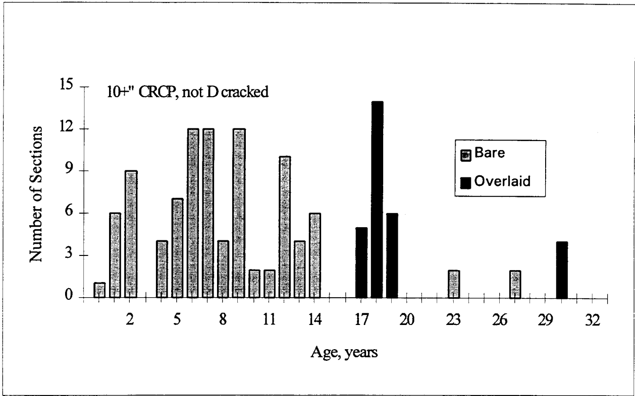
Figure 25. Age distribution of 10-in or more CRCP without D cracking.
