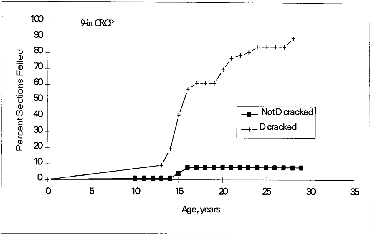
Figure 23. Age survival curves for 9-in CRCP.
