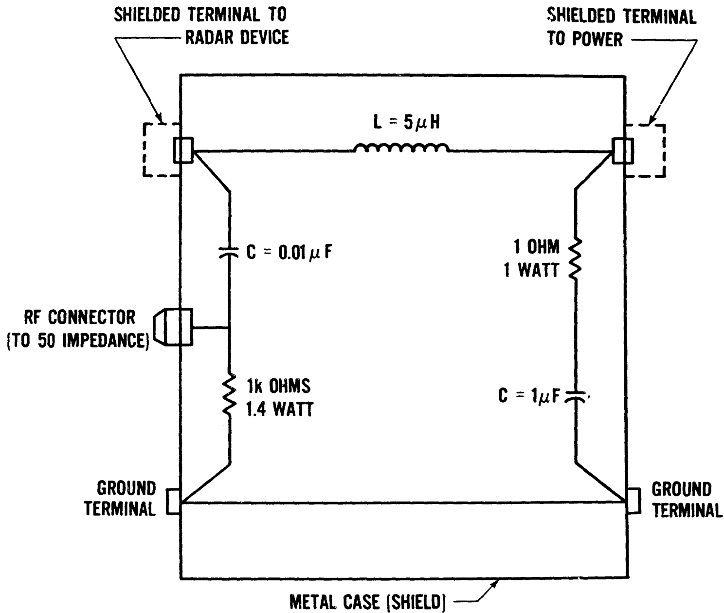
Figure No. 1 Line impedance stabilization network (LISN).
