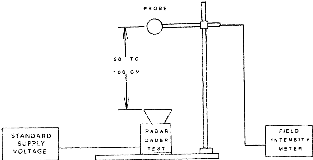
Figure No. 5 Block diagram for antenna beam width measurement.
