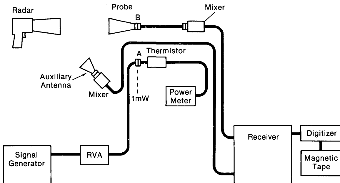
Figure 2. Schematic diagram of measurement system used to determine power density. As shown here, the system is connected for measuring the probe output produced by an incident electromagnetic field. The auxiliary antenna and circuit provide a stable reference signal to which the receiver is phase locked. A 1 mW calibrating signal is established at point A by means of the calibrated thermistor, power meter, and rotary-vane attenuator (RVA).
