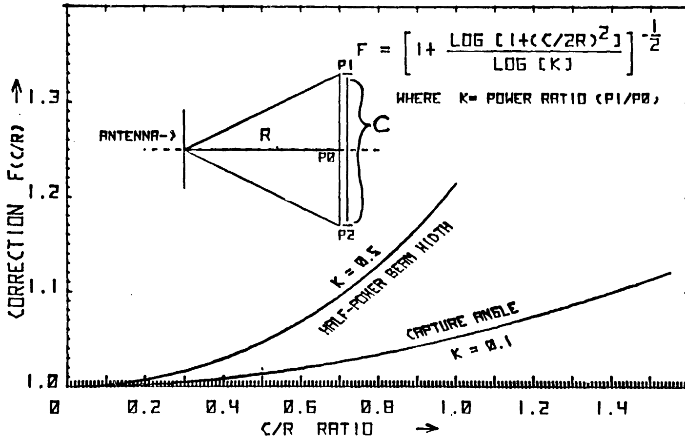
Figure No. 6 Antenna beam width correction factor, f^\circ .
