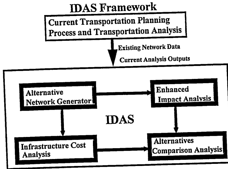
Figure 1—IDAS Framework
