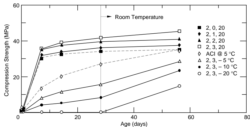
Figure 2. Effect of temperature on strength gain of concrete. The dotted lines show the strength gain of control concrete at 20°C (70°F) and 5°C (40°F). The 5°C (40°F) line is based on guidance from ACI (1988). All results are for concrete made with a 365-kg/m 3 (611 lb/yd 3 ) cement factor cured at a given temperature for 28 days, followed by 28 days of curing at room temperature.
