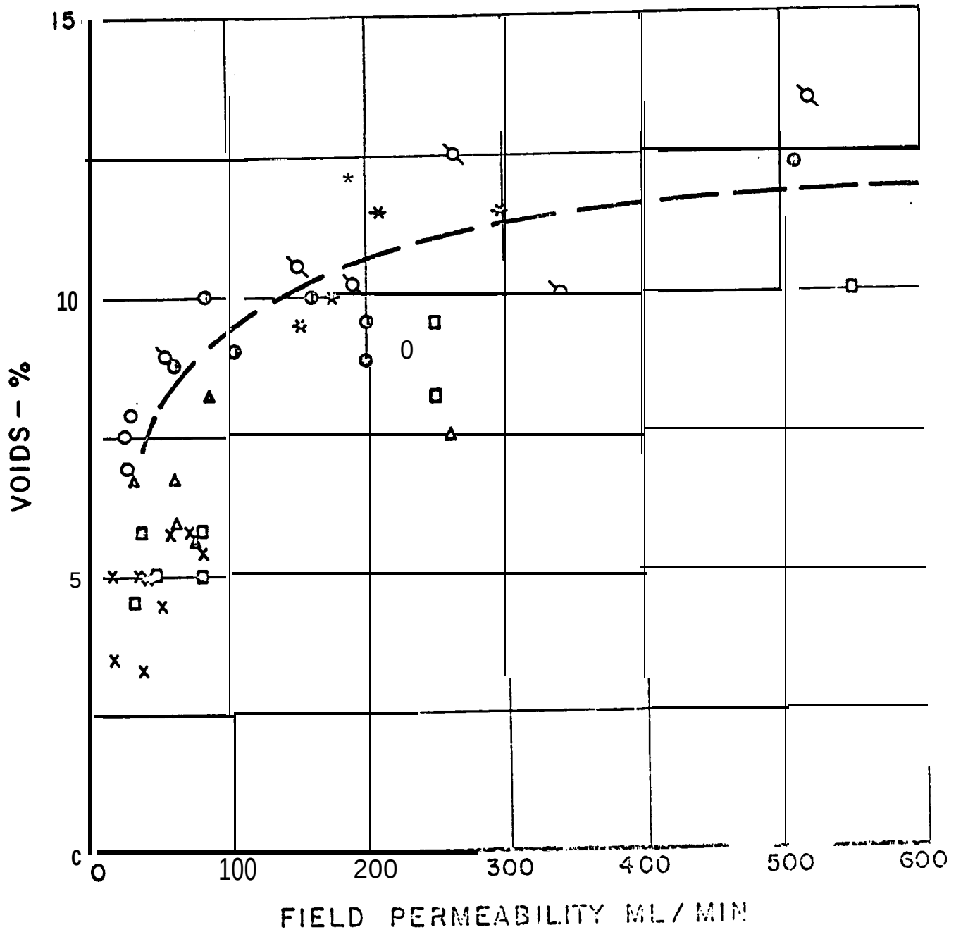
Figure 3. Relationships between air voids and permeability (after Zube) in California study.
