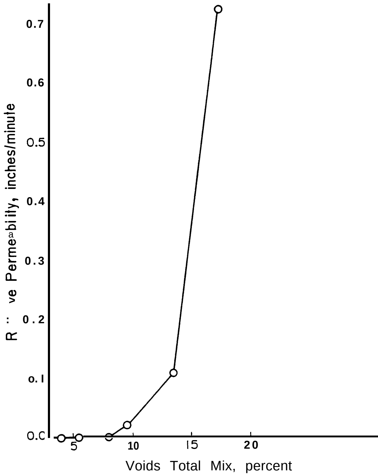
Figure 4. Relationship between air voids and permeability in Georgia Study (after Brown, Collins, and Brownfield).
