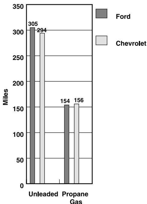
Figure 16. The driving range of propane gas and control vans (on a typical FedEx duty cycle at 40 miles per day) was estimated.
