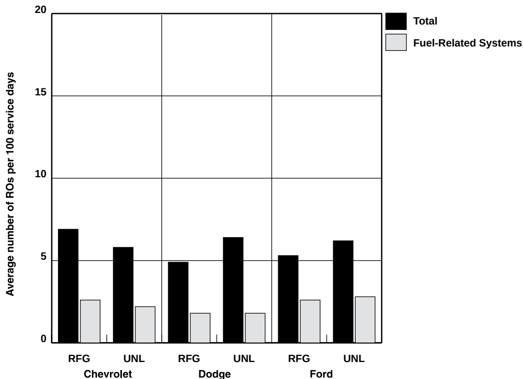
Figure 26. The number of repair orders per 100 days of service for the total van and fuel-related systems is compared for RFG and control vans.
