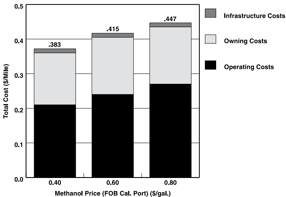
Figure 38. Costs were estimated for an M-85 fleet in a 1996 economic case study.
