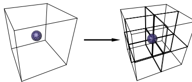
Figure 2.1: Cell Dividing into 8 Children
