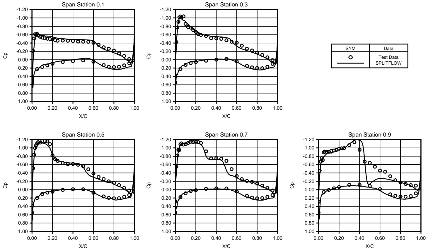
Figure 6.6: Wing C Solution
