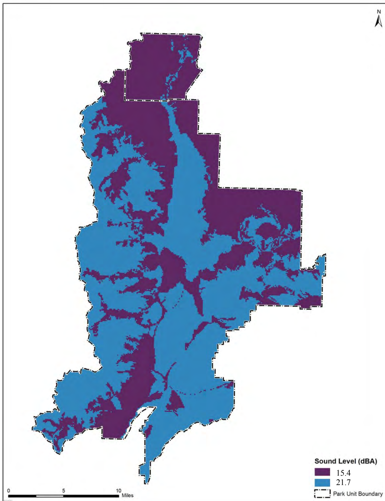
Figure 2: Grand Teton natural ambient map
