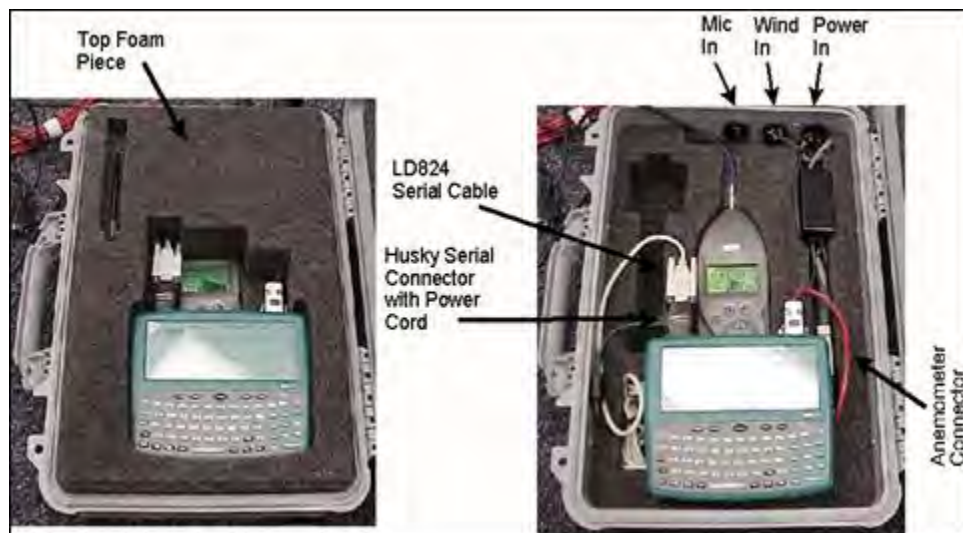
Figure 66. SLM acoustics case.
