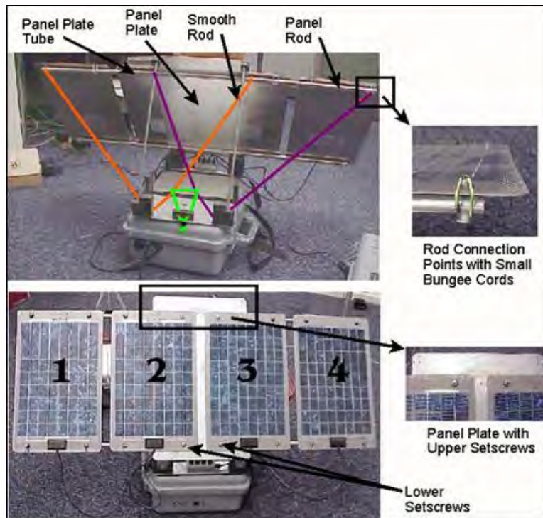
Figure 64. Solar panel array setup.
