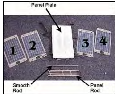
Figure 63. Unpack solar array.
