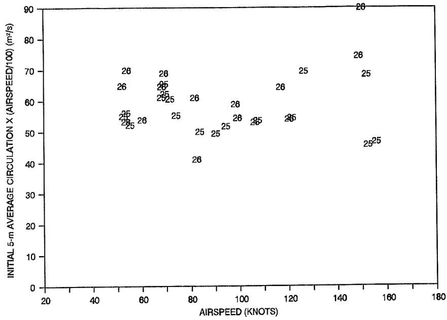
FIGURE 4-6. UH-60A 5-M INITIAL AVERAGE CIRCULATION X (V/100) VS. AIRSPEED (KNOTS)
