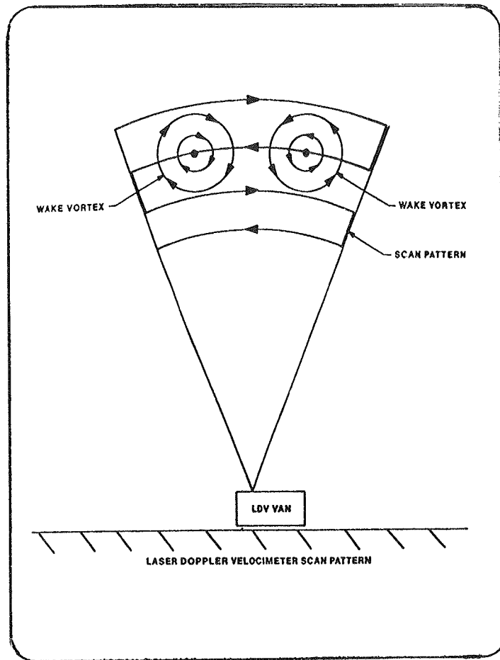
FIGURE 3-5. LDV SCAN METHODOLOGY
