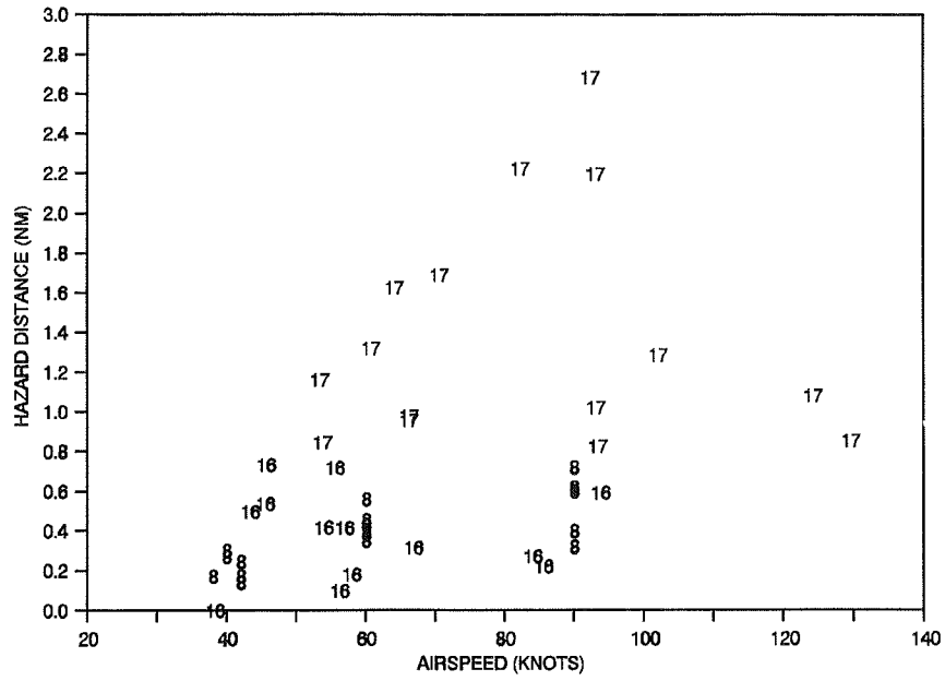
FIGURE 4-17. S-76A PREDICTED VORTEX HAZARD DISTANCE (NM) VS. AIRSPEED (KNOTS)
