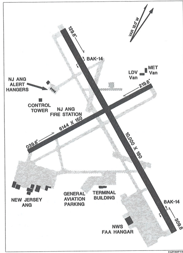
FIGURE 3-2. LDV INSTALLATION AT FAA TECHNICAL CENTER
