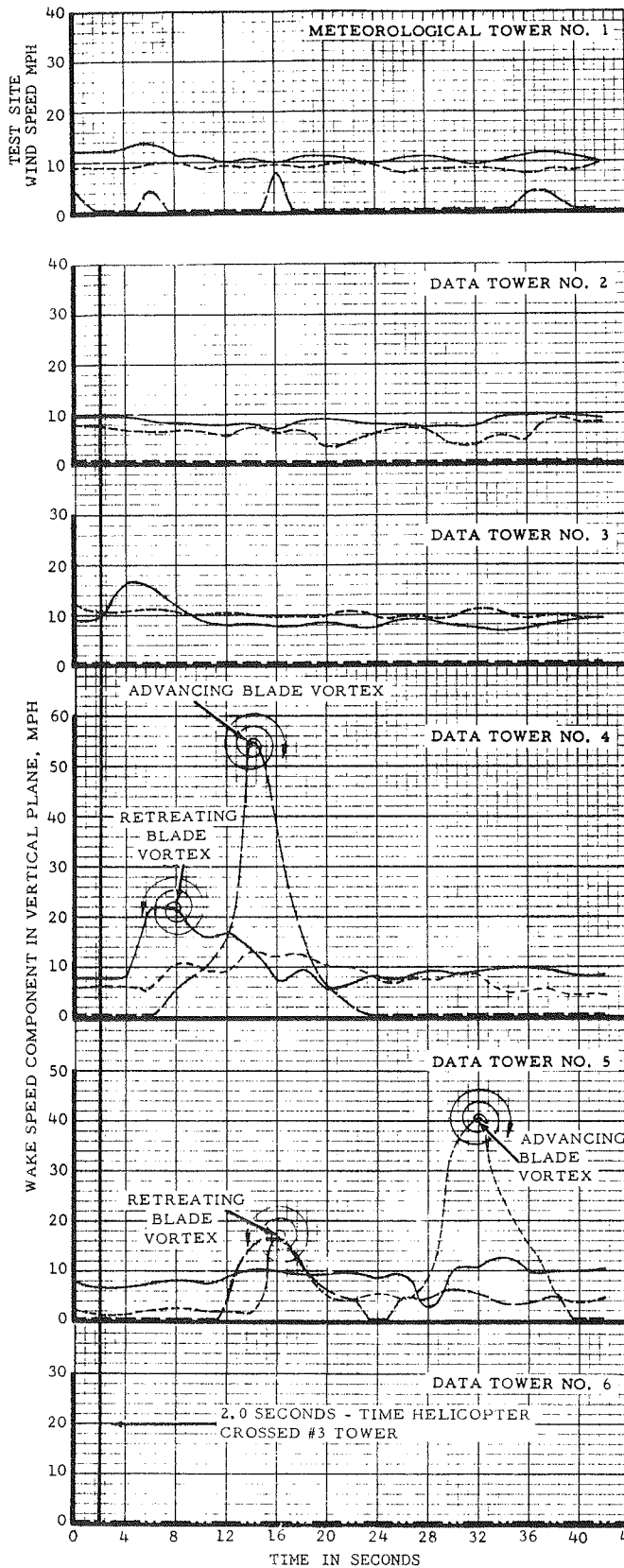
FIGURE 1-2. S-58 HELICOPTER WAKE VORTEX TIME HISTORY, CROSSWIND RUN NUMBER FOUR
