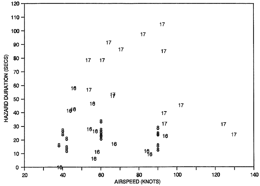
FIGURE 4-13. S-76A MODELED VORTEX HAZARD DURATION VS. AIRSPEED (KNOTS)
