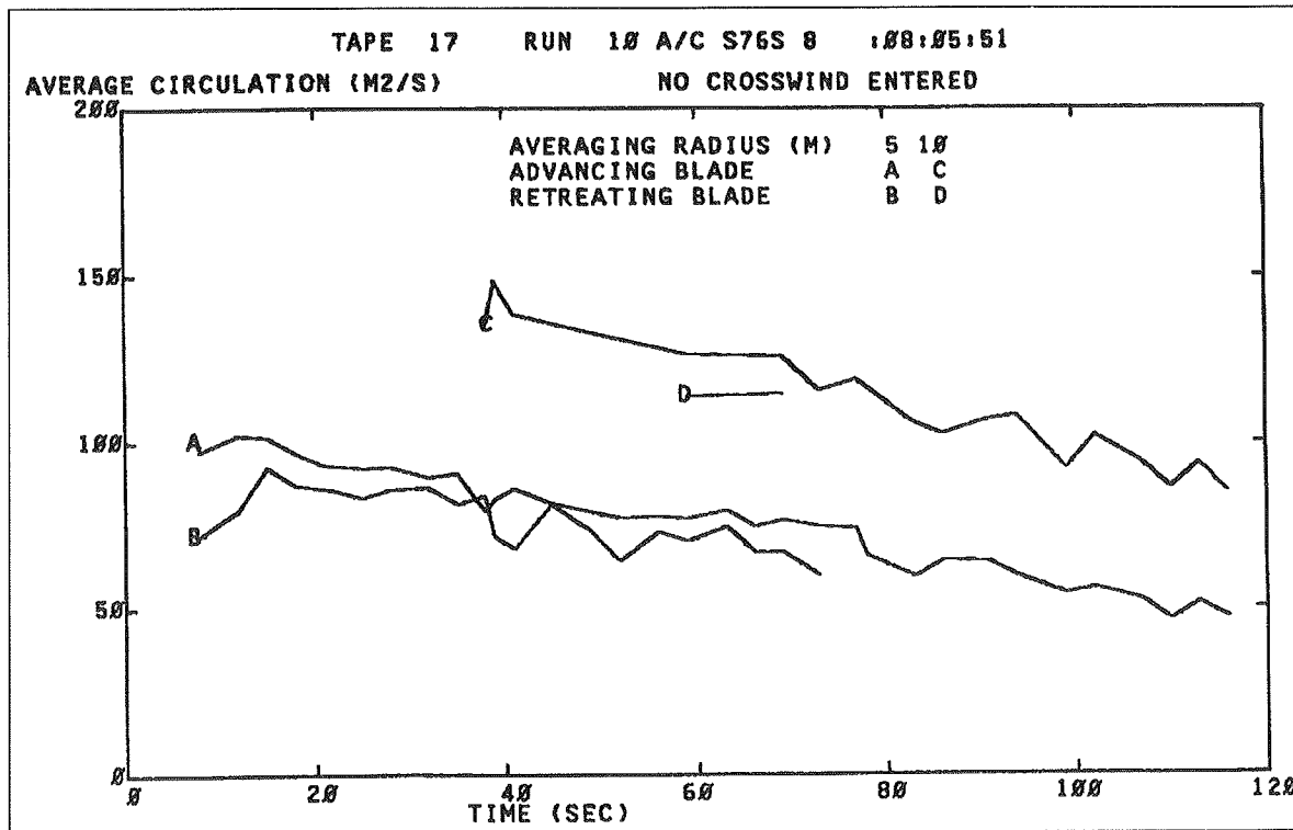
FIGURE 3-11. S-76A AVERAGE CIRCULATION VS. TIME
