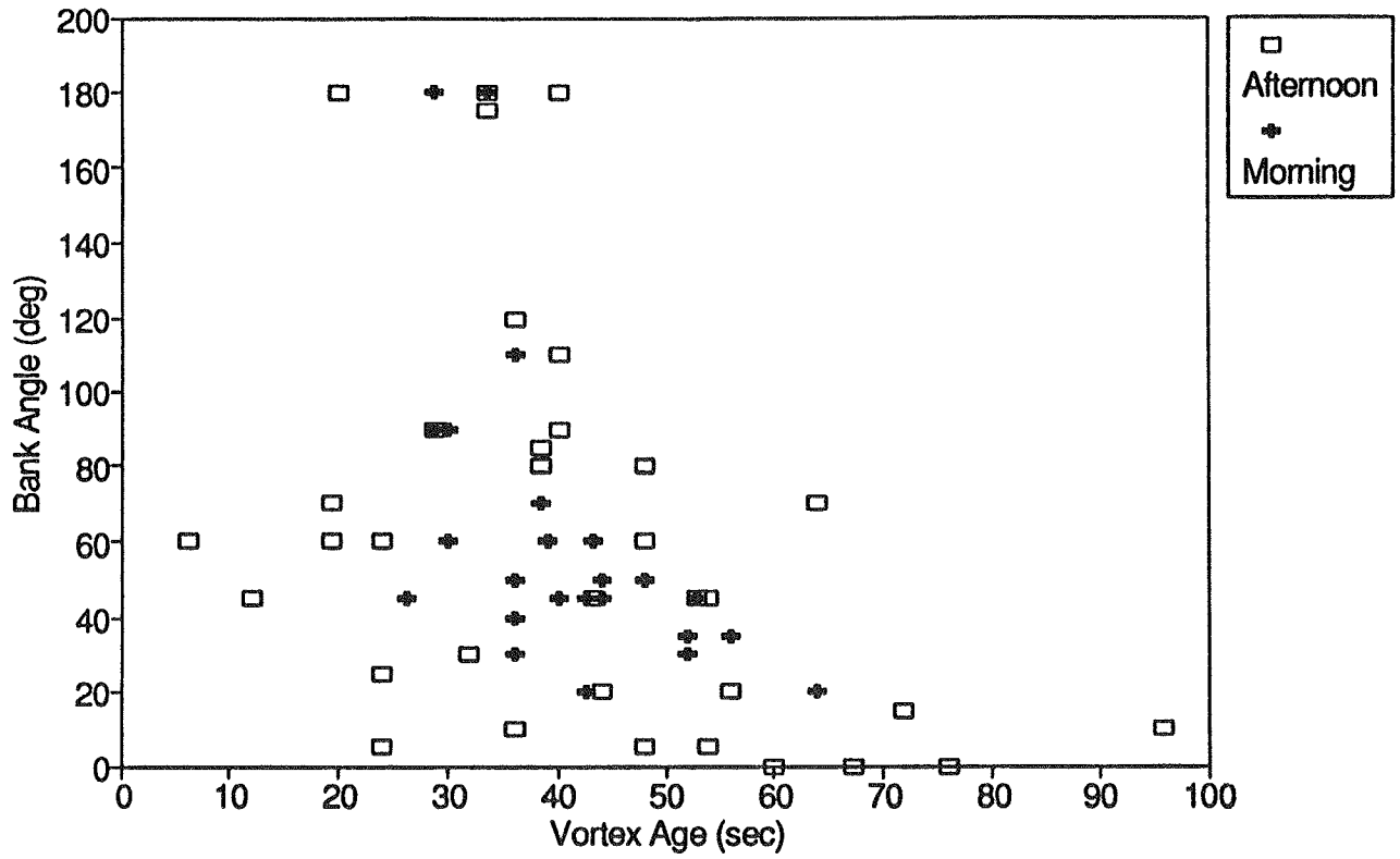
FIGURE 6-3. PROBE UPSET BANK ANGLE VS. VORTEX AGE FOR CH-47D
