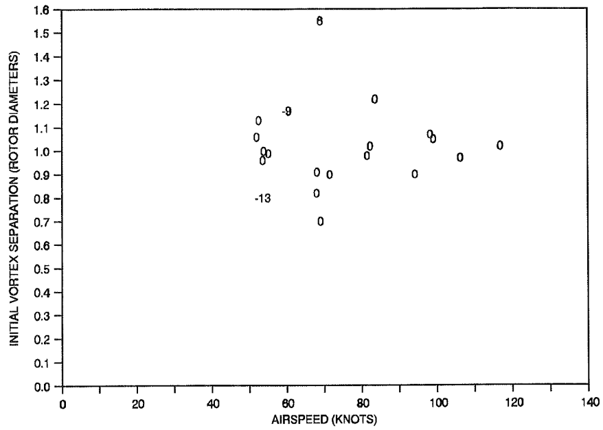
FIGURE 4-10. UH-60A VORTEX SEPARATION (ROTOR DIAMETERS) VS. AIRSPEED (KNOTS)
