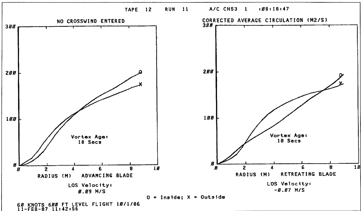
FIGURE 3-10. CH-53E CIRCULATION PROFILES
