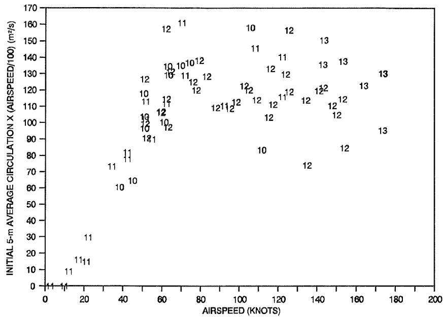
FIGURE 4-8. CH-53E 5-M INITIAL AVERAGE CIRCULATION X (V/100) VS. AIRSPEED (KNOTS)
