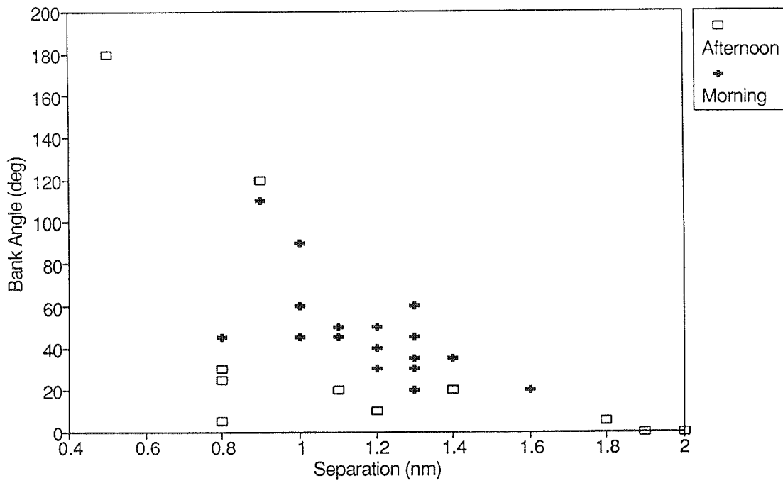
FIGURE 5-9. BANK ANGLE VS. SEPARATION FOR CH-47D (90-120 KNOTS AIRSPEED)
