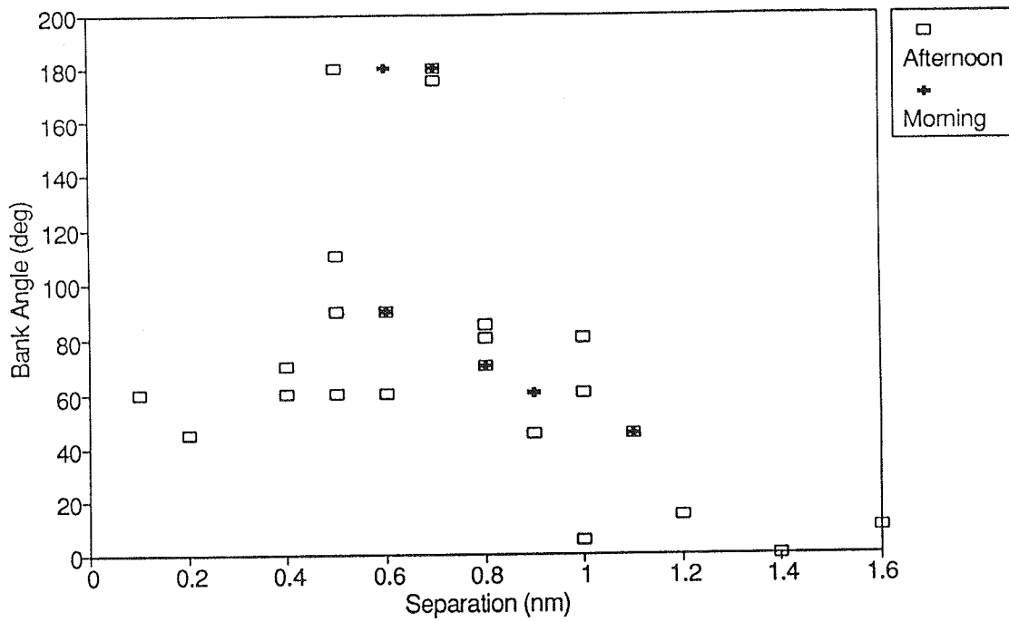
FIGURE 5-8. BANK ANGLE VS. SEPARATION FOR CH-47D (45-75 KNOTS AIRSPEED)
