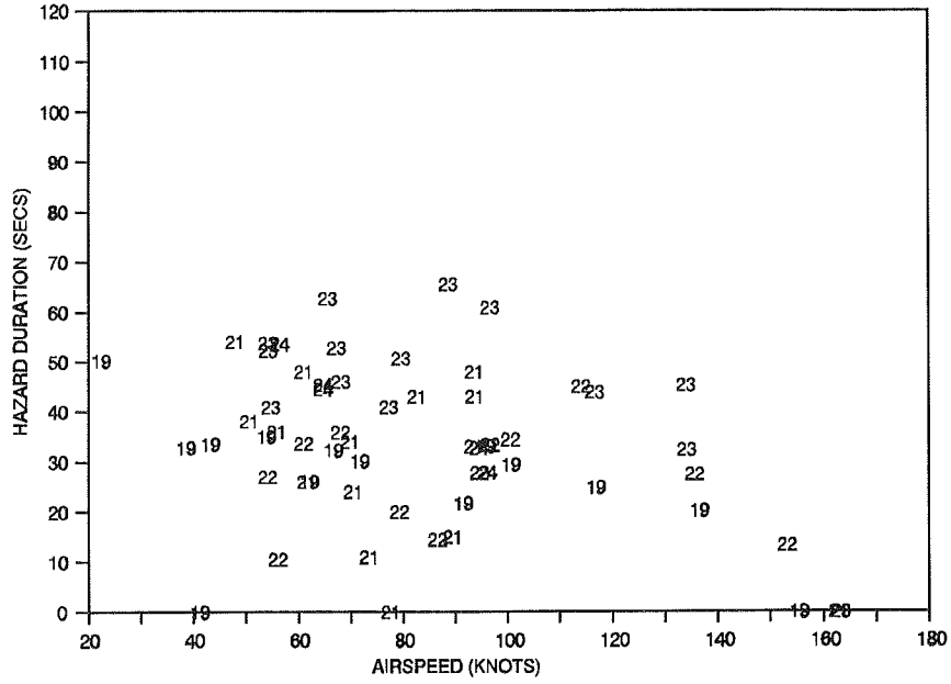
FIGURE 4-15. CH-47D MODELED VORTEX HAZARD DURATION VS. AIRSPEED (KNOTS)
