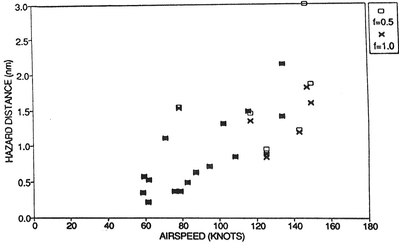
FIGURE 6-2. PREDICTED HAZARD DISTANCE VS. AIRSPEED FOR CH-53E (TAPE 12)
