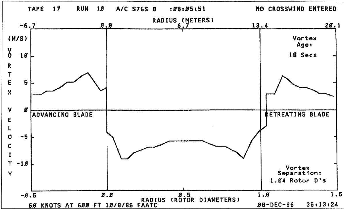
FIGURE 3-9. FULL-SIZE S-76A WAKE VELOCITY PROFILE
