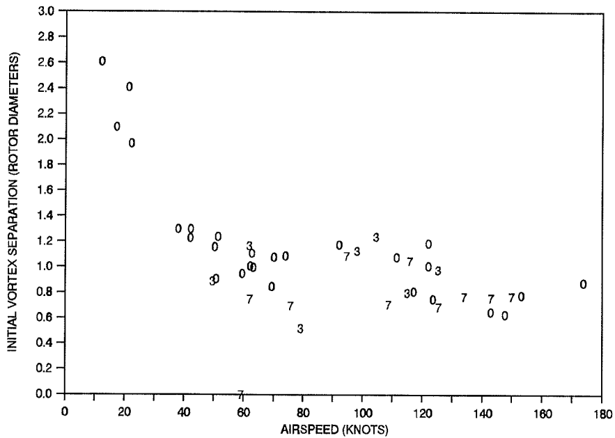
FIGURE 4-12. CH-53E VORTEX SEPARATION (ROTOR DIAMETERS) VS. AIRSPEED (KNOTS)
