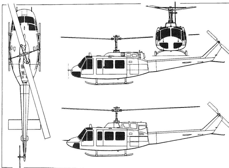
FIGURE 1-4. BELL UN-1H HELICOPTER SCHEMATIC (REFERENCE 12)
