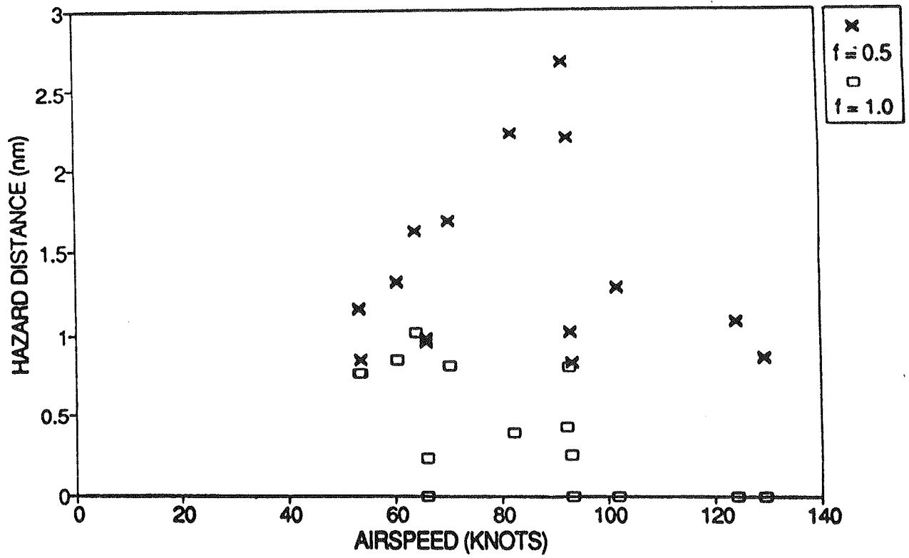
FIGURE 6-1. PREDICTED HAZARD DISTANCE VS. AIRSPEED FOR S-76A (TAPE 17)
