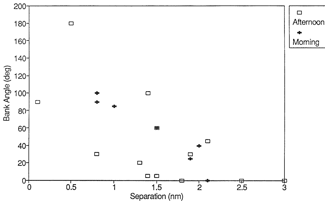
FIGURE 5-10. BANK ANGLE VS. SEPARATION FOR CH-53E (80-120 KNOTS AIRSPEED)
