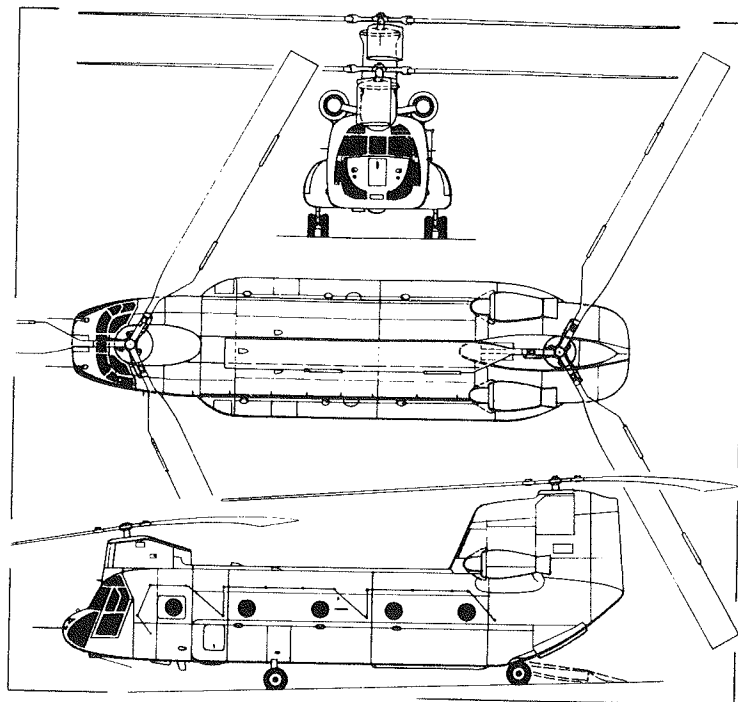
FIGURE 1-8. BOEING VERTOL CH-47D HELICOPTER SCHEMATIC (REFERENCE 12)
