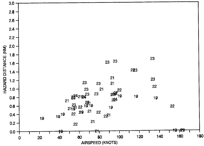
FIGURE 4-19. CH-47D PREDICTED VORTEX HAZARD DISTANCE (NM) VS. AIRSPEED (KNOTS)
