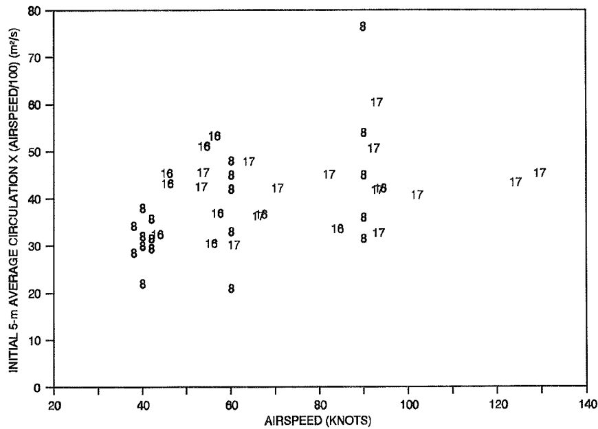
FIGURE 4-5. S-76A 5-M INITIAL AVERAGE CIRCULATION X (V/100) VS. AIRSPEED (KNOTS)
