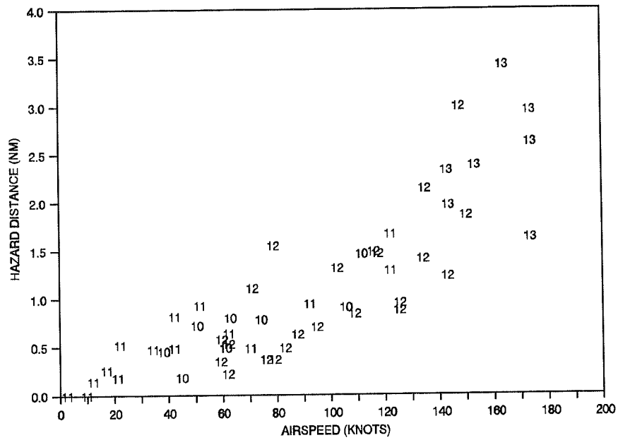
FIGURE 4-20. CH-53E PREDICTED VORTEX HAZARD DISTANCE (NM) VS. AIRSPEED (KNOTS)
