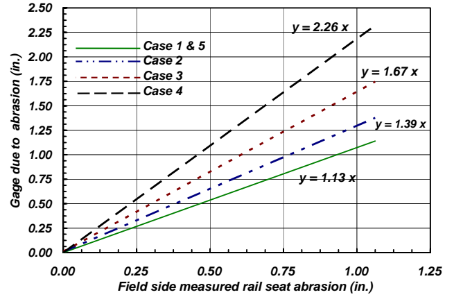
Figure 9. Recommended charts to calculate loaded gage at location with concrete tie rail seat abrasion.
