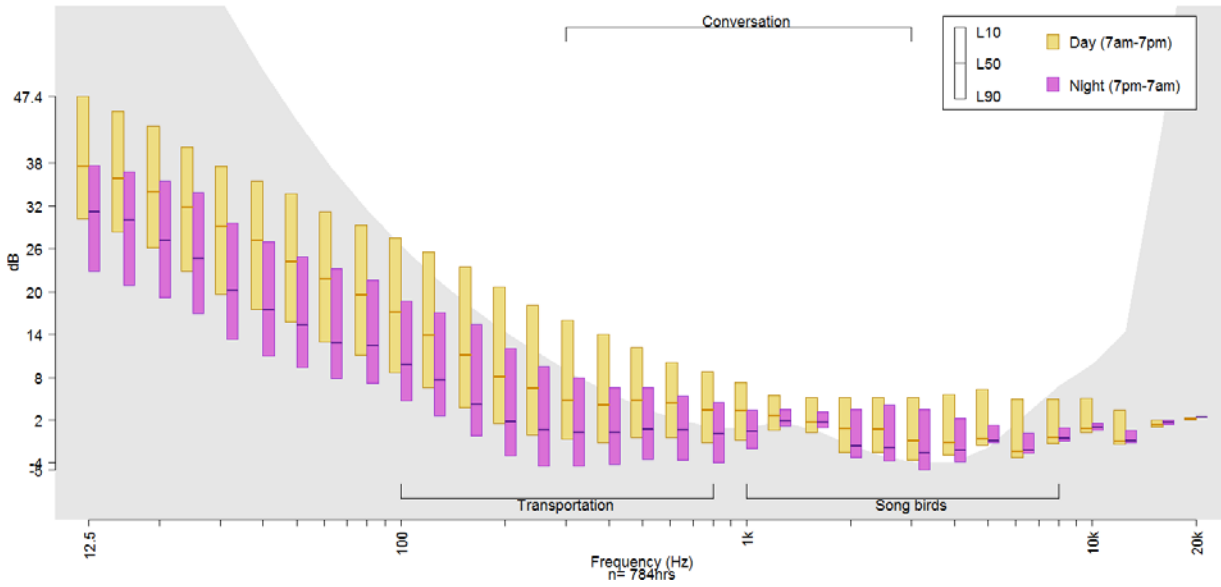
Figure 15. Sound spectrum for WUPA001
