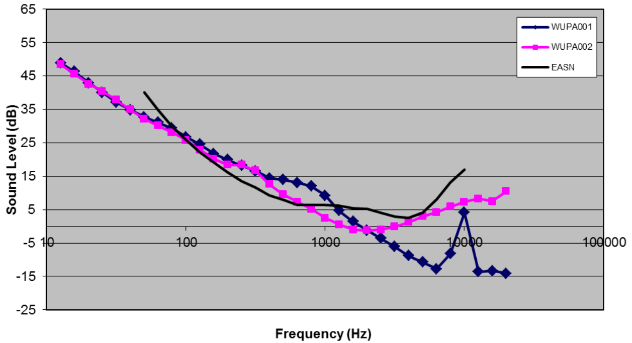
Figure 3. Spectral data for the Existing Ambient Without Air Tours ( L_{50} ) for each site*
