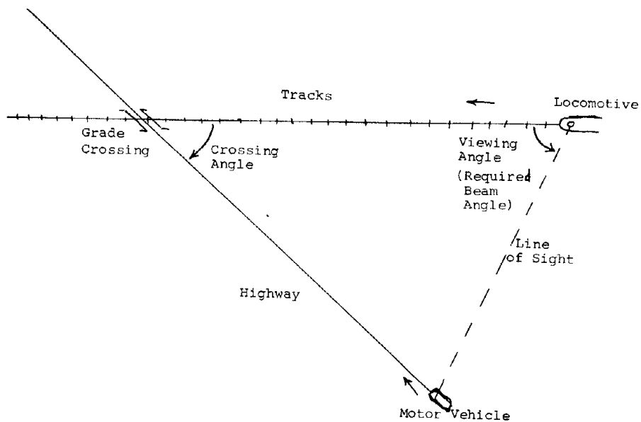
Figure 9. a. Required Beam Angle as a Function of Crossing Angle, for Various Ratios of Vehicle Speed to Train Speed b. Geometry of a
