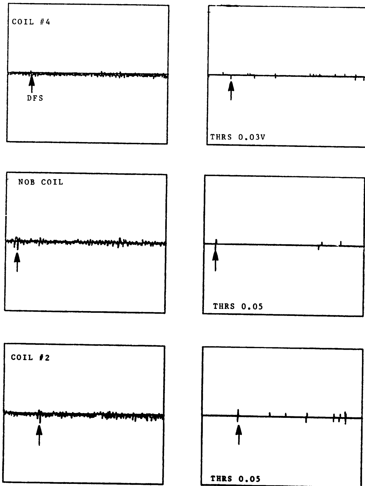
FIGURE 22. AMPLITUDE-TIME HISTORIES OF ANALOG AND DIFFERENTIATED-THRESHOLDED SIGNALS FOR SECTION OF RAIL CONTAINING A DETAIL FRACTURE
