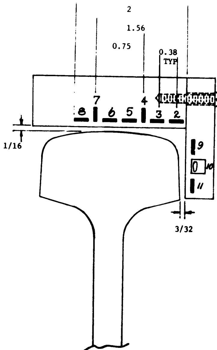
FIGURE 13. LAYOUT OF HALL ELEMENT SENSORS
