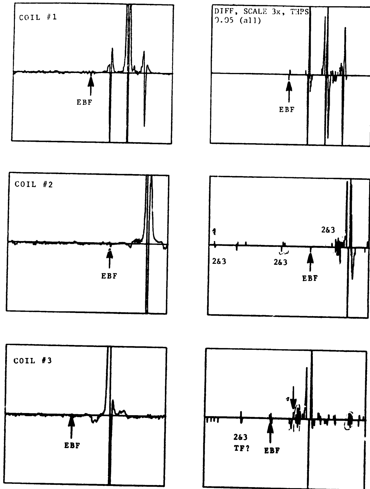
FIGURE 23. AMPLITUDE-TIME HISTORIES OF ANALOG AND DIFFERENTIATED-THRESHOLDED SIGNALS FOR RAIL SECTION CONTAINING AN ENGINE BURN FRACTURE
