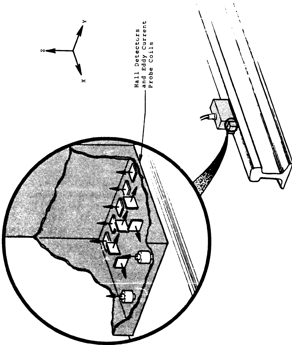
FIGURE 5. SENSOR CONFIGURATION TO BE USED IN INITIAL EXPERIMENTS
