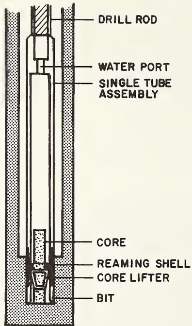
FIGURE 7-27. SINGLE TUBE CORE BARREL
