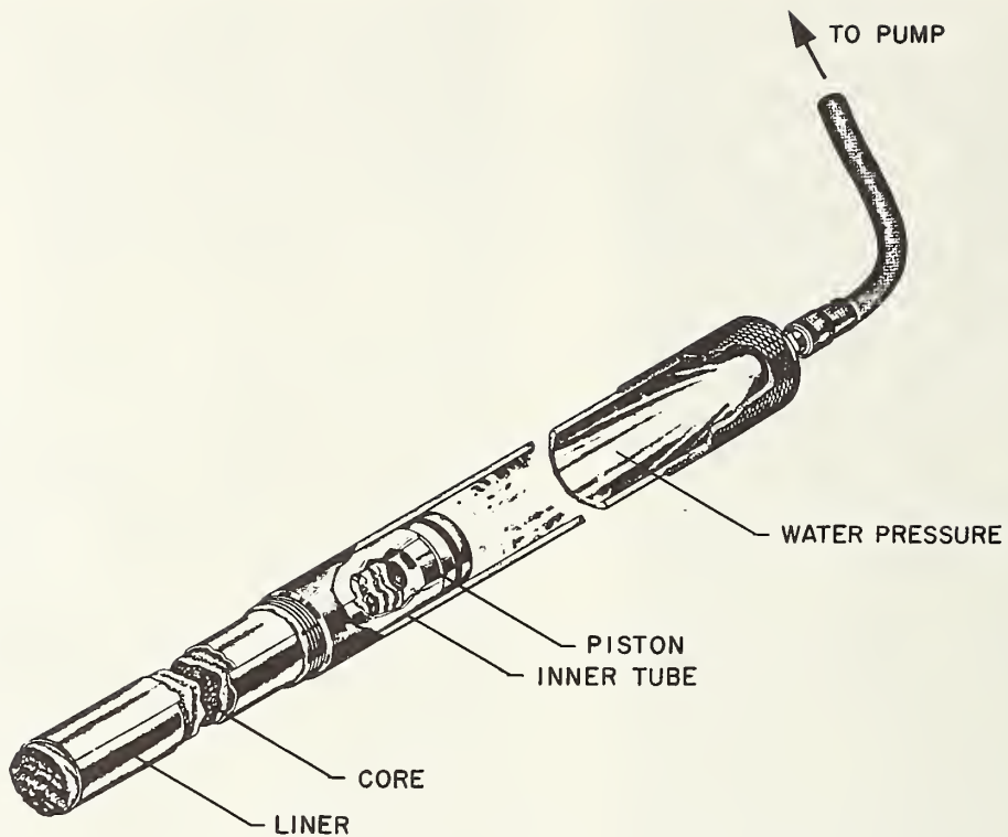
FIGURE 7-41. HYDRAULIC REMOVAL OF SPLIT-INNER LINER FROM HXWL CORE BARREL
