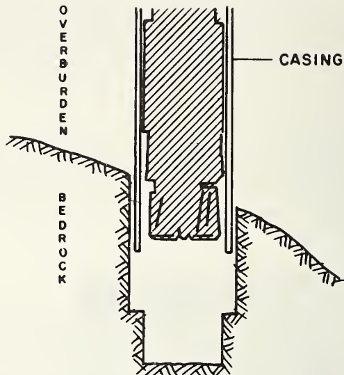
FIGURE 7-11. ODEX BIT WITHDRAWN WITH ECCENTRIC REAMER RETRACTED
