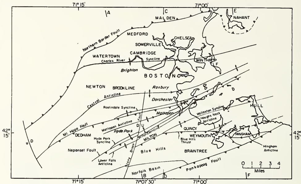
FIGURE 5-1. TECTONIC MAP OF BOSTON BASIN BILLINGS (19-2)
