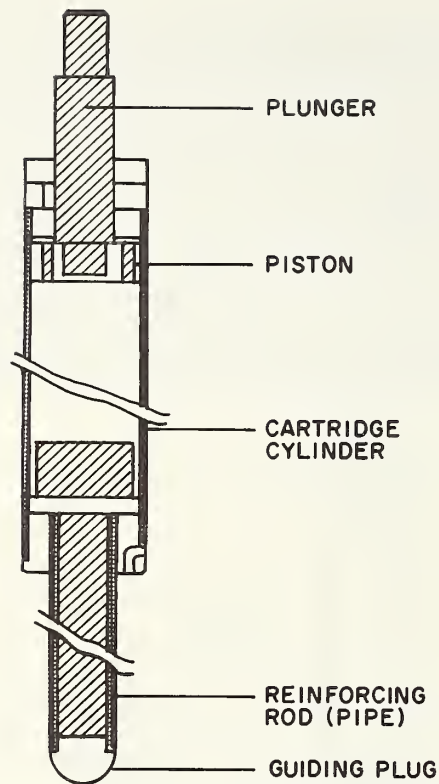
FIGURE 7-38. CSIR RESIN CARTRIDGE AND REINFORCING PIPE ASSEMBLY
