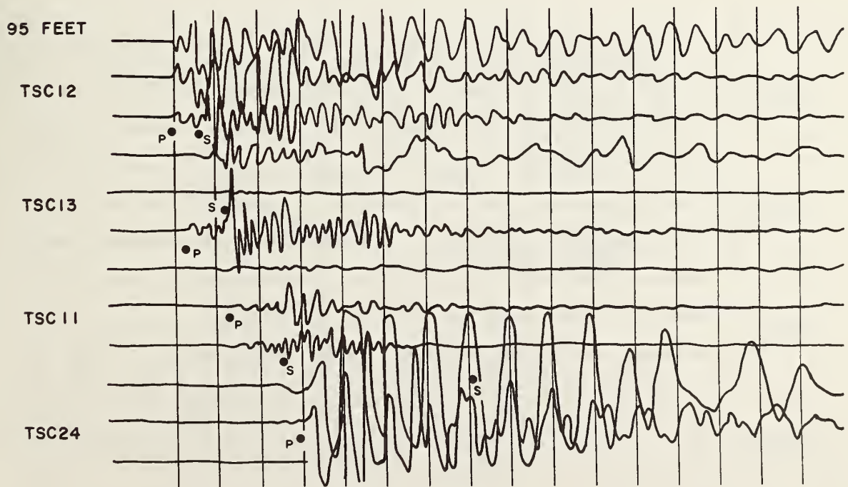
TYPICAL WAVEFORMS.
