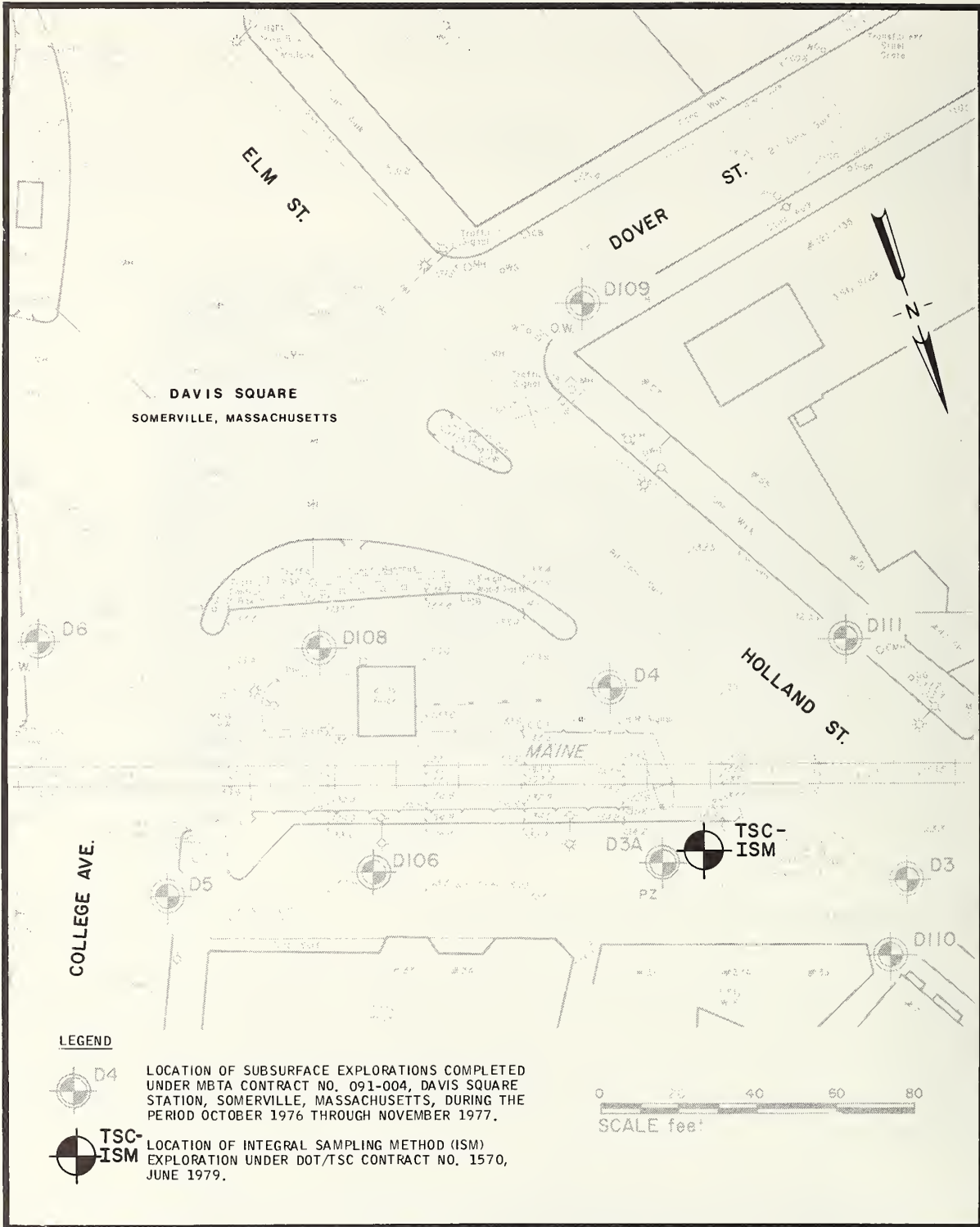
FIGURE 6-4. SUBSURFACE EXPLORATION PLAN, DAVIS SQUARE SITE, SOMERVILLE, MASSACHUSETTS
