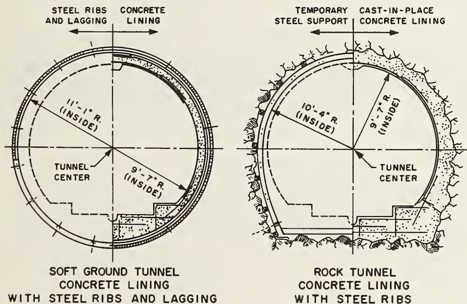
FIGURE 4-2. TYPICAL RED LINE TUNNEL SECTIONS
