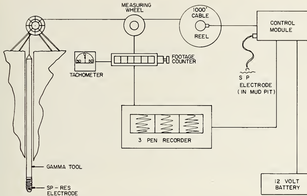
FIGURE 7-56. SCHEMATIC OF ELECTRIC BOREHOLE LOGGER
