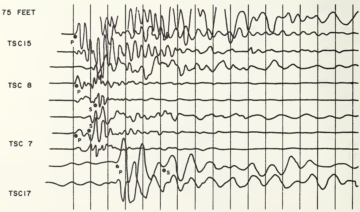
WAVE FORMS WITHOUT REFRACTION INTERFACE. GEOPHONES ROTATED IN LOWER TRACE.
