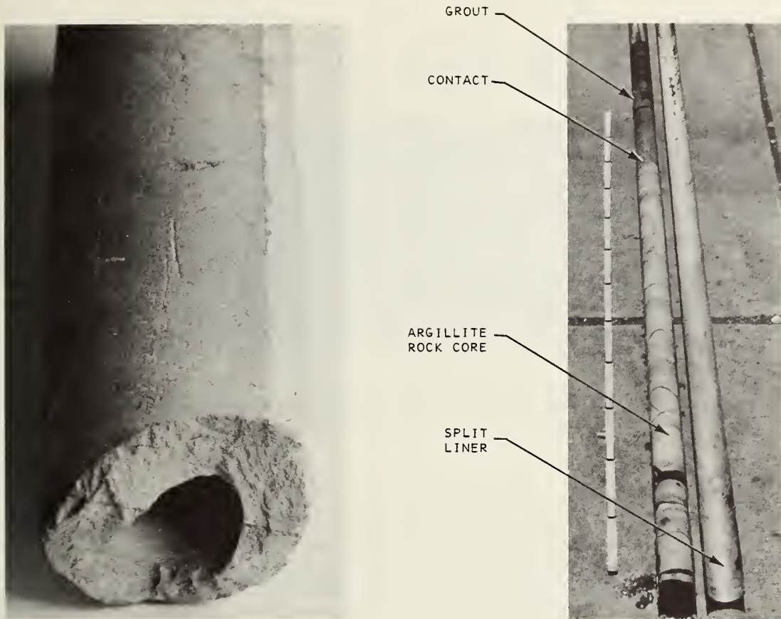
FIGURE 7-48. ISM ROCK CORE
