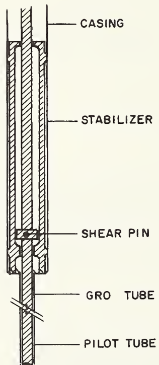
FIGURE 7-36. ISM PHASE II, GRO TUBE AND STABILIZING ASSEMBLY
