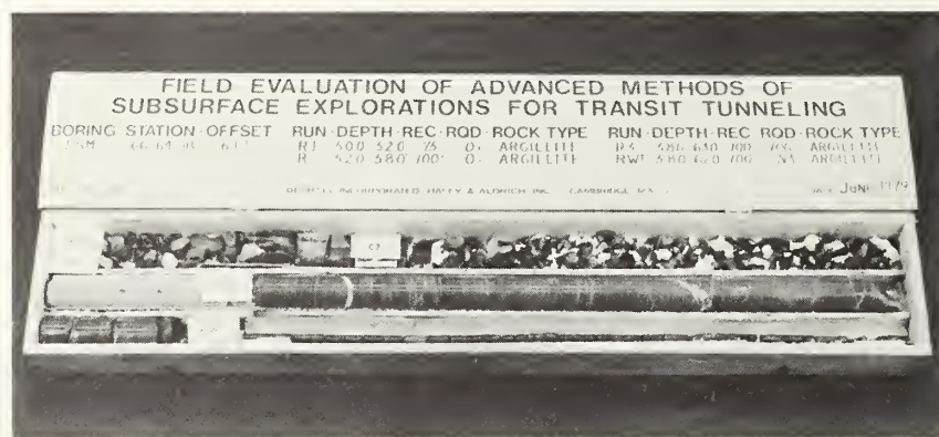
FIGURE 7-44. DAVIS SQUARE ISM ROCK CORE
