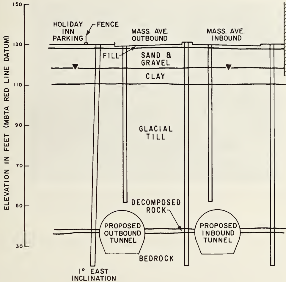
FIGURE 6-2. TYPICAL HIGH-INTENSITY EXPLORATION INSTRUMENTATION PROFILE
