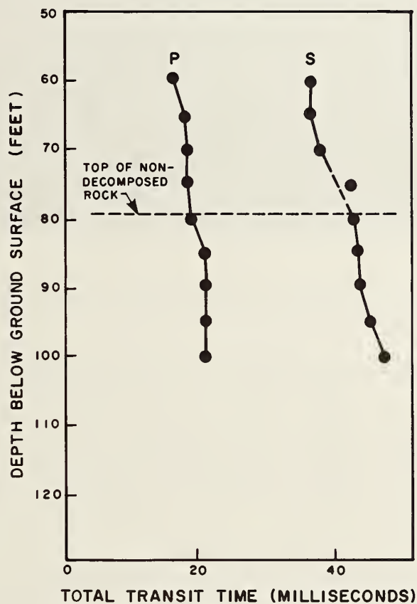
FIGURE 9-1. SEISMIC UPHOLE DATA, BORING TSC 17, SERIES 4A
