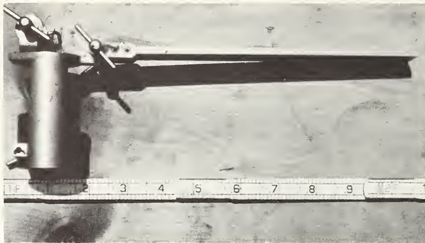
FIGURE 7-35. ISM ORIENTING SIGHT ASSEMBLY
