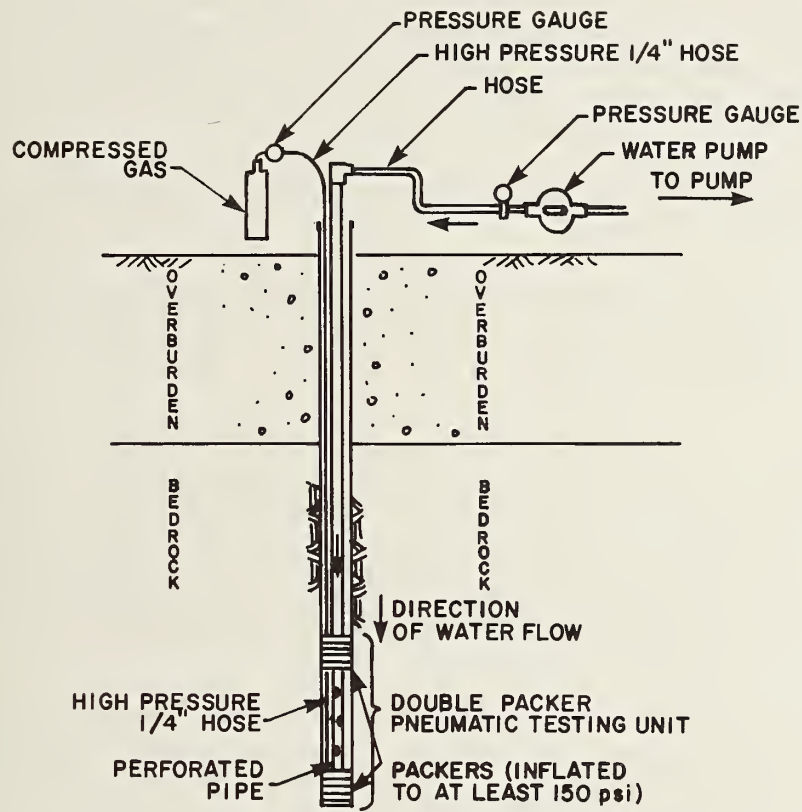
FIGURE 7-65. SCHEMATIC DIAGRAM OF WATER PRESSURE TEST ASSEMBLY
