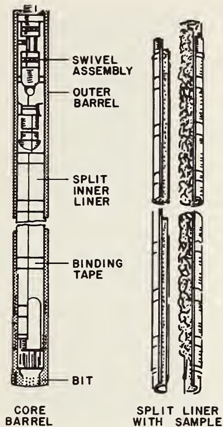
FIGURE 7-31. NWD3 TM SPLIT-INNER LINER CORE BARREL
