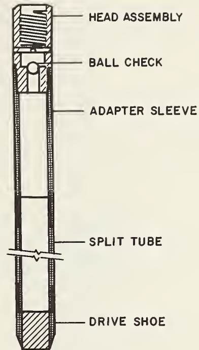
FIGURE 7-19. STANDARD SPLIT-SPOON SAMPLER
