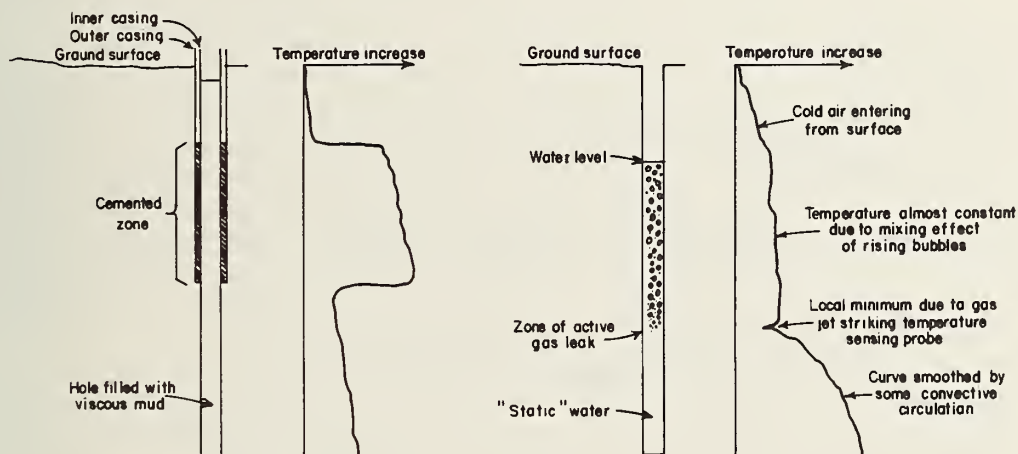
FIGURE 8-2. SCHEMATICS OF TEMPERATURE LOGS DAVIS (11-6)
