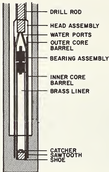
FIGURE 7-22. DENISON TM CORE BARREL
