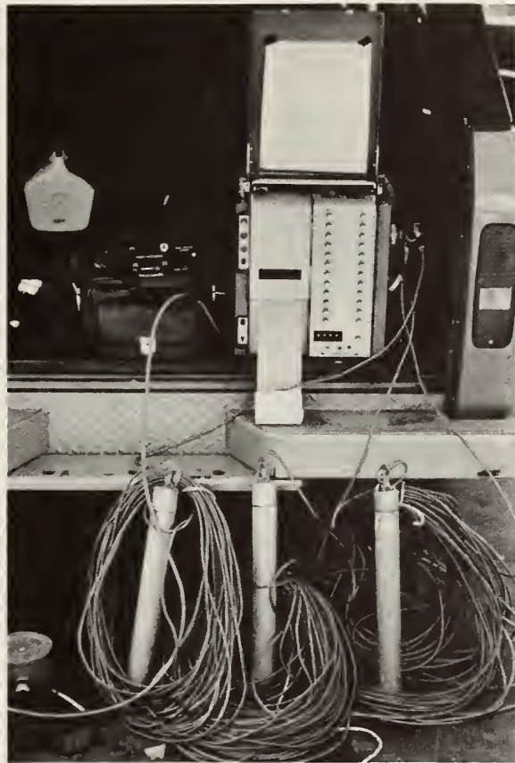
FIGURE 7-58. SIGNAL ENHANCEMENT SEISMIC UNIT WITH BOREHOLE GEOPHONES
