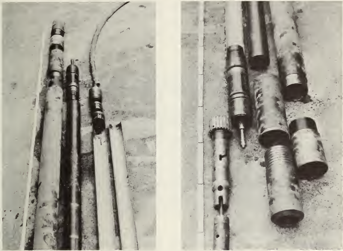
FIGURE 7-40. SPRAGUE & HENWOOD HXWL TM TRIPLE TUBE SPLIT-INNER LINER CORE BARREL
