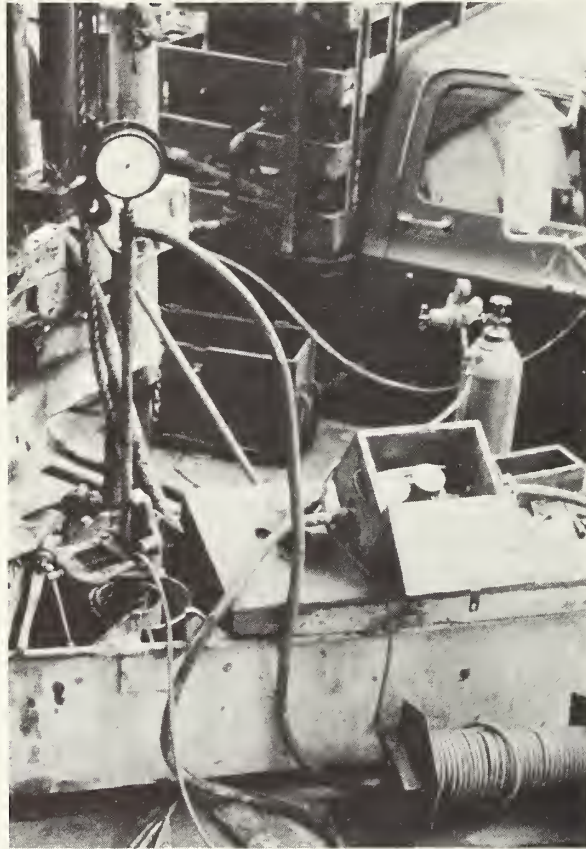
FIGURE 7-64. WATER PRESSURE TEST SURFACE EQUIPMENT
