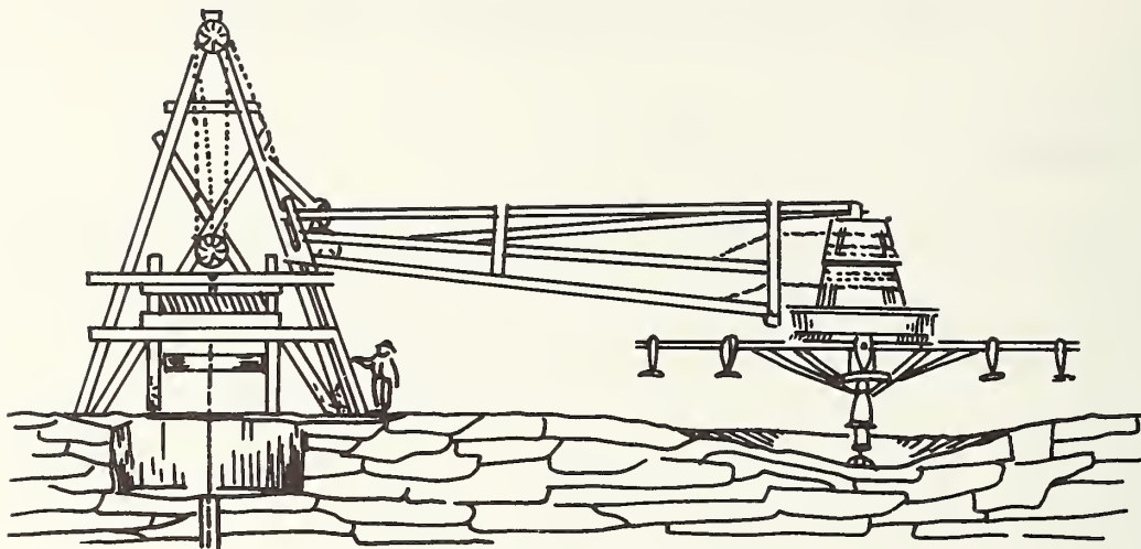
FIGURE 7-1. GRENELLE DRILL RIG, 16TH CENTURY GASS (8-14)
