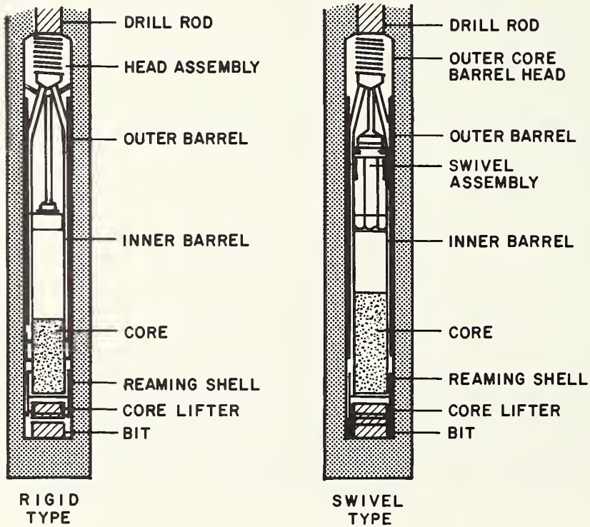
FIGURE 7-28. DOUBLE TUBE CORE BARRELS
