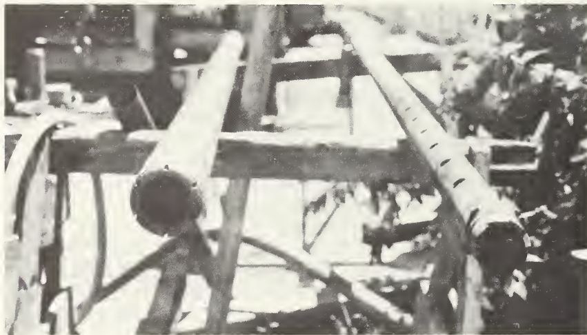
FIGURE 7-42. ISM CORE BARRELS: HXWL OVERCORE BARREL (LT.) AND RWT PILOT CORE BARREL WITH STABILIZING ASSEMBLY (RT.)
