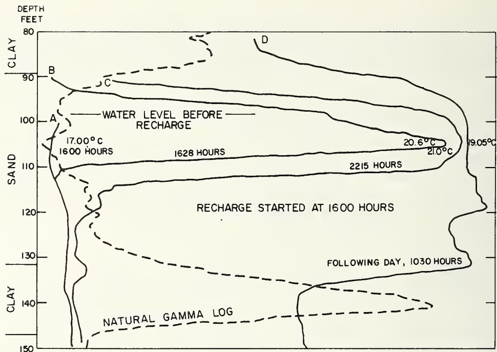
FIGURE 8-3. TEMPERATURE LOGGING DURING ARTIFICIAL RECHARGE KEYS (1-15)
