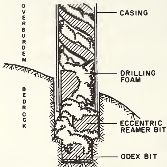
FIGURE 7-10. ODEX TM BIT ADVANCING WITH ECCENTRIC REAMER EXTENDED AND CASING FOLLOWING
