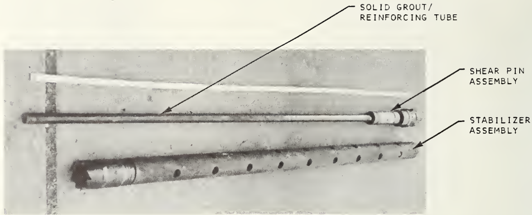
FIGURE 7-49. GRO STABILIZING ASSEMBLY WITH SOLID GROUT/REINFORCING TUBE
