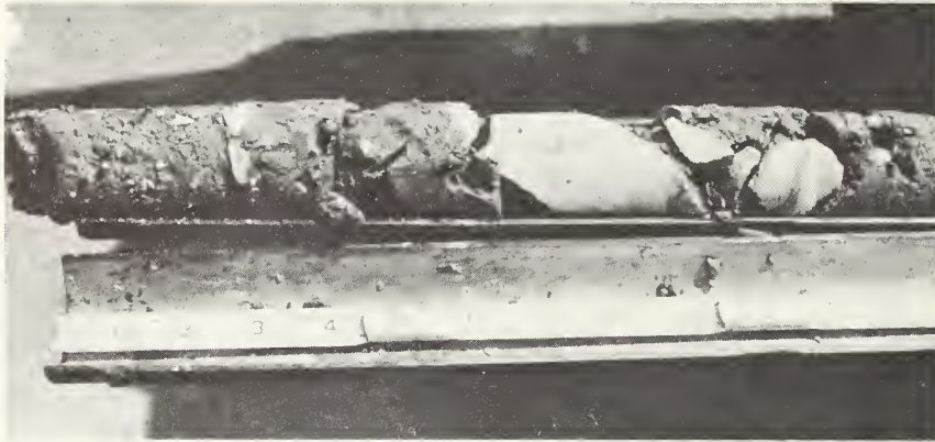
FIGURE 7-29. GLACIAL TILL RECOVERED WITH NWD3 TM SPLIT INNER LINER CORE BARREL
