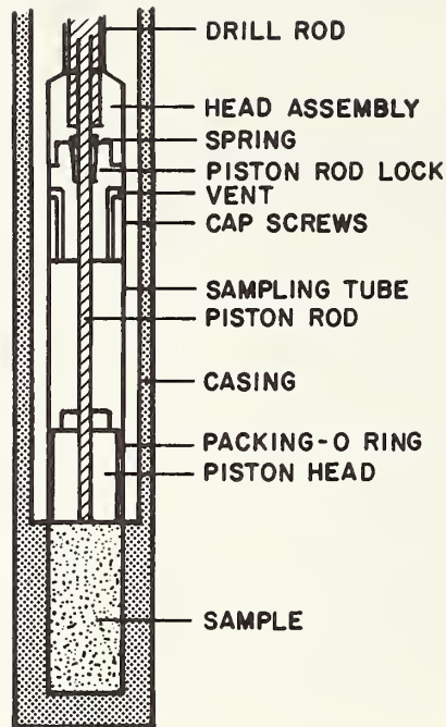
FIGURE 7-18. STATIONARY PISTON SAMPLER
