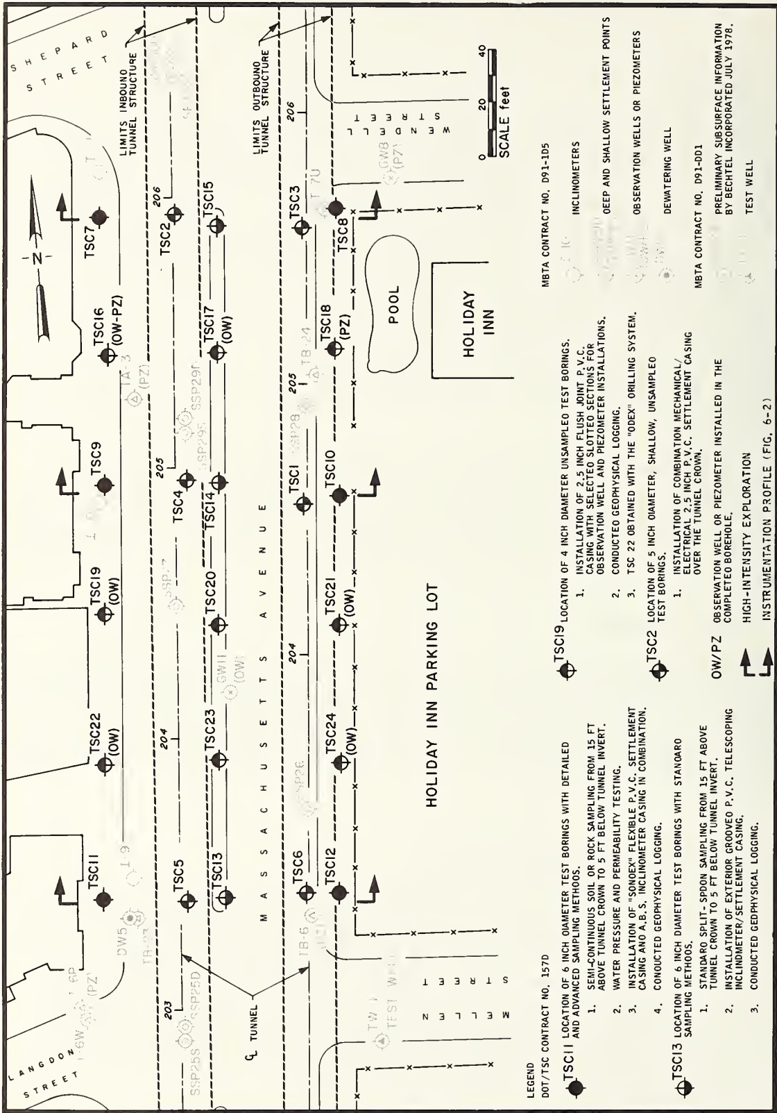
FIGURE 6-1. SUBSURFACE EXPLORATION PLAN, HOLIDAY INN SITE, CAMBRIDGE, MASSACHUSETTS
