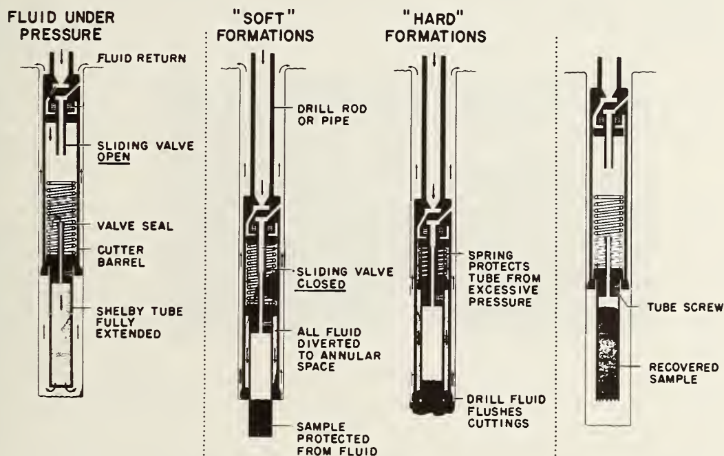
FIGURE 7-25. PITCHER TM SAMPER OPERATION
