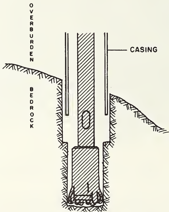
FIGURE 7-12. CONVENTIONAL ROCK DRILLING IN ODEX BOREHOLE
