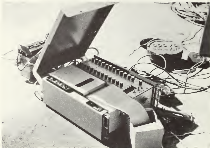
FIGURE 7-59. GEOMETRICS/NIMBUS INSTRUMENTS MODEL 1200™ MULTIPLE CHANNEL SIGNAL ENHANCEMENT SEISMOGRAPH
