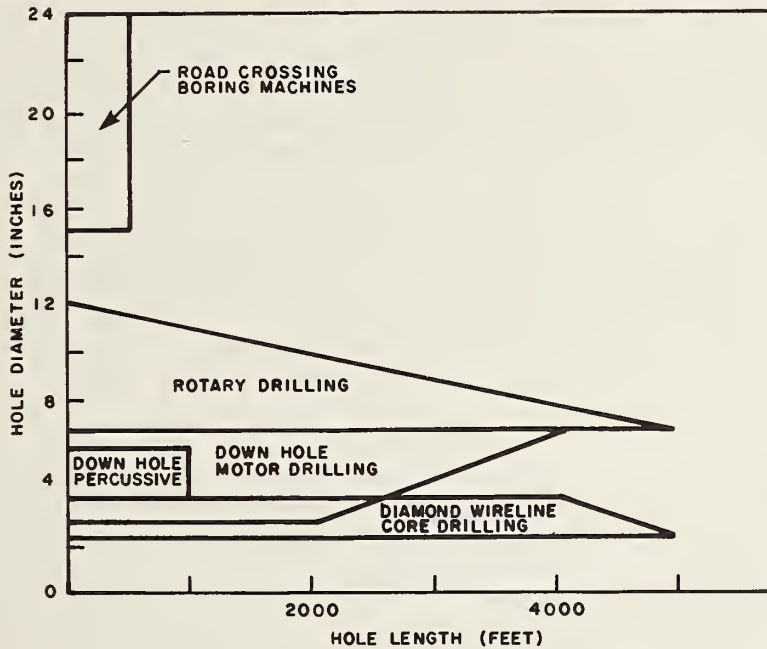
FIGURE 8-1. TYPICAL HORIZONTAL PENETRATION CAPABILITY HARDING (10-18)
