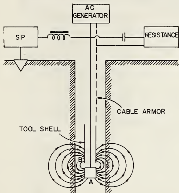
FIGURE 7-54. SCHEMATIC DIAGRAM OF SINGLE POINT RESISTIVITY LOGGING TECHNIQUE
