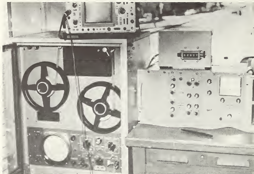
FIGURE 7-52. DIGITAL RECORDING COMPUTER AND NUCLEAR LOGGING CONTROL PANEL
