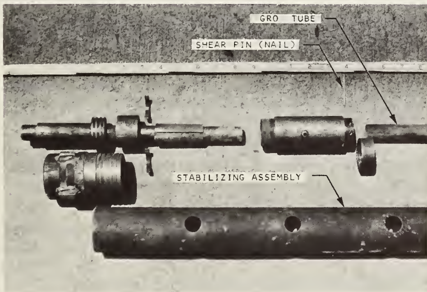
FIGURE 7-46. DISASSEMBLED GRO TUBE SHOWING CONNECTION OF GRO TUBE TO ORIENTING RODS WITH SHEAR PIN
