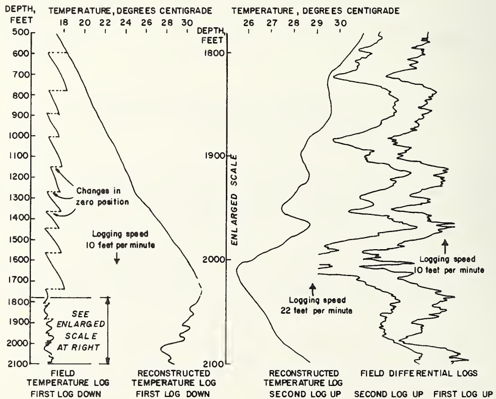
FIGURE 8-4. TYPICAL FIELD AND RECONSTRUCTED TEMPERATURE LOGS KEYS (1-15)
