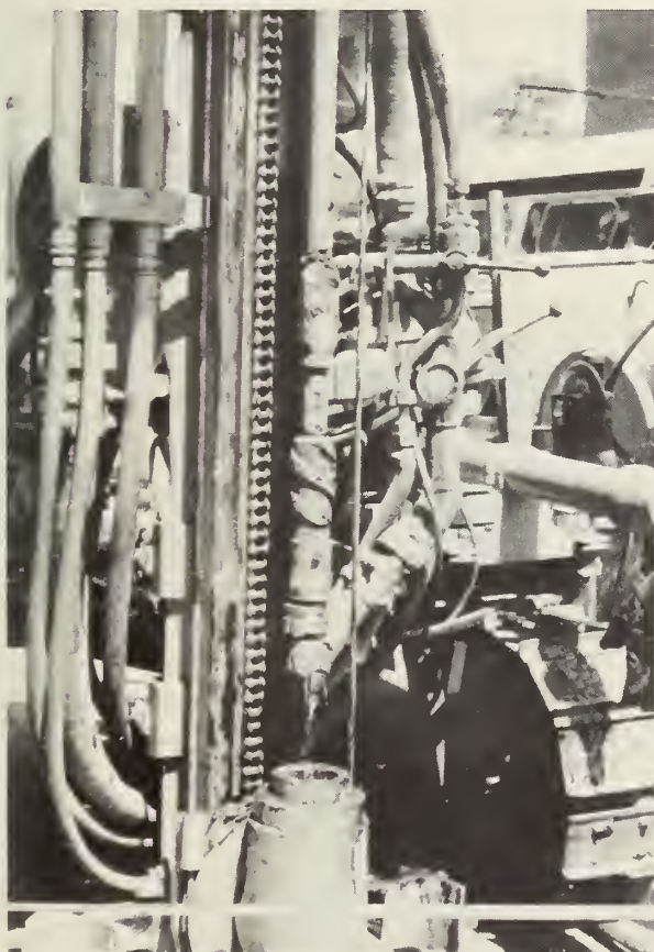
FIGURE 7-9. ODEX 76 TM BIT WITH EXTENDED REAMER
