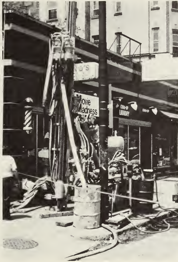
FIGURE 7-14. CHICAGO PNEUMATIC G900™ EQUIPPED WITH ATLAS COPCO™ DOUBLE ACTING HAMMER
