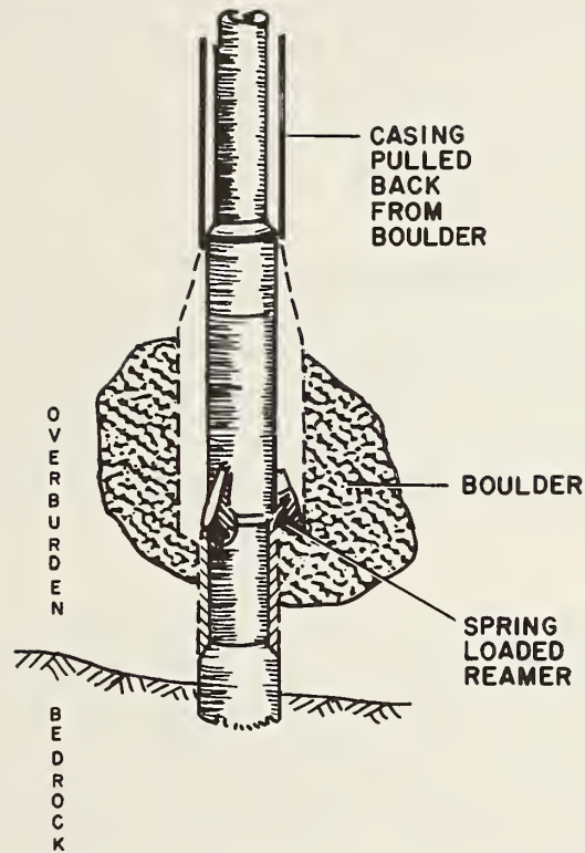
FIGURE 7-2. SERVO TM MODEL 58WCB UNDERREAMER
