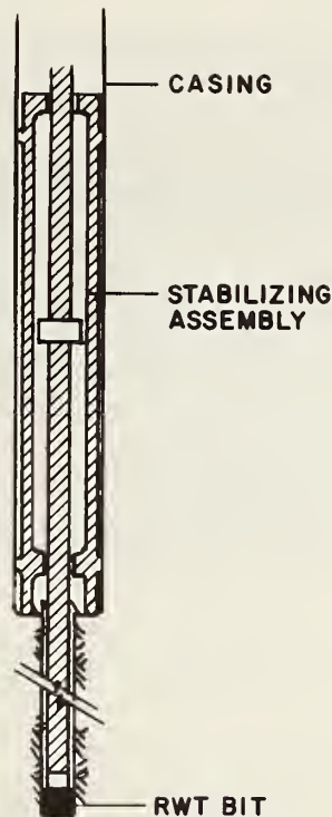
FIGURE 7-34. ISM PHASE I, RWT PILOT HOLE DRILLING AND STABILIZING ASSEMBLY
