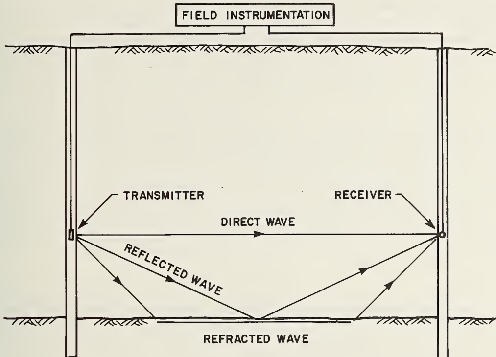
FIGURE 8-6. INTER-BOREHOLE ACOUSTIC VELOCITY LOGGING
