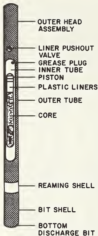
FIGURE 7-33. TRIPLE TUBE CORE BARREL WITH SOLID CLEAR PLASTIC LINER
