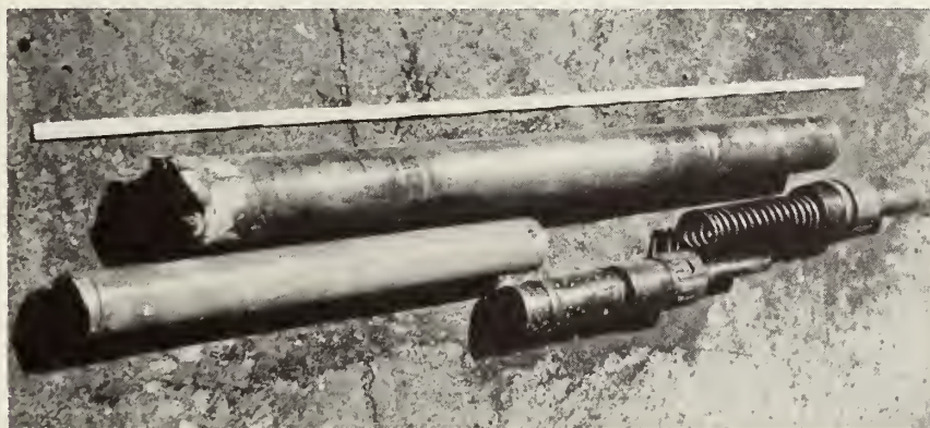
FIGURE 7-23. DISASSEMBLED PITCHER TM SAMPLER
