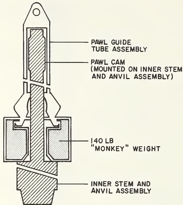
FIGURE 7-20. AUTOMATIC FREE-FALLING TRIP WEIGHT
