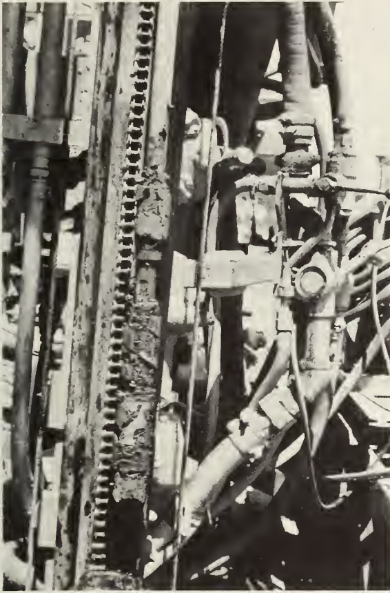
FIGURE 7-16. ODEX™ BIT PLUGGED BY THE MARINE CLAY
