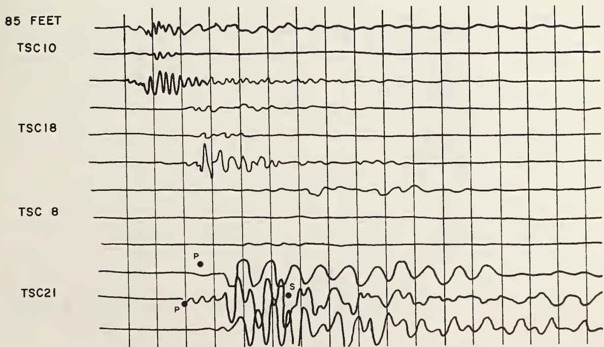
GAIN-RANGING CAPABILITY OF RECORDING SYSTEM SHOWN IN UPPER HALF OF EACH RECORD.
