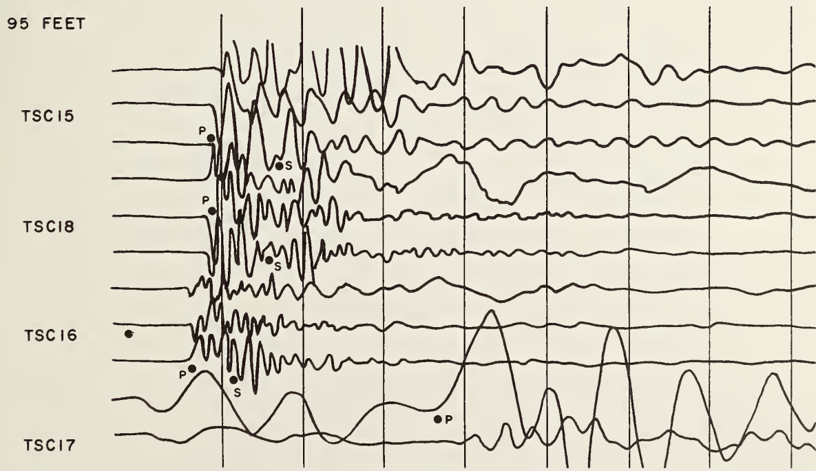
EXPANDED PLAYOUT IN LOWER HALF. NOTE GROUND ROLL AT TSC17 CAUSED BY PASSING VEHICLES.
