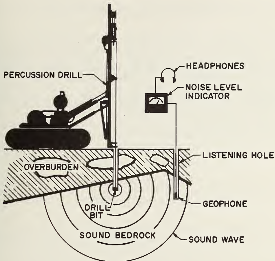
FIGURE 8-7. COMPONENTS USED FOR ACOUSTIC SOUNDING TECHNIQUE LUNDSTROM (5-24)
