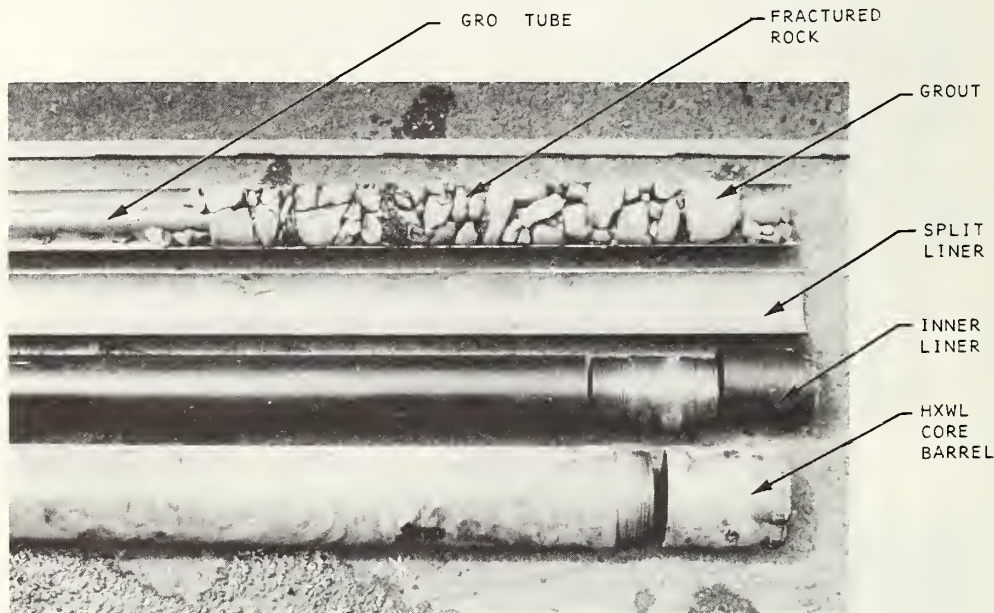
FIGURE 7-47. ISM CORE RECOVERED WITH HXWL OVERCORE BARREL WITHOUT PROPER GROUT INJECTION
