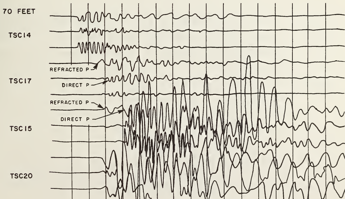
REFRACTED COMPRESSIONAL WAVES FROM UNDERLYING HIGH VELOCITY MATERIALS.
