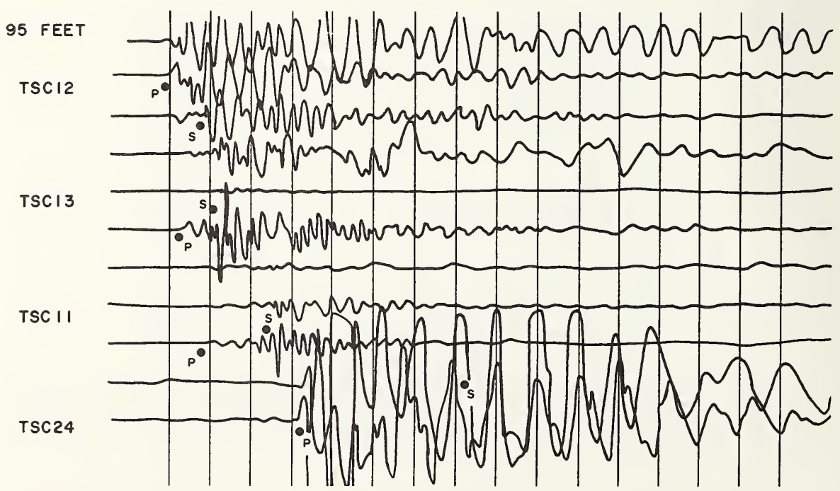
TYPICAL WAVEFORMS AFTER ROTATION.
