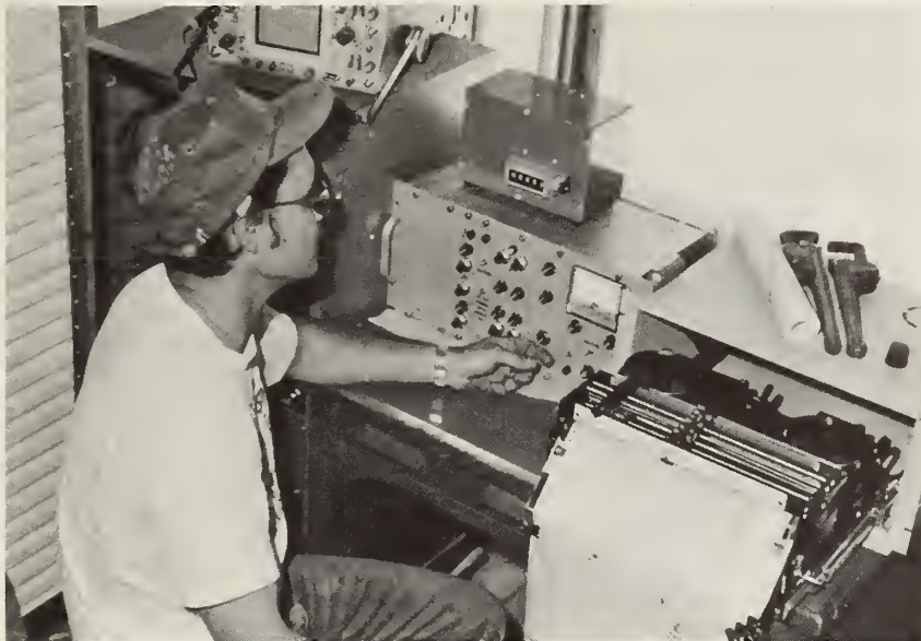
FIGURE 7-50. NUCLEAR LOGGING CONTROL PANEL, COMPUTER AND GRAPH RECORDER
