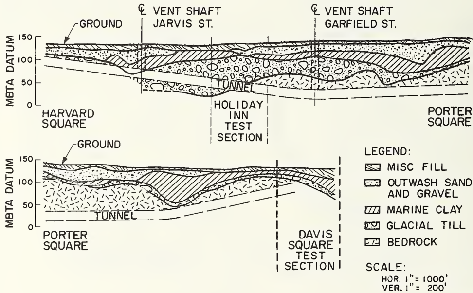
FIGURE 4-3. GENERALIZED SUBSURFACE PROFILE, HARVARD SQUARE TO DAVIS SQUARE
