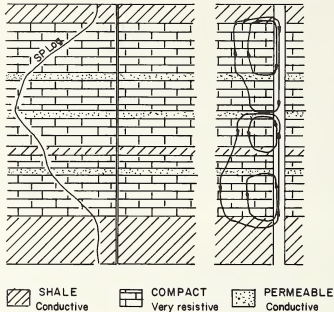
FIGURE 7-53. ELECTRICAL LOGGING EFFECTS IN VARIABLE FORMATIONS
