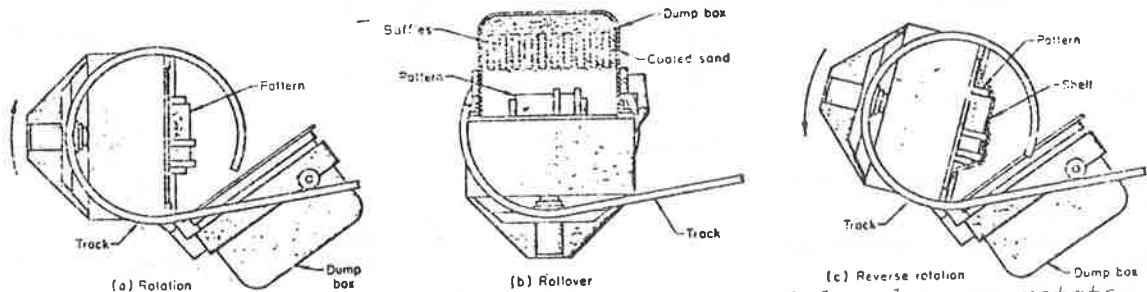
Variation A: Dump-box method in which pattern and dump box are rotated at high speed on a circular track
