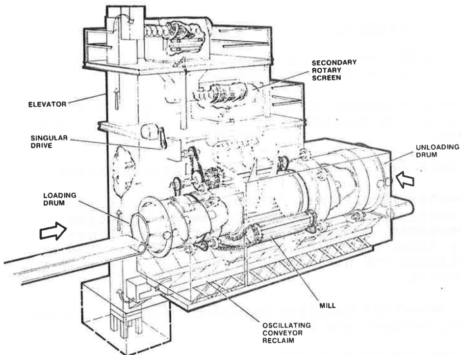
FIGURE 13 Blasting Machine
