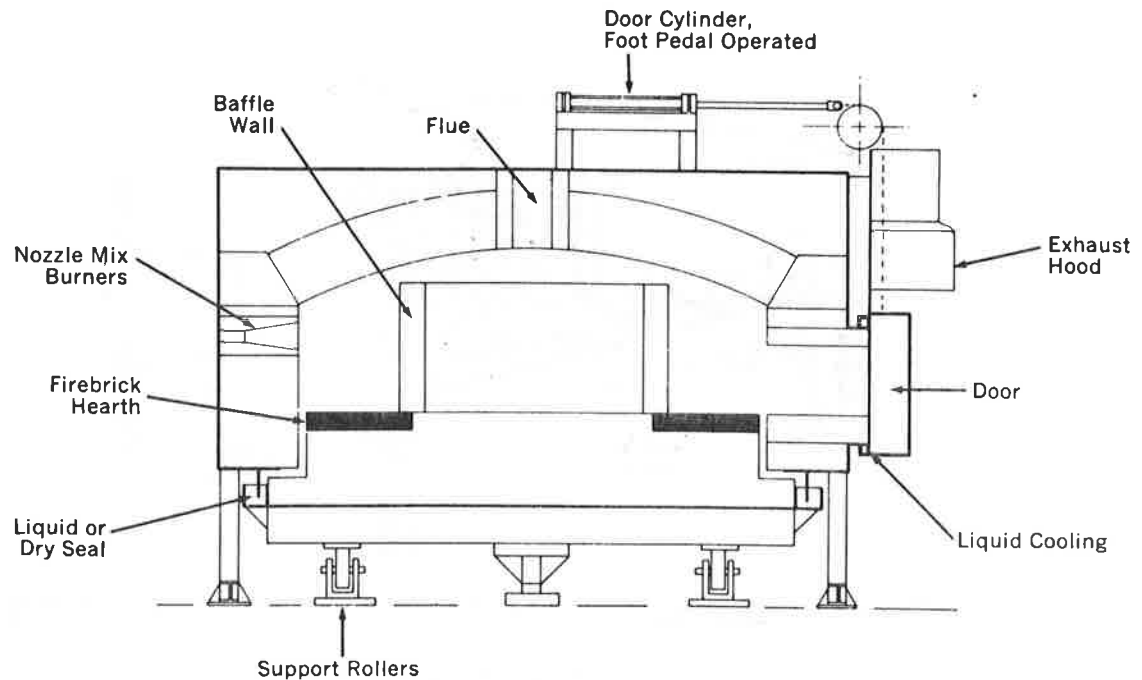
FIGURE 12 Rotary Hearth
