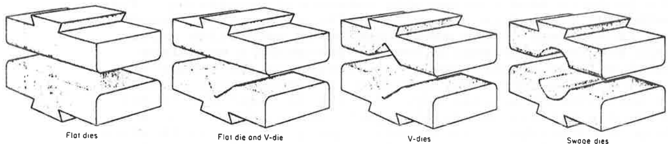
FIGURE 1 Four Types of Die Sets Commonly Used in Open-Die Forging
