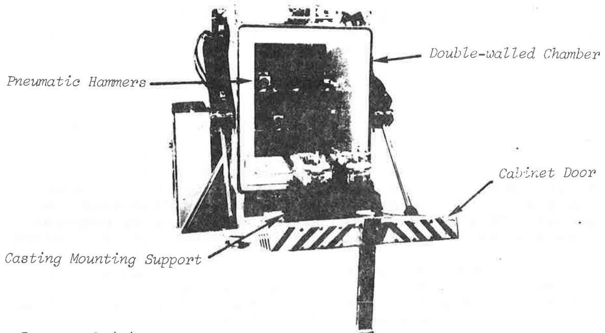
FIGURE 10 Pneumatic Hammer Decorating Cabin
