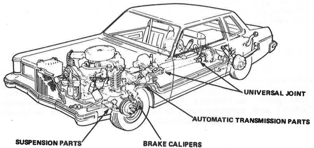
FIGURE 5 Malleable Iron Sand Castings on an Automobile
