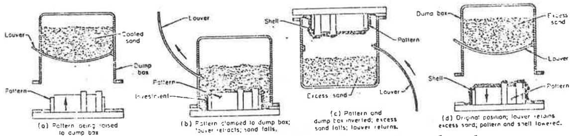
Variation B: Shell mold made by using a louver type dump box
