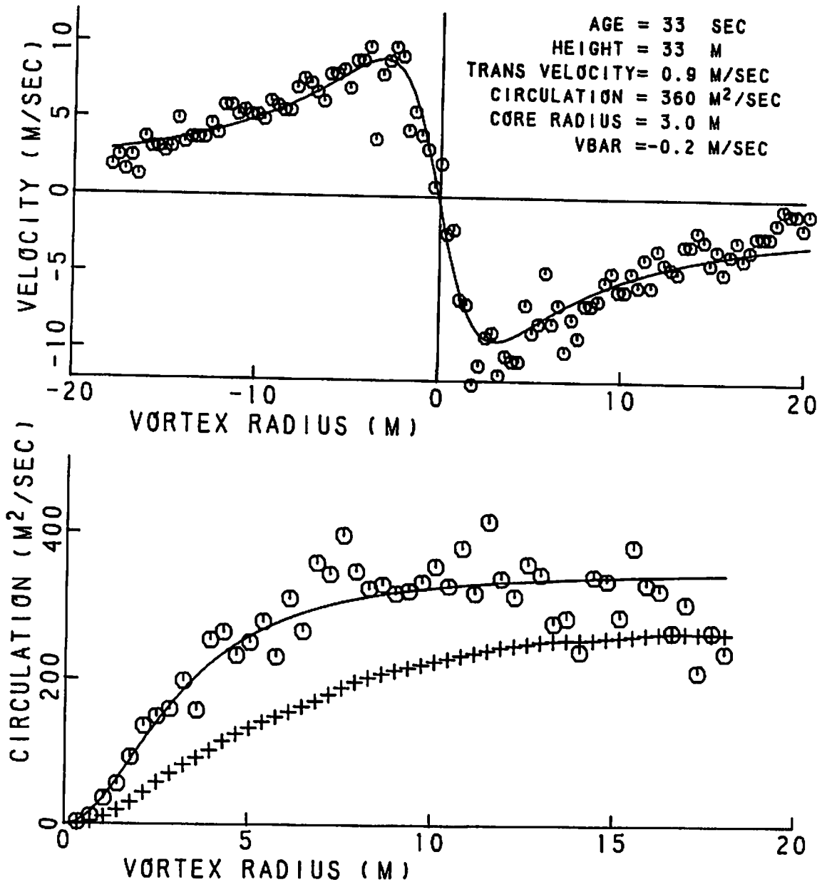
FIGURE 5. VORTEX VELOCITY AND CIRCULATION PROFILES
