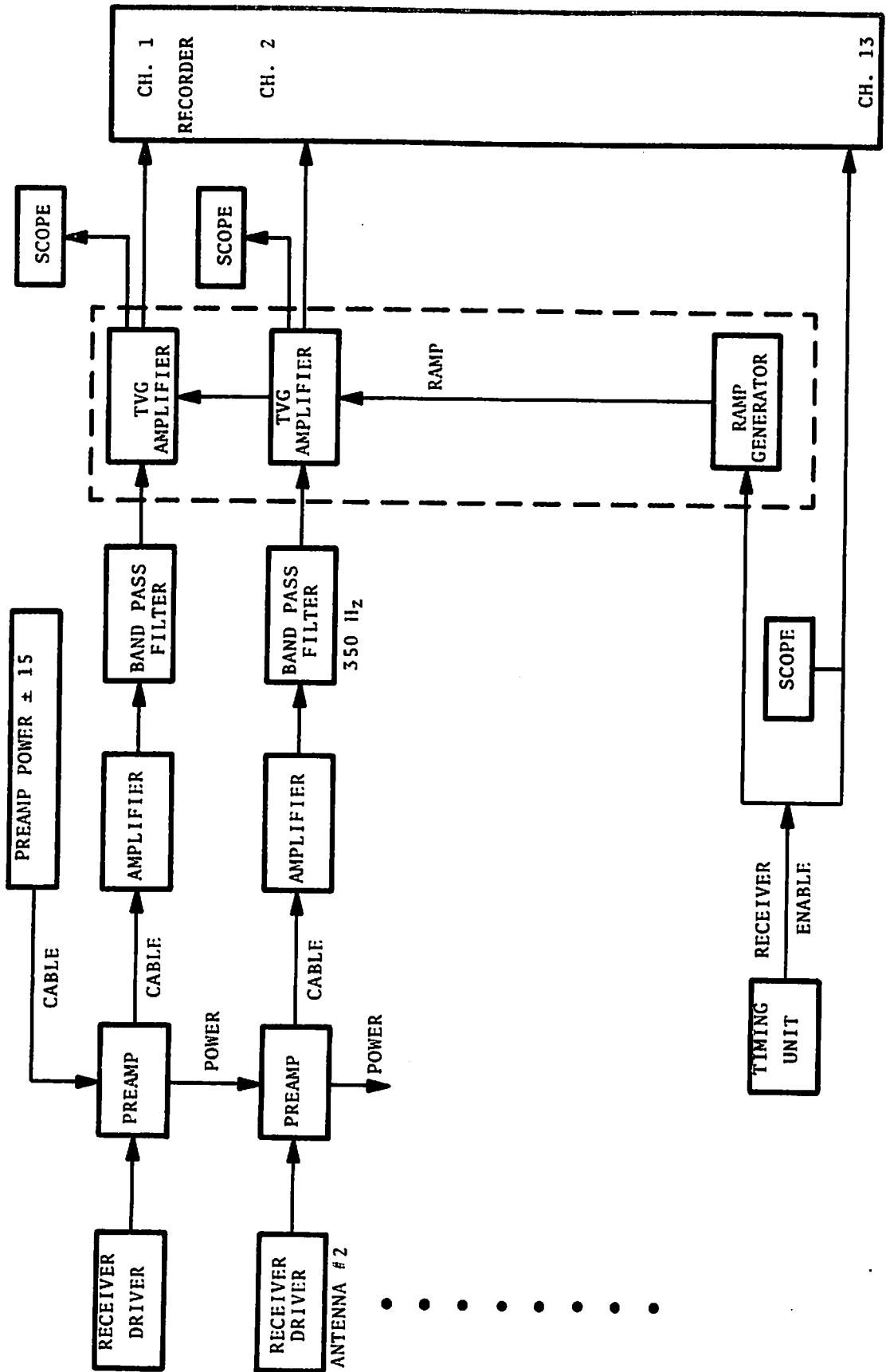
FIGURE 7. MAVSS RECEIVER AND RECORDING ELECTRONICS
