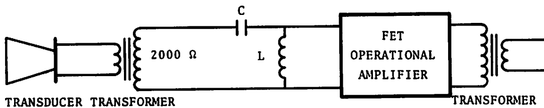
FIGURE 9. PREAMPLIFIER CIRCUIT DIAGRAM
