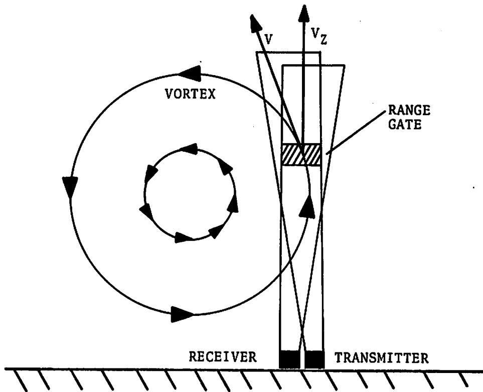
FIGURE 2. MONOSTATIC ACOUSTIC VORTEX SENSING SYSTEM (MAVSS) CONFIGURATION
