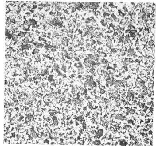
B. Heat-affected zone. 300 dph. X500.
