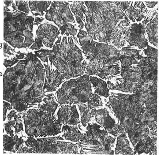
B-2. 300 dph. X500.
