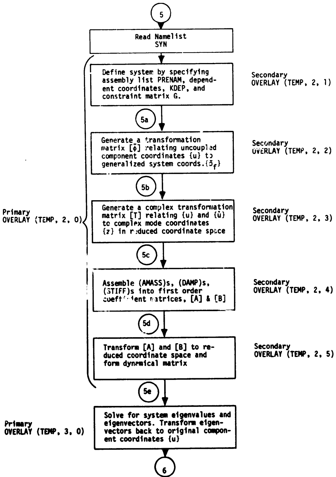
Figure 1d. Flow Diagram for Segment 3.
