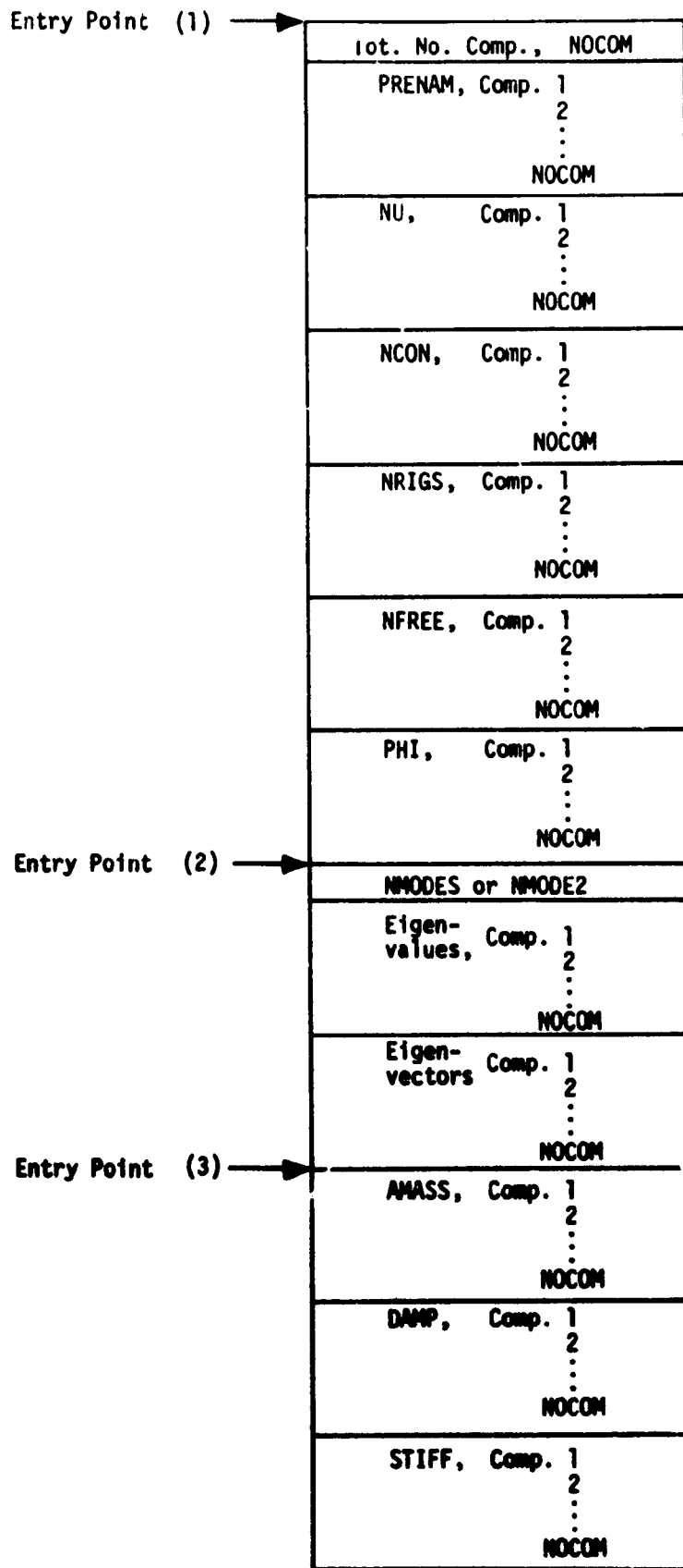
Figure 2. Layout of Component Data File (C.D.F.)
