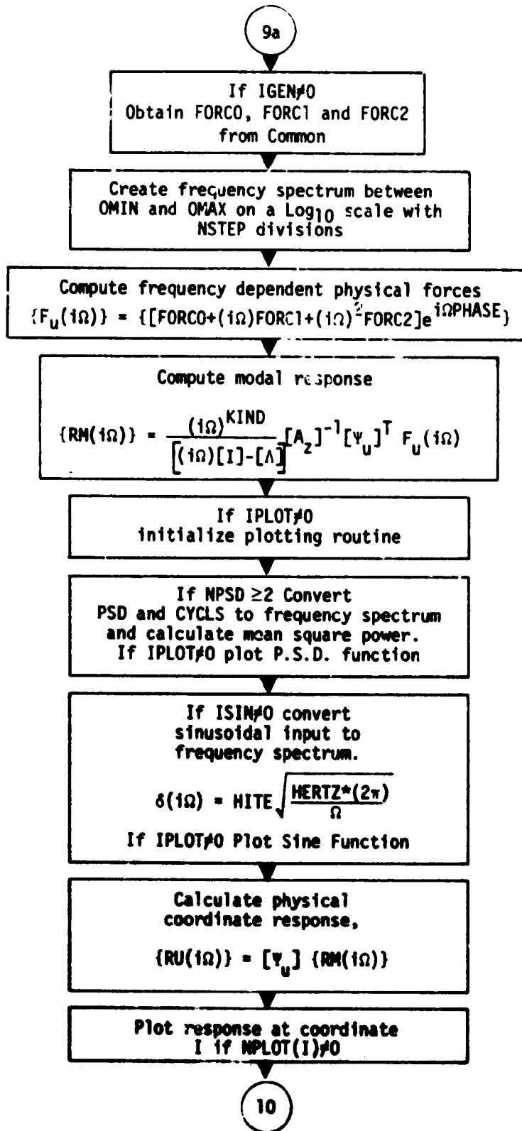
Figure 1m. Flow Diagram for OVERLAY (4.2)
