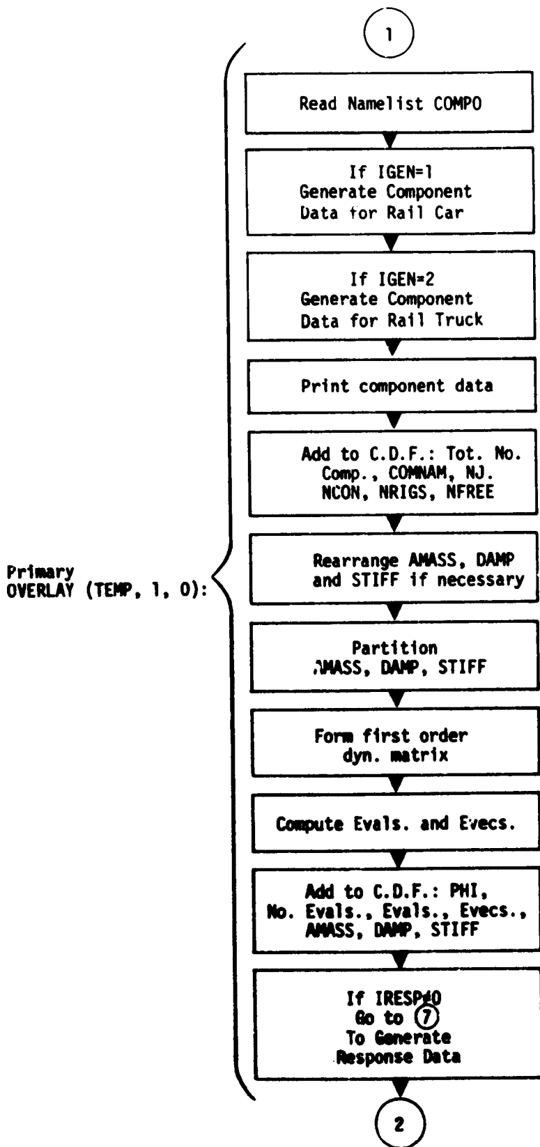
Figure 1b. Flow Diagram for Segment 1
