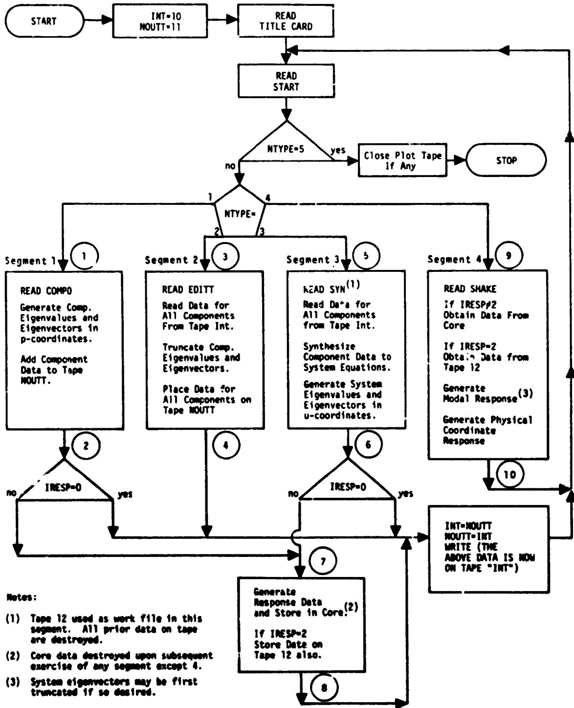
Figure 1a. DYNALIST II Flow Diagram
