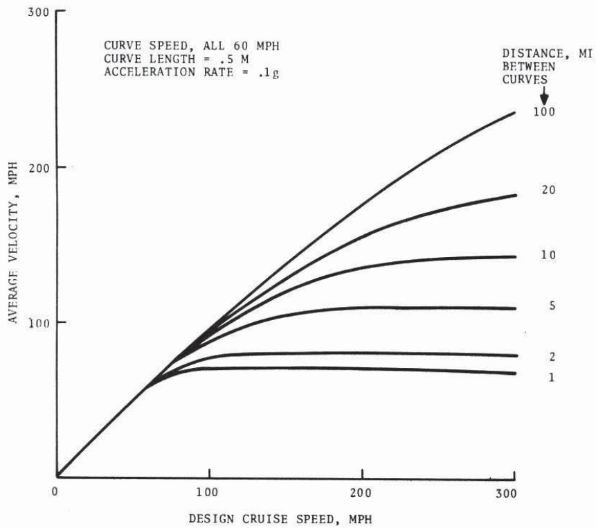
Figure 4-17. Average Velocity Versus Design Cruise Speed for Various 60 MPH Curve Densities, Chicago-Detroit
