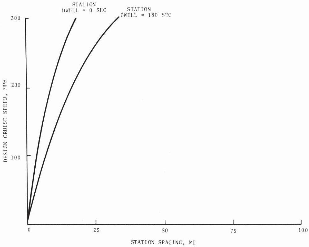
Figure 2-33. Design Cruise Speed Vs. Station Spacing and Dwell Time
