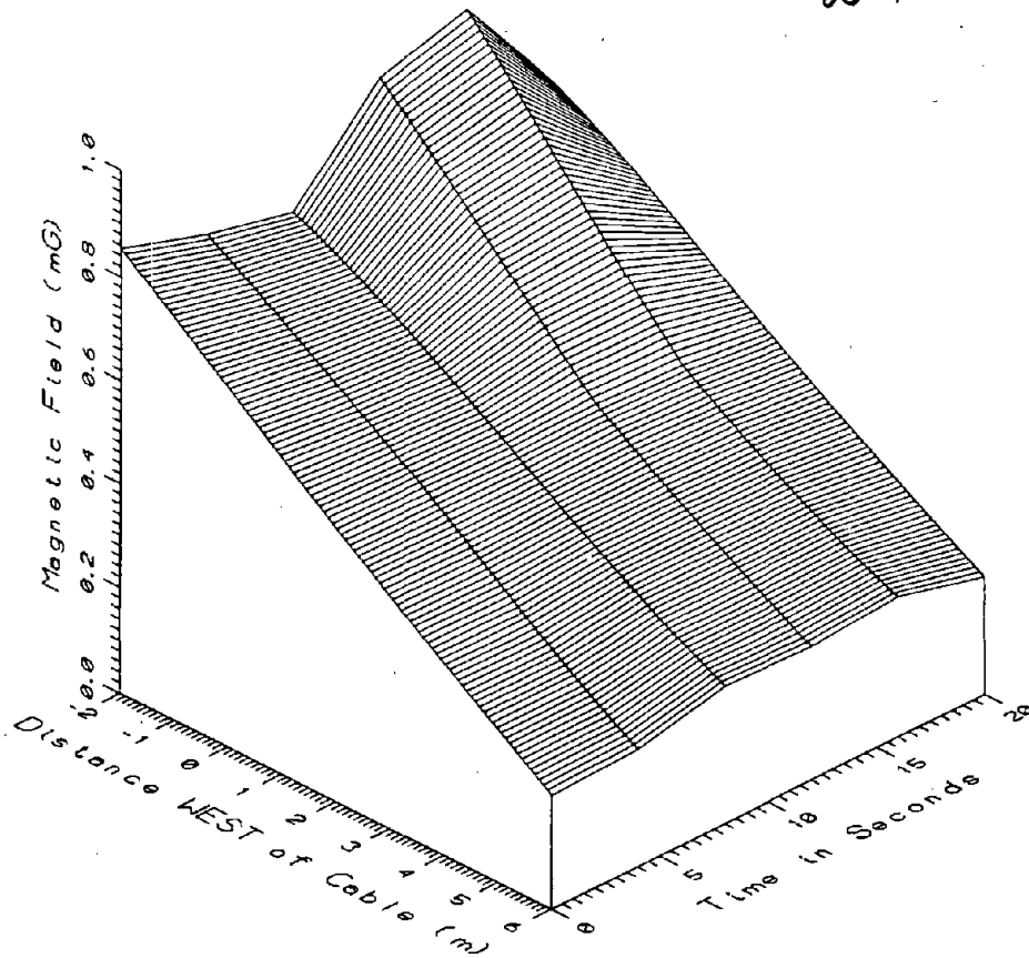
TR7028. BURIED CABLE FEEDING INVERTER BUILDING - ALL FREQUENCIES, 5-2560Hz
