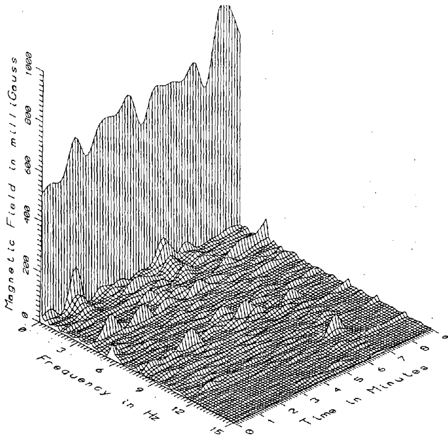
TR7008 - SEAT LEVEL - WINDOW SEAT AT REAR OF PASSENGER SECTION, CAR#2
