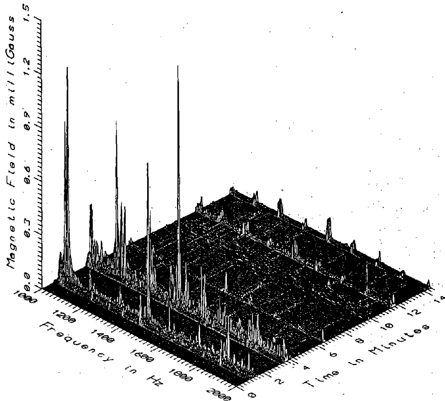
TR7030 - 15M NORTH OF INVERTER BUILDING
