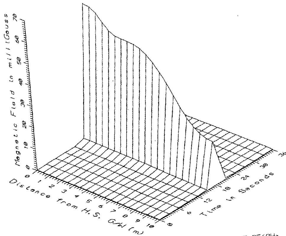
TR015, HIGH STEEL GUIDEWAY - ALL FREQUENCIES, 5-2560Hz
