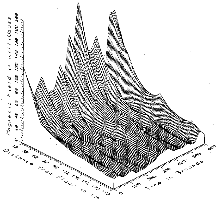
TR7002, AISLE SEAT IN MIDDLE OF PASSENGER SECTION, CAR2 - LOW FREQUENCY, 5-45Hz
