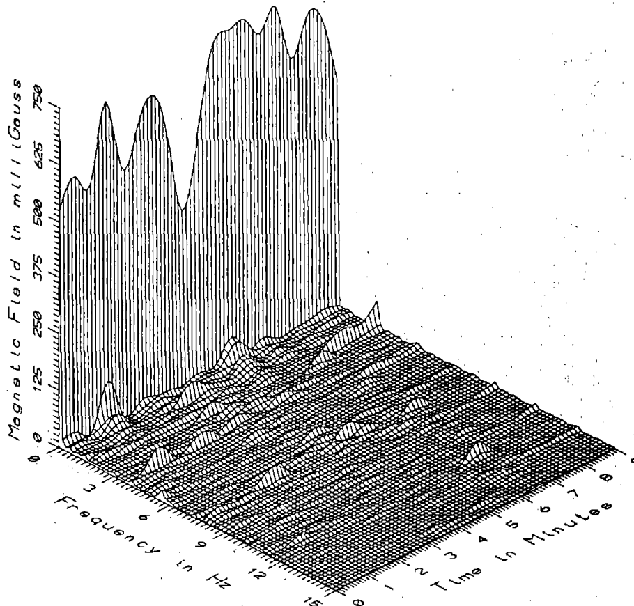
TR7008 - SEATED HEAD LEVEL - WINDOW SEAT AT REAR OF PASSENGER SECTION, CAR#2
