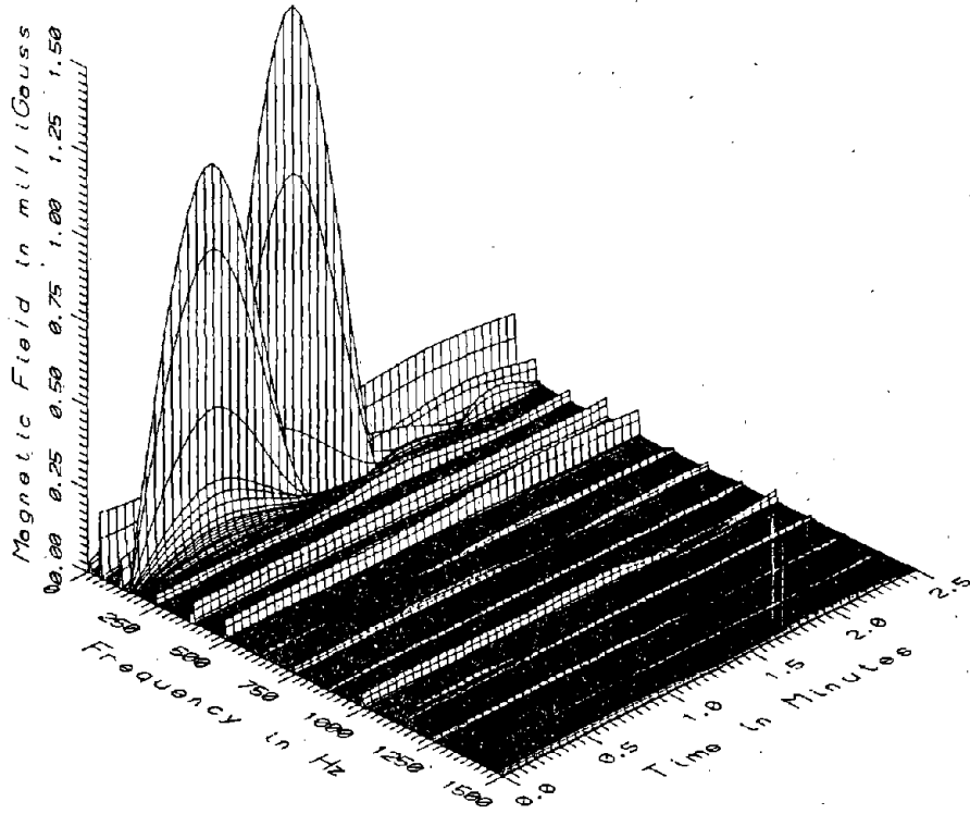
TR7012 - PROFILE OF HIGH STEEL GUIDEWAY - 10M FROM CENTER OF GUIDEWAY
