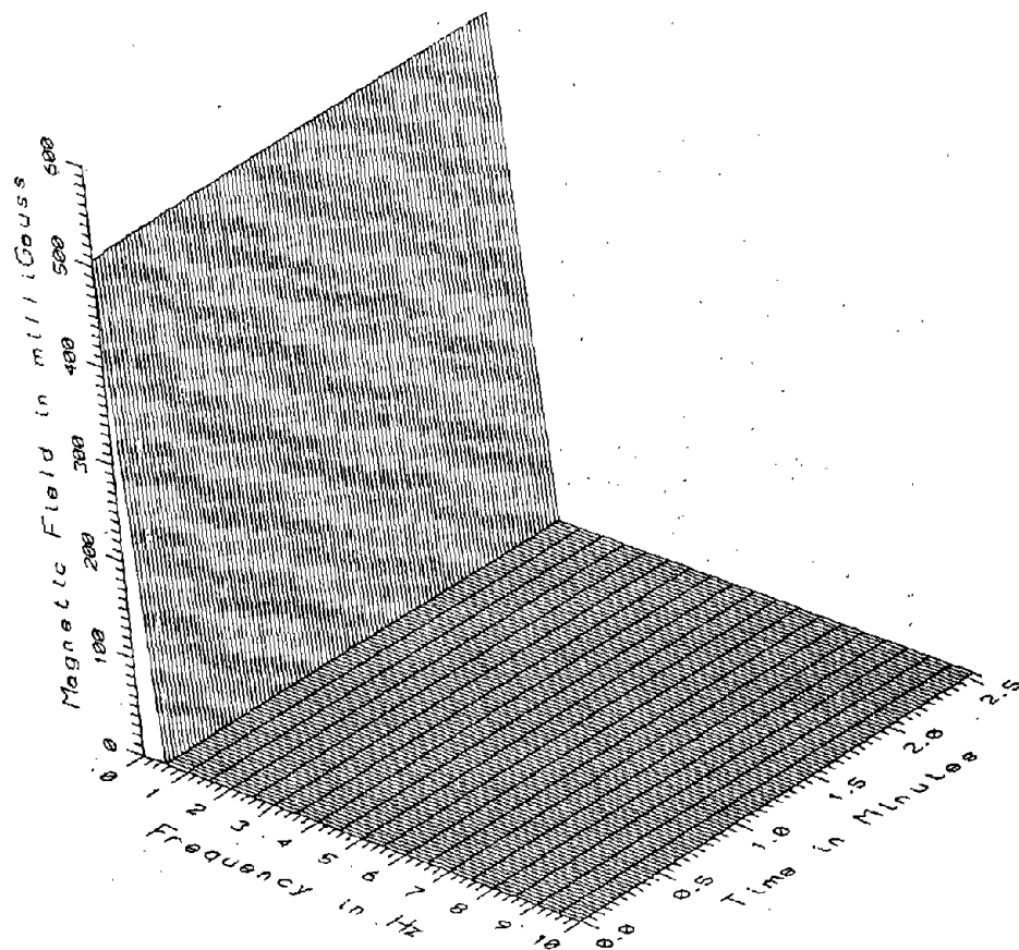
TR018 - 3M WEST OF HIGH STEEL GUIDEWAY, 25M NORTH OF PROFILE
