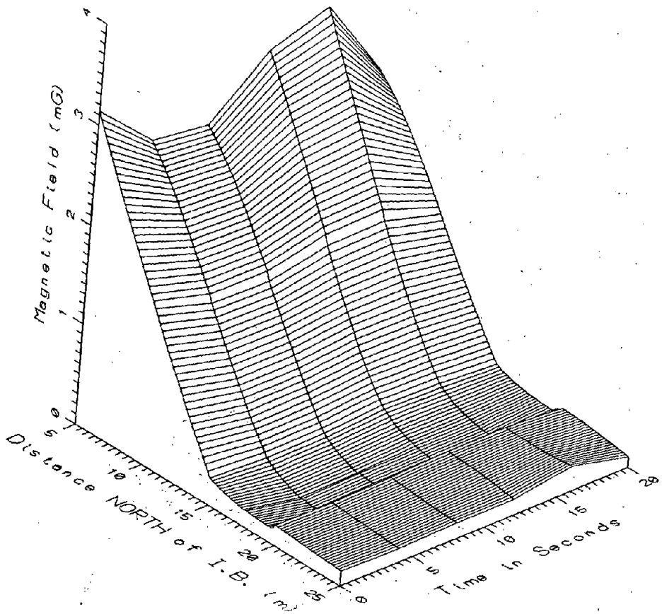
TR7028, INVERTER BUILDING - LOW FREQUENCY, 5-45Hz
