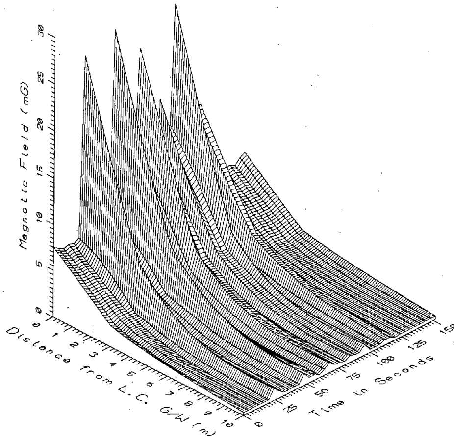
TR7026, LOW CONCRETE G/W OUTSIDE MAINTENANCE FACILITY - POWER HARM, 60-300Hz
