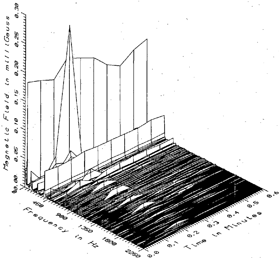
TR7025 - 3M NORTHWEST OF LOW CONCRETE GUIDEWAY OUTSIDE MAINTENANCE FACILITY
