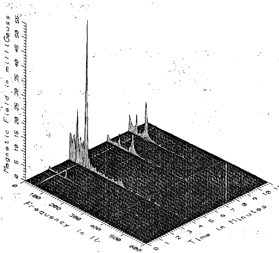
TR7013 - 311 WEST OF HIGH STEEL GUIDEWAY
