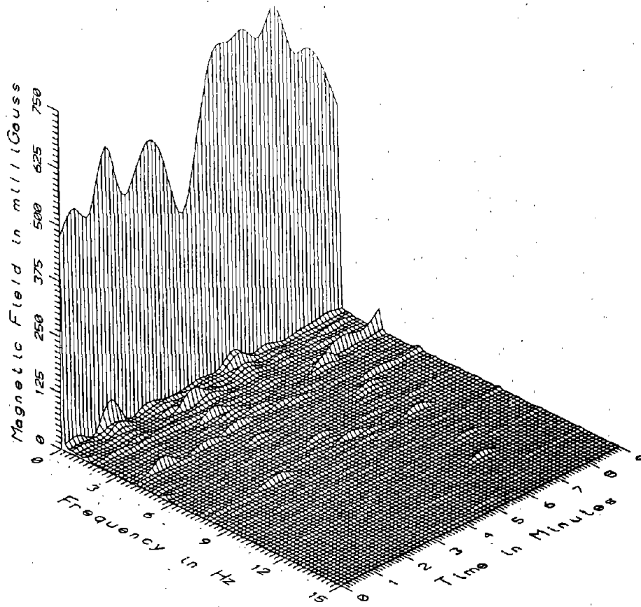
TR7008 - STANDING HEAD LEVEL - WINDOW SEAT AT REAR OF PASSENGER SECTION, CAR#1
