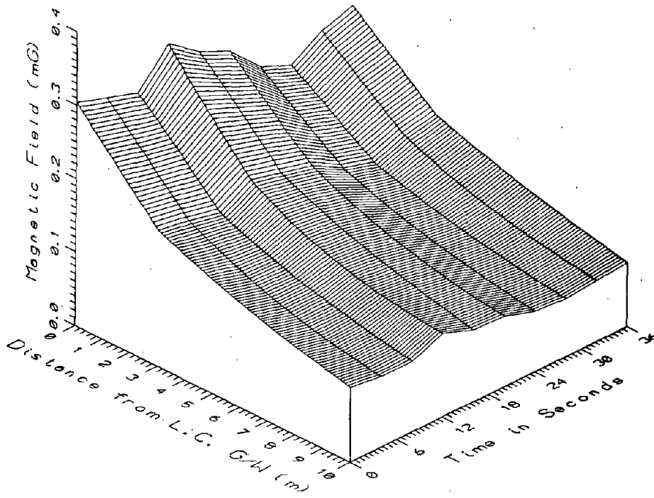
TR7025, LOW CONCRETE G/W OUTSIDE MAINTENANCE FACILITY - POWER FREQUENCY 50-60Hz
