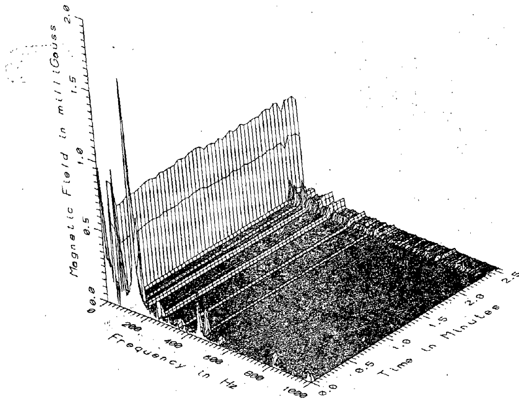
TR701B - 1M WEST OF OUTPUT TRANSFORMER YARD AND 7M EAST OF INVERTER BUILDING
