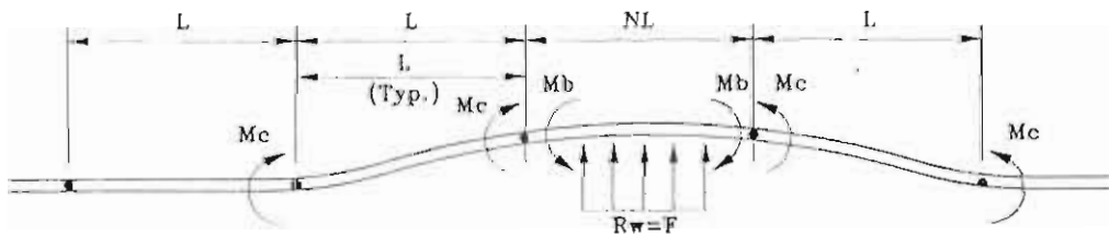
(C) THREE SPAN FAILURE MODE, N = 3
