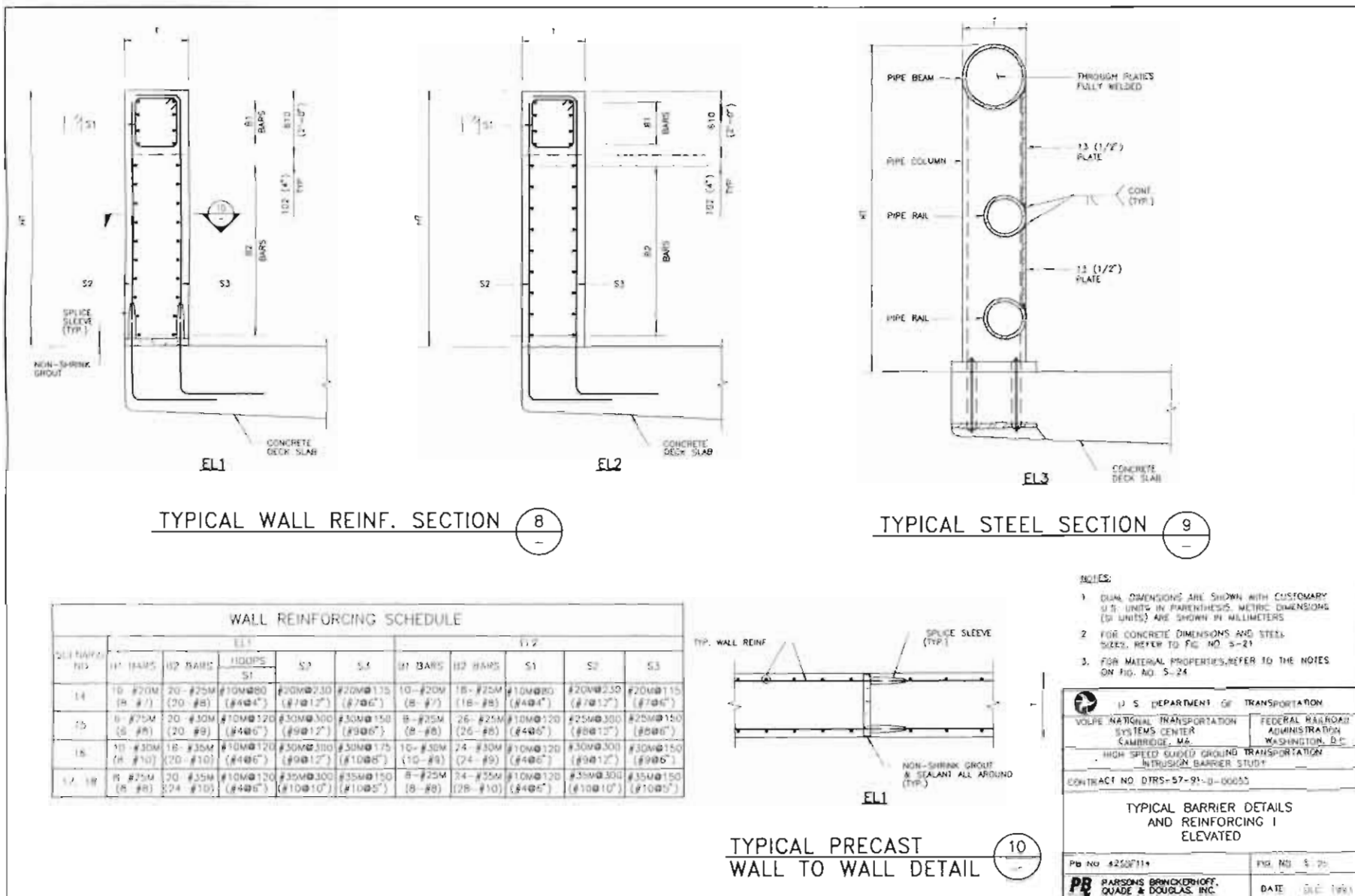
FIGURE 4-30. TYPICAL ELEVATED BARRIER DETAILS
