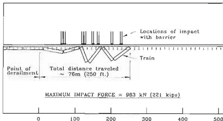
FIGURE 3-1. DERAILMENT/IMPACT MODEL
