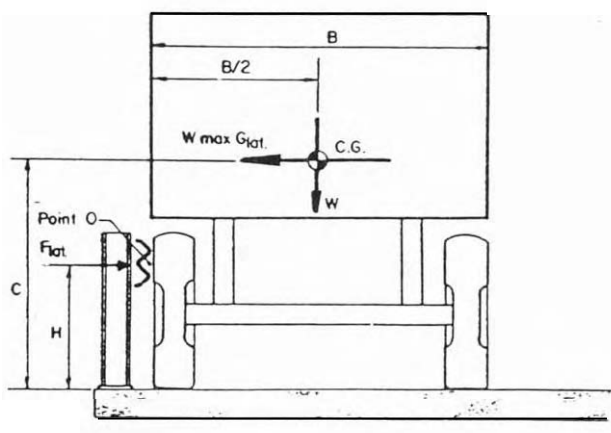
FIGURE 3-20. APPROXIMATE ANALYSIS OF BRIDGE RAIL EFFECTIVE HEIGHT REQUIRED TO PREVENT VEHICLE FROM ROLLING OVER RAIL [16]
