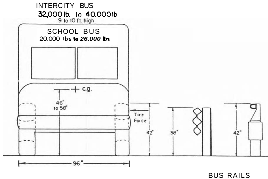
FIGURE 3-17. BASIC PROPERTIES OF BUSES AND TWO EFFECTIVE LONGITUDINAL RARRIERS [16]
