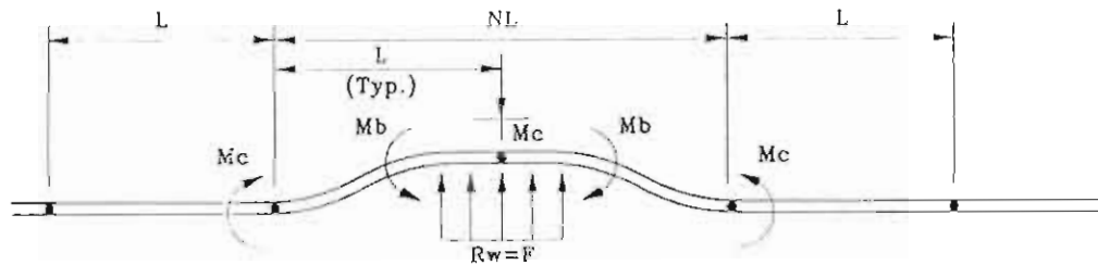
(B) TWO SPAN FAILURE MODE, N = 2
