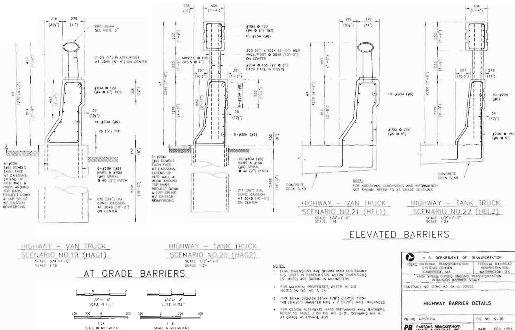
FIGURE 4-31. TYPE 1 AND 2 HIGHWAY BARRIER DETAILS
