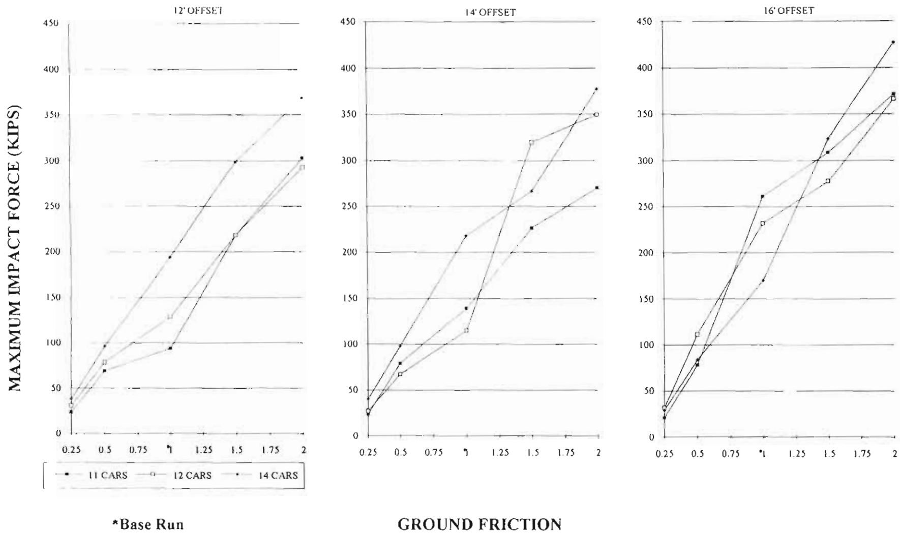
FIGURE 3-10. IMPACT FORCE VS. GROUND FRICTION
