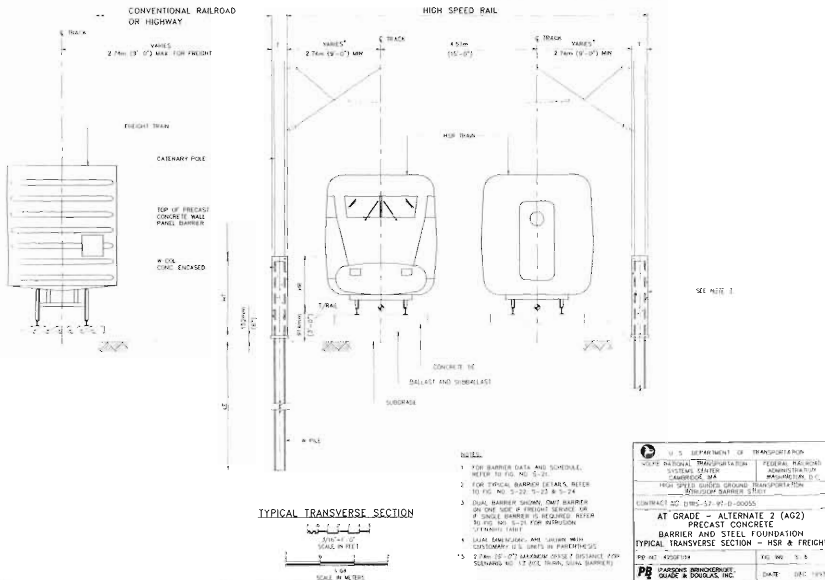
FIGURE 4-11. AT GRADE ALTERNATE 2: P/C WALL AND STEEL FOUNDATION - TRANSVERSE SECTION/RR
