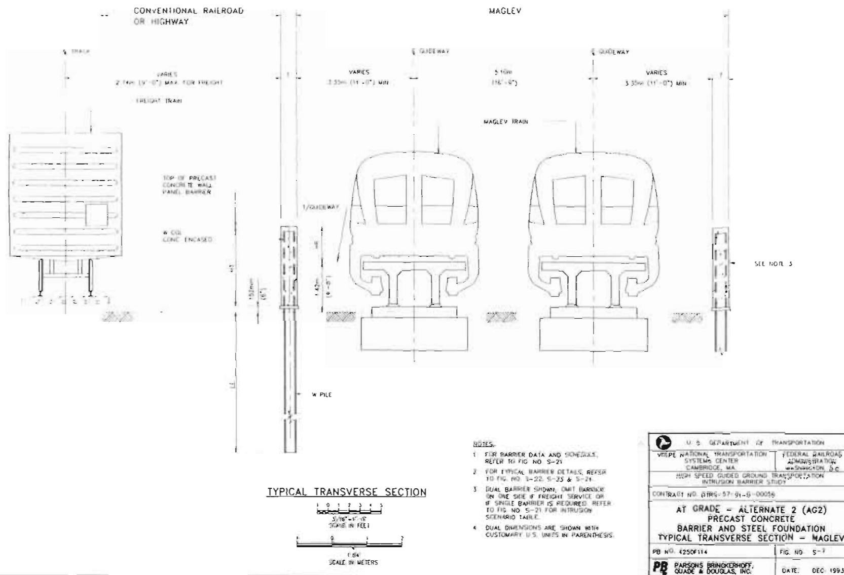
FIGURE 4-12. AT GRADE ALTERNATE 2: P/C WALL AND STEEL FOUNDATION - TRANSVERSE SECTION/MAGLEV
