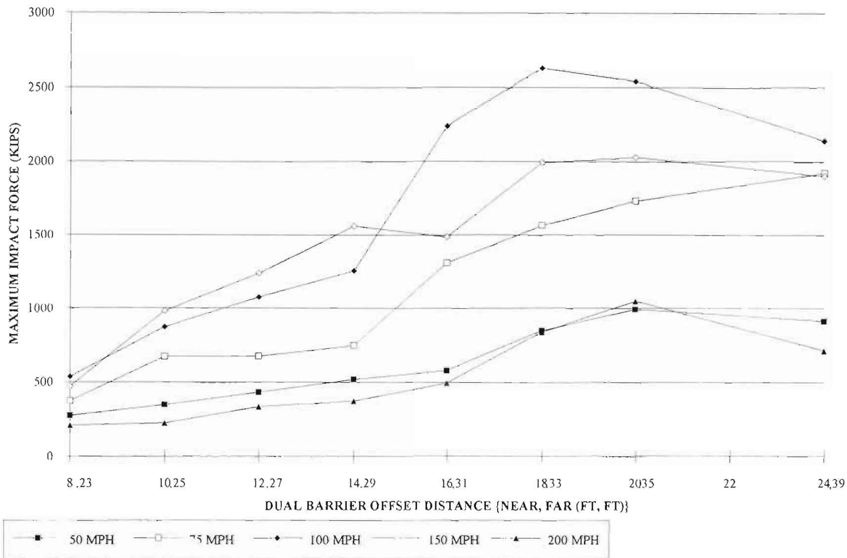
FIGURE 3-14. IMPACT FORCE VS. DUAL BARRIER OFFSET DISTANCE
