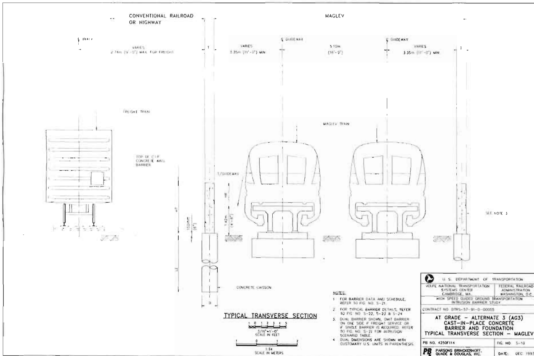
FIGURE 4-15. AT GRADE ALTERNATE 3: C.I.P. CONC. WALL AND C.I.P. CONC. FOUNDATION - TRANSVERSE SECTION/MAGLEV
