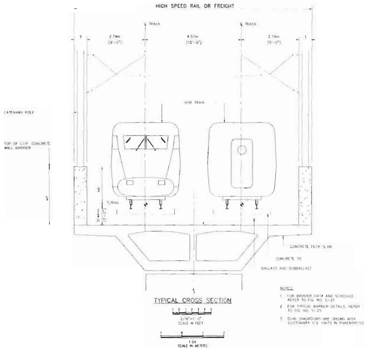
FIGURE 4-22. ELEVATED ALTERNATE 2: C.I.P. CONCRETE WALL - TRANSVERSE SECTION/RR
