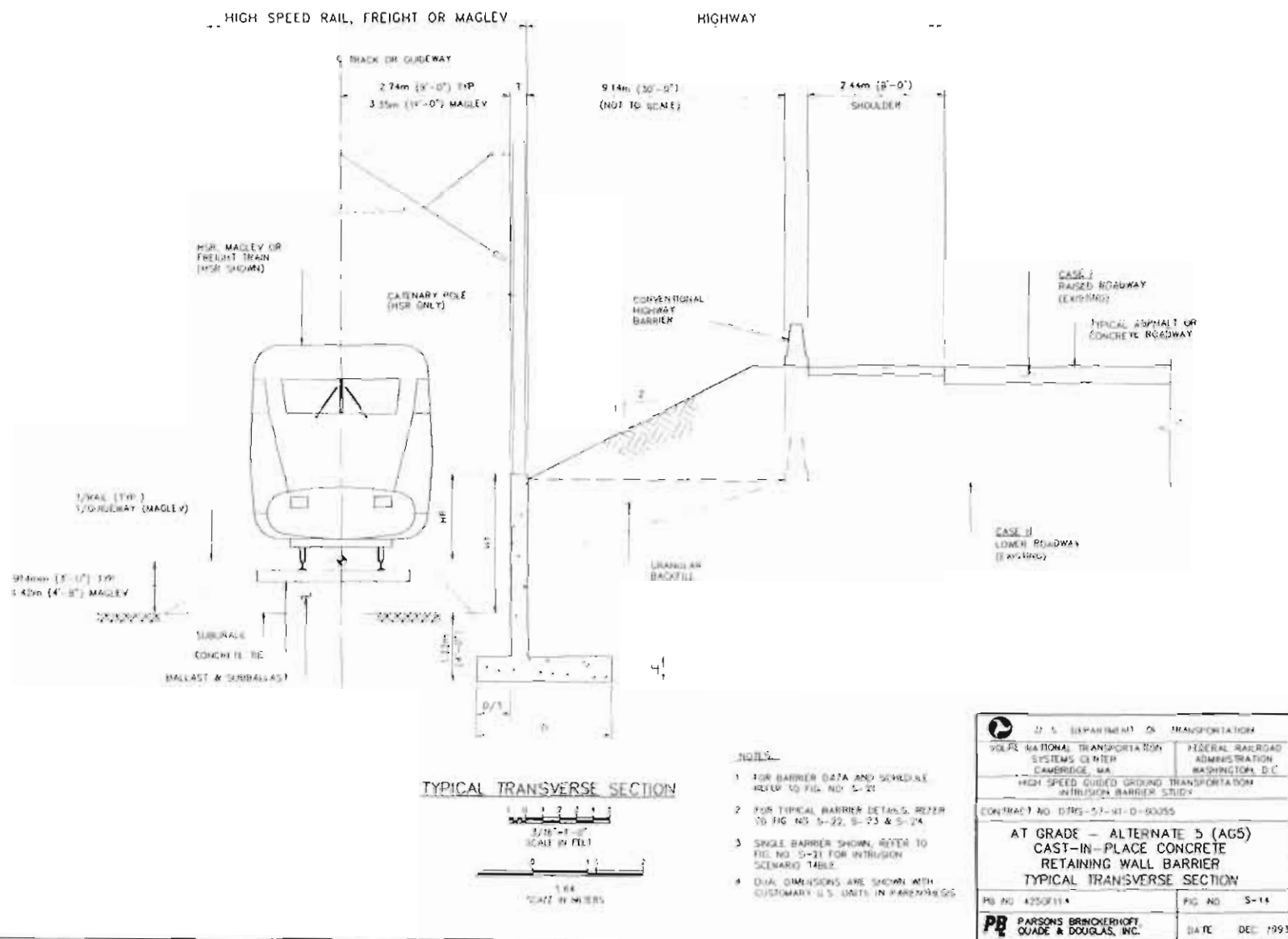
FIGURE 4-19. AT GRADE ALTERNATE 5: C.I.P. CONCRETE RETAINING WALL BARRIER - TRANSVERSE SECTION/RR & MAGLEV
