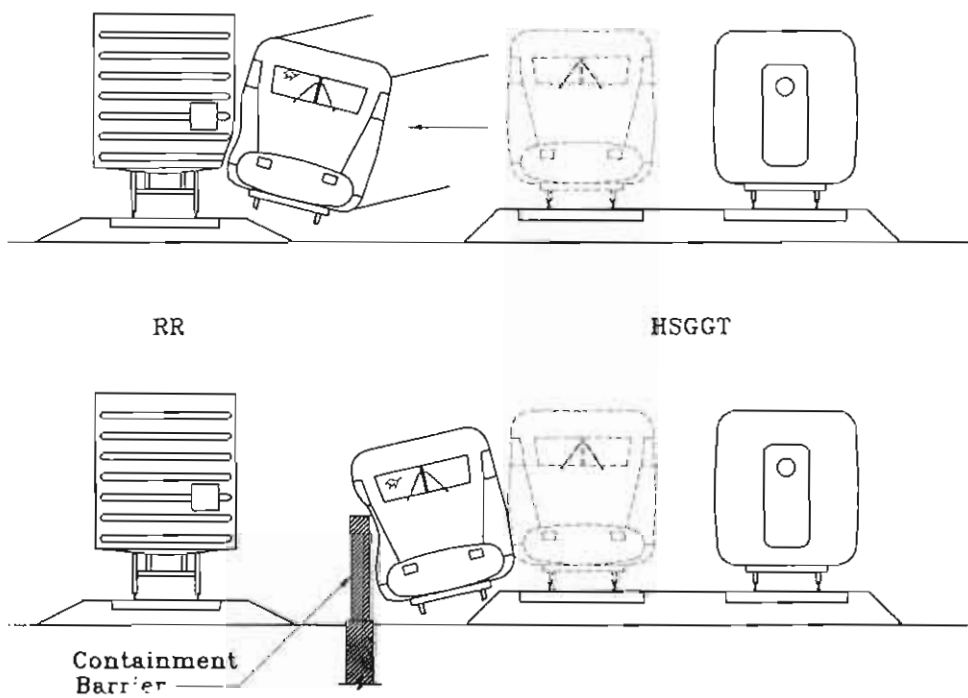
FIGURE 2-2. CONTAINMENT BARRIER
