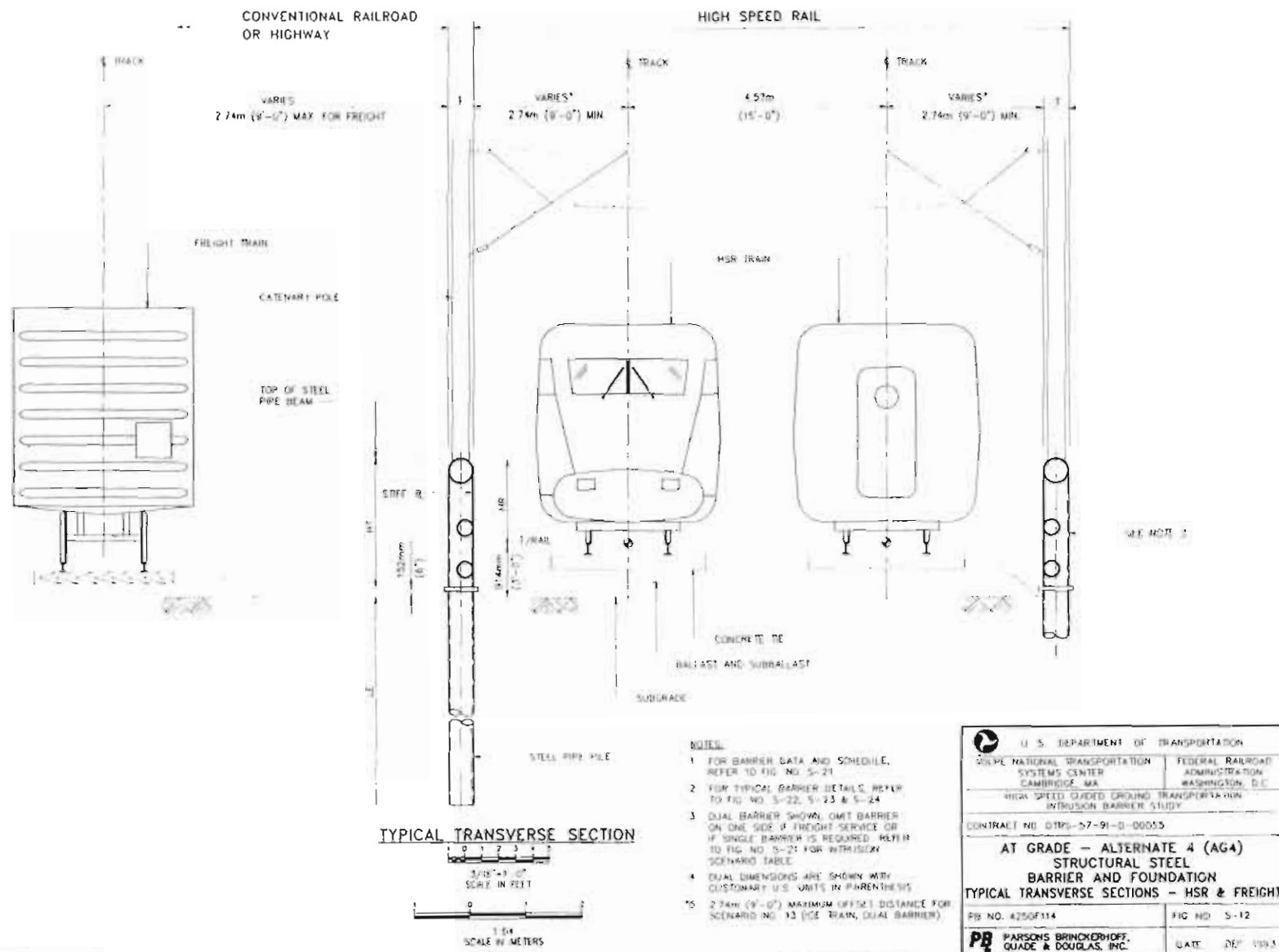
FIGURE 4-17. AT GRADE ALTERNATE 4: STRUCTURAL STEEL POST, RAILING AND FOUNDATION - TRANSVERSE SECTION/RR
