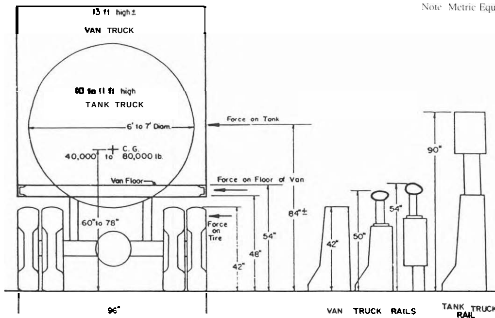
FIGURE 3-18. BASIC PROPERTIES OF TRACTOR-TRAILER TRUCKS (VAN AND TANK TYPES) AND SOME EFFECTIVE LONGITUDINAL RARRIERS [16]
