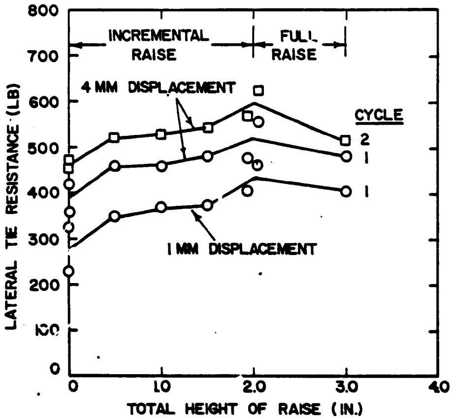
Figure 4.3. The Effect of the Height of a Tamping Raise on Lateral Tie Resistance
