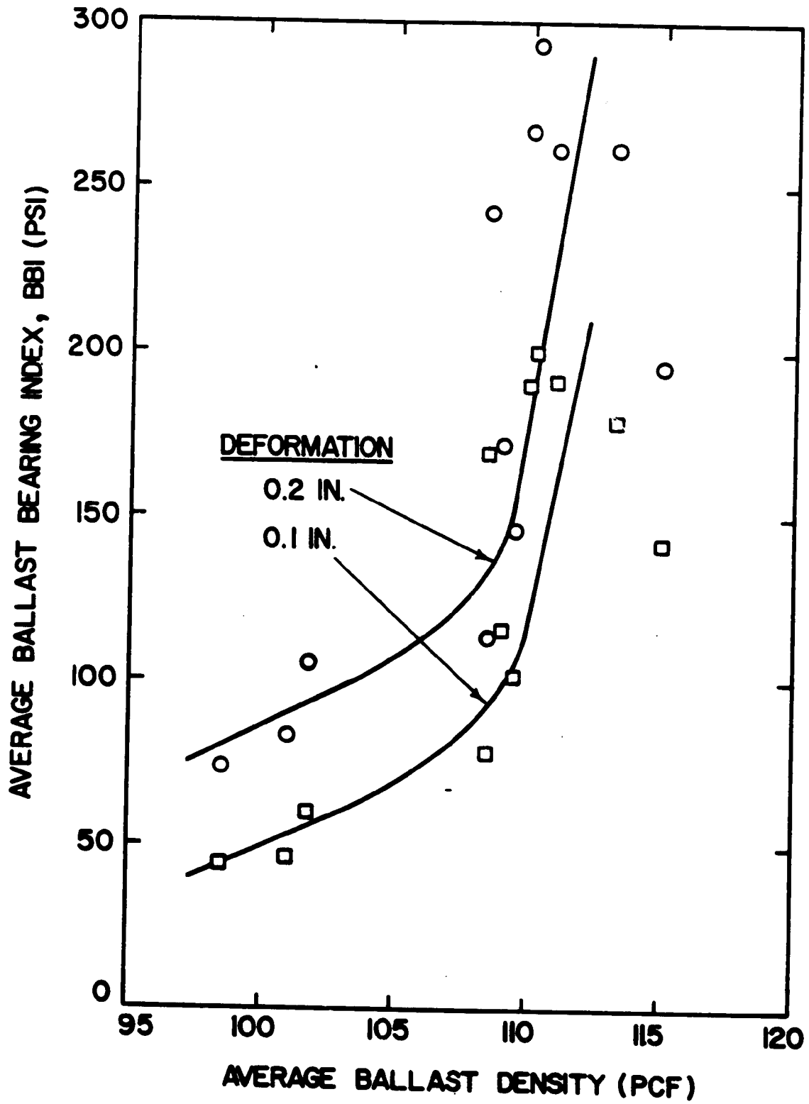
Figure 3.7. Strength-Density Relationship for the Simulated Track Bed
