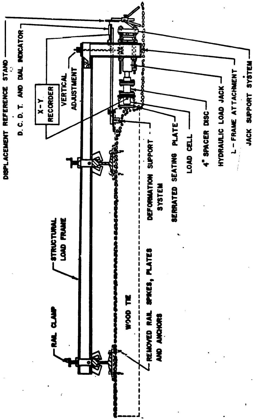
Figure 4.1.1. Assembled Lateral Tie Push Test Apparatus (Ref. 1)
