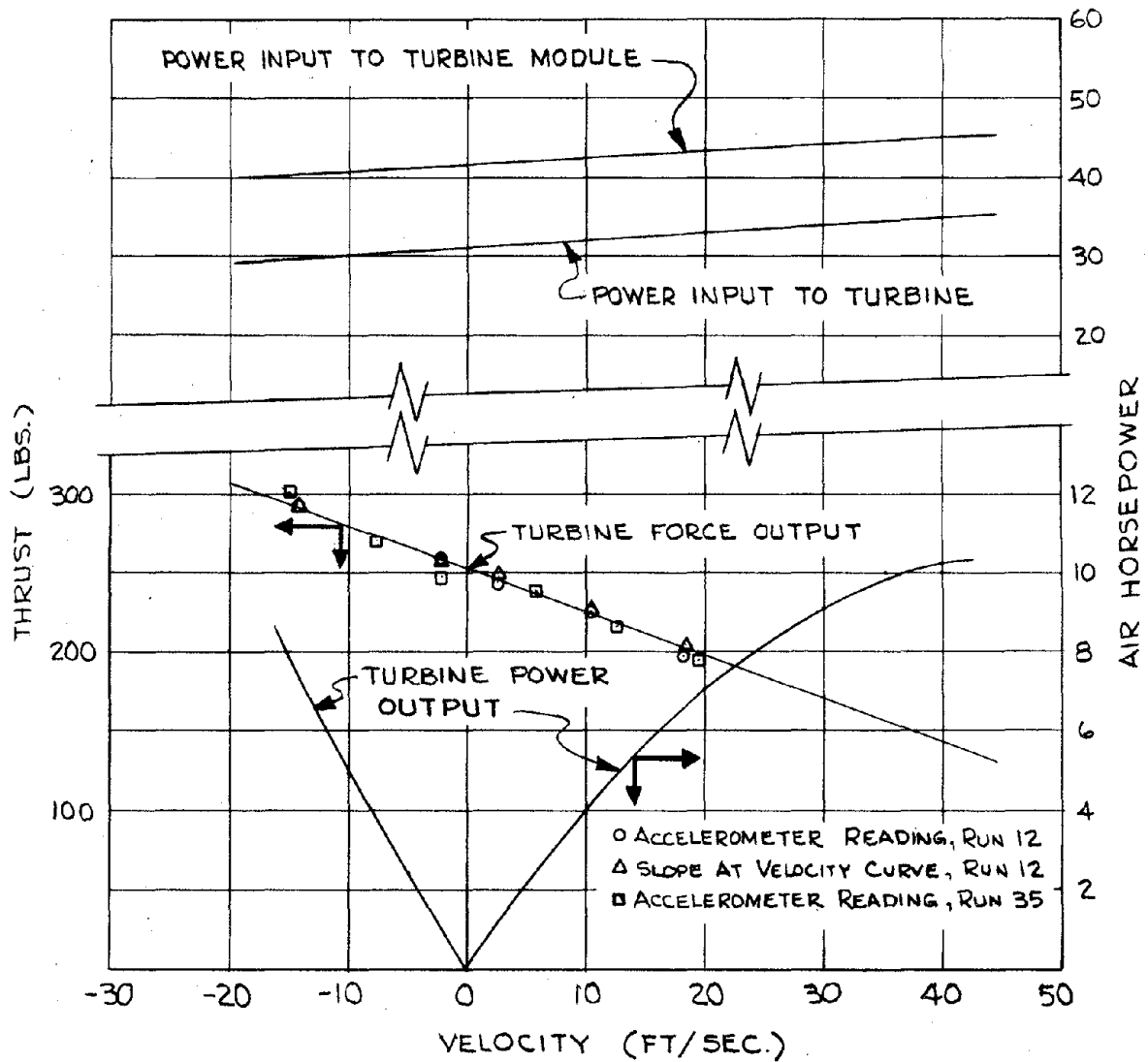
Figure 6-9. Turbine performance versus velocity.
