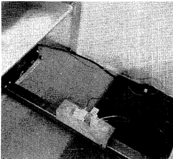
Figure 6-3. Accelerometer Installation.
