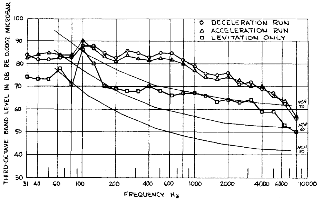
Figure 3-8. Sound pressure levels measured inside empty vehicle.
