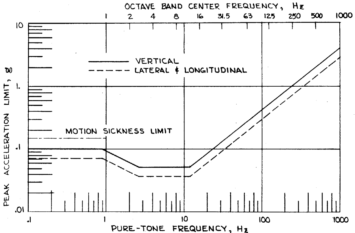
Figure 6-13. Permitted maximum vertical and lateral/longitudinal vibration levels on urban trips.
