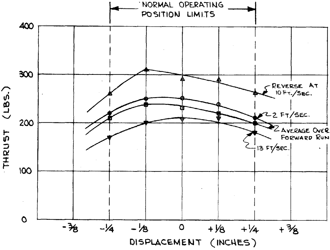
Figure 6-11. Thrust versus lateral displacement of vehicle.
