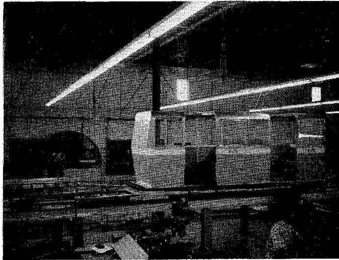
Figure 6-1. Vehicle entering arresting mechanism.
