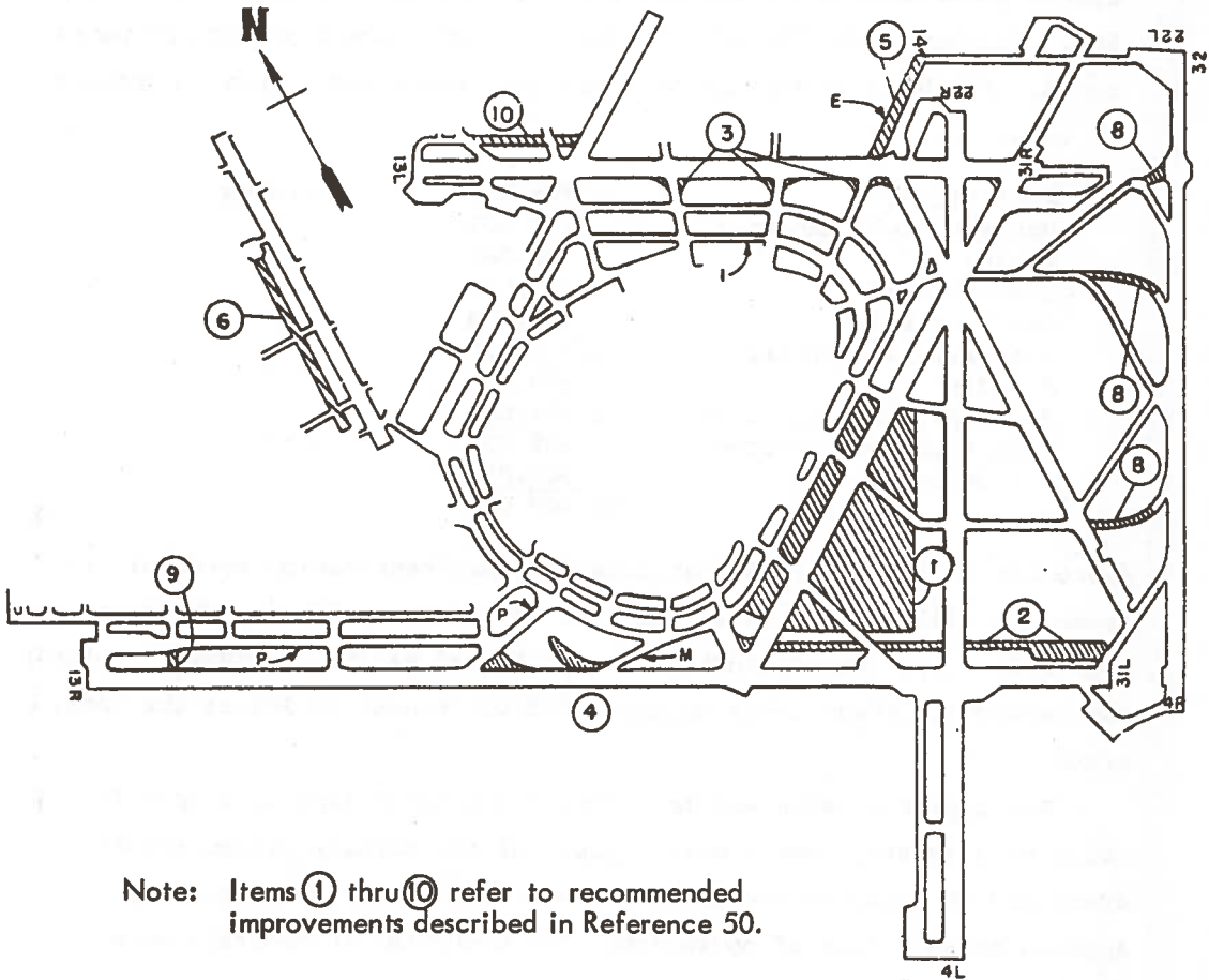
Figure 24 Taxiway Network -- Kennedy Airport
