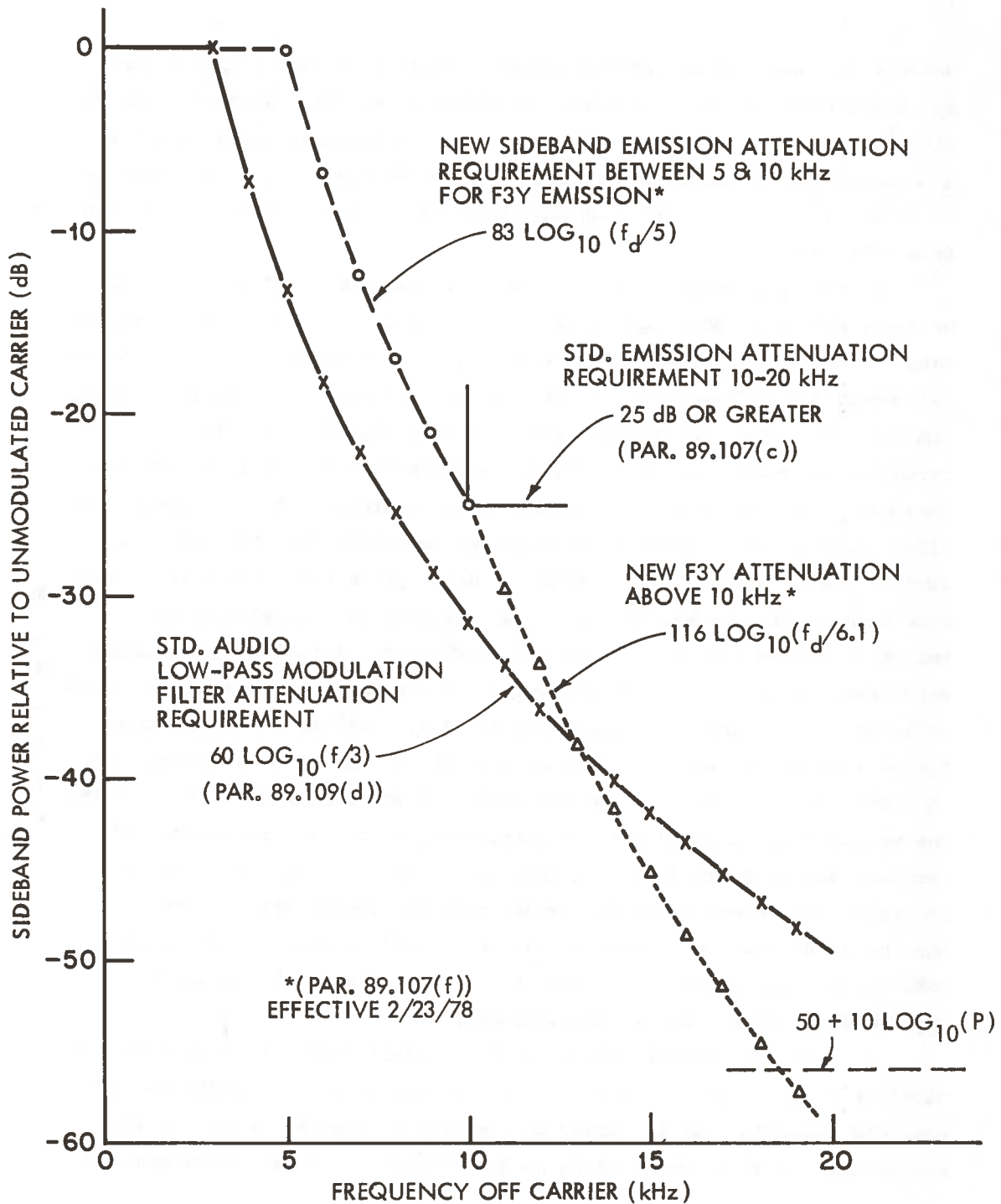
Figure 30 Comparison of Standard Audio Low-Pass Filter and New Emission-Attenuation-Based Rolloff for F3Y Digital Modulation
