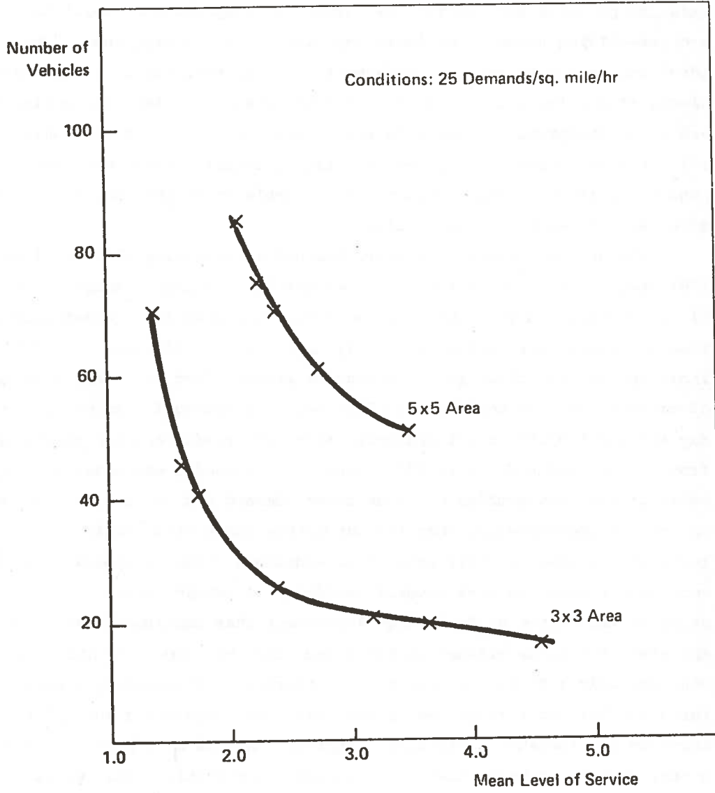
Figure 23 Relationships between Number of Vehicles and Level of Service (Many-to-Many DAR, 25 Demands/sq. mile/hr.)
