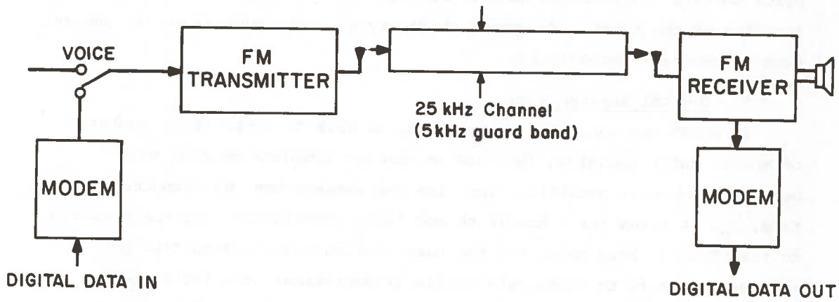
Figure 28 Digital Data Transmission via FM Voice Radios
