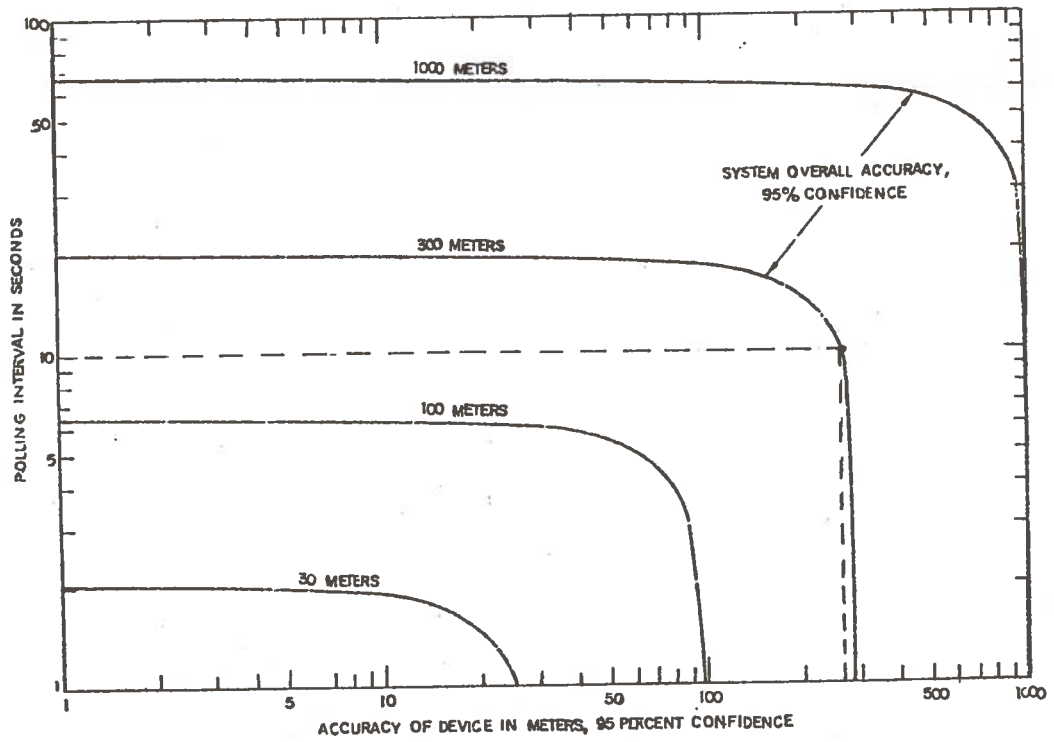
Figure 16 AVL System Accuracy versus Update Rate
