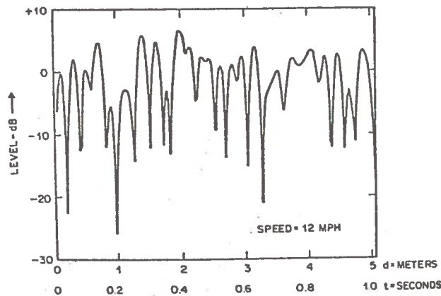
Figure 27 Typical Fading Envelope Measured at a Carrier Frequency of 850 MHz
