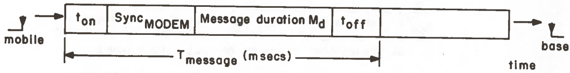
Figure 29 Time Components of a Mobile-to-Base Transmission
