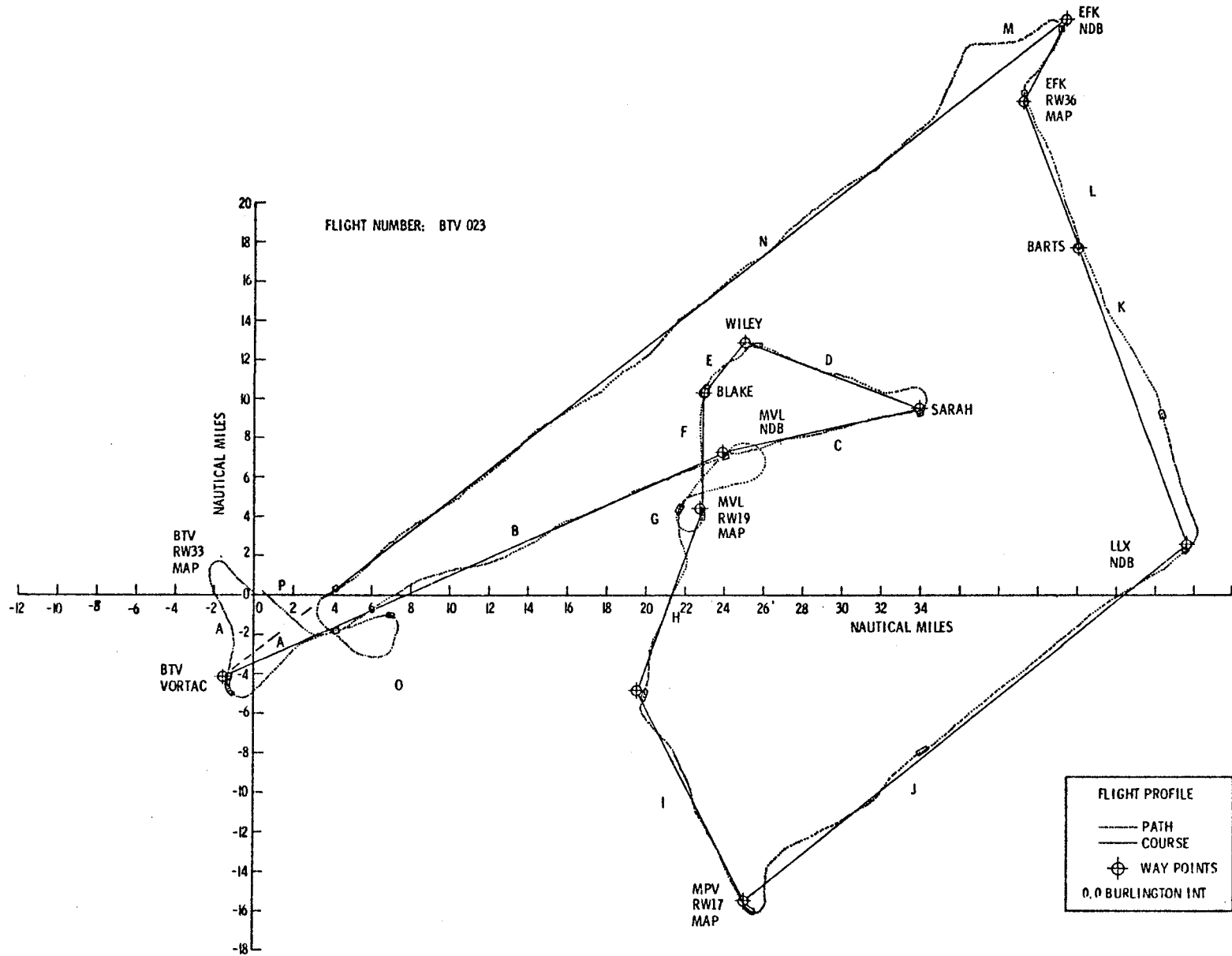
FIGURE 2.1-7. FLIGHT PROFILE FOR FLIGHT BTV 023
