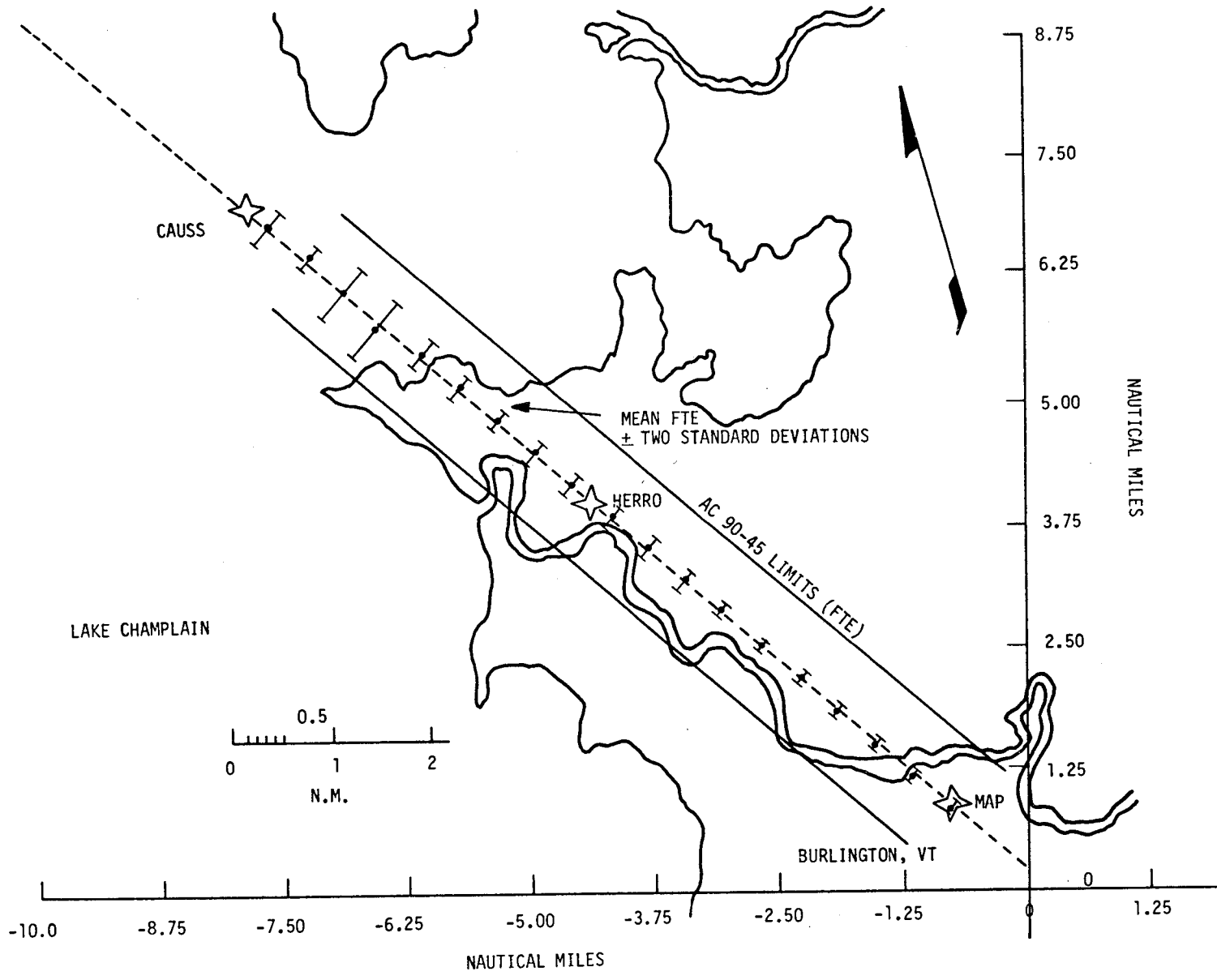
FIGURE 2.1-15. IMPROVEMENT IN FTE ALONG THE APPROACH
