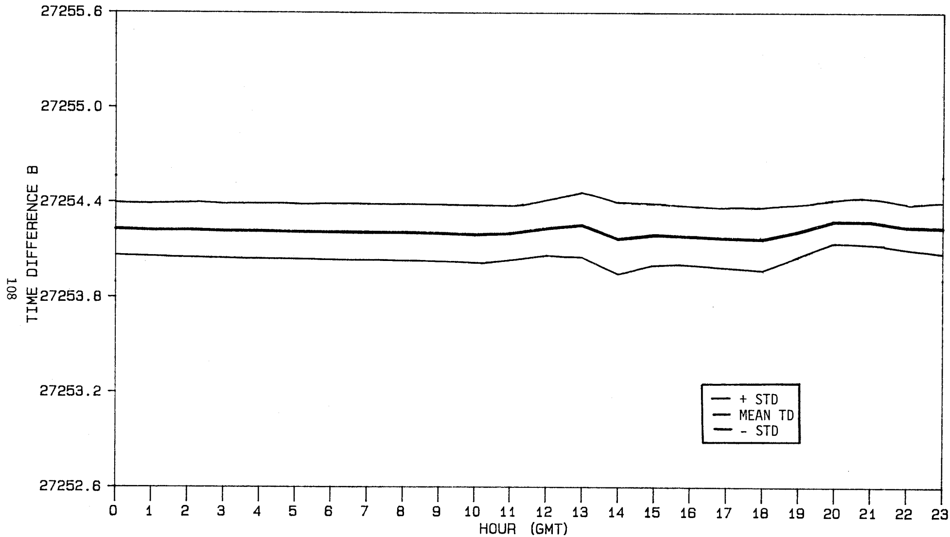
FIGURE 2.3-16. DIURNAL TD VARIATIONS FOR NANTUCKET (TDL-711) AT BURLINGTON
