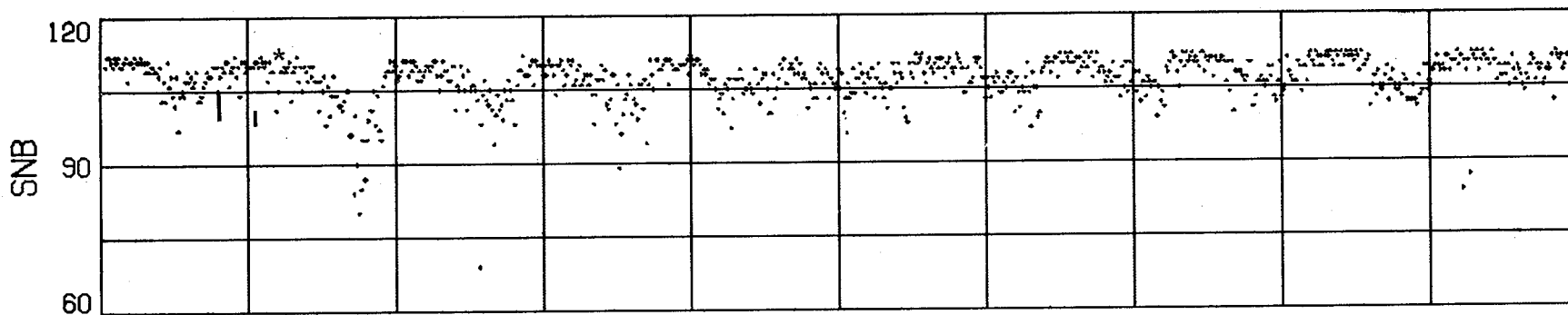
FIGURE 2.3-6. SNR TIME HISTORY FOR NANTUCKET AT BURLINGTON (13 NOV 79 TO 28 NOV 79)
