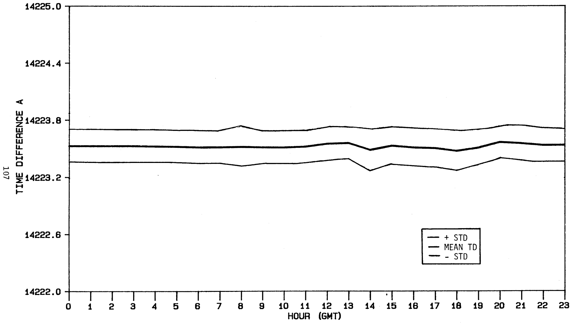
FIGURE 2.3-15. DIURNAL TD VARIATIONS FOR CARIBOU (TDL-711) AT BURLINGTON
