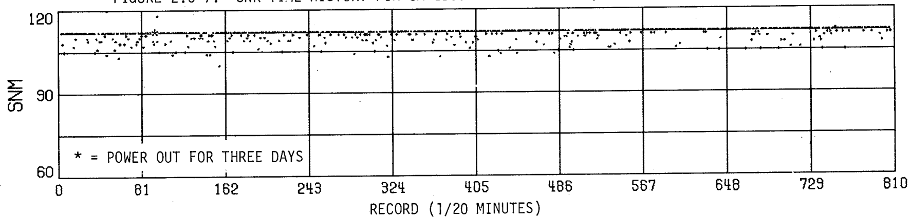
FIGURE 2.3-8. SNR TIME HISTORY FOR SENECA AT BURLINGTON (13 NOV 79 TO 28 NOV 79)
