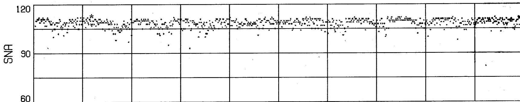
FIGURE 2.3-7. SNR TIME HISTORY FOR CARIBOU AT BURLINGTON (13 NOV 79 TO 28 NOV 79)
