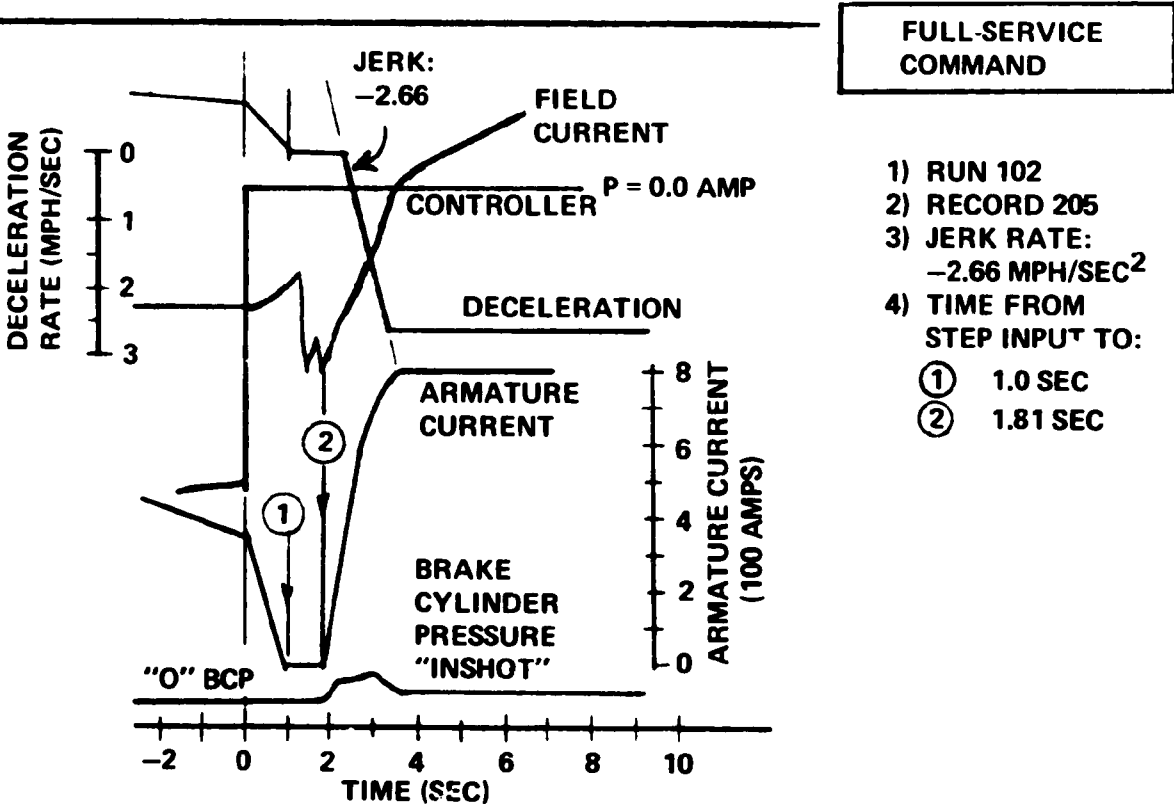
Figure 3-5. Blended Breaking Deadtime and Jerk Rate (105,000-Pound Car).
