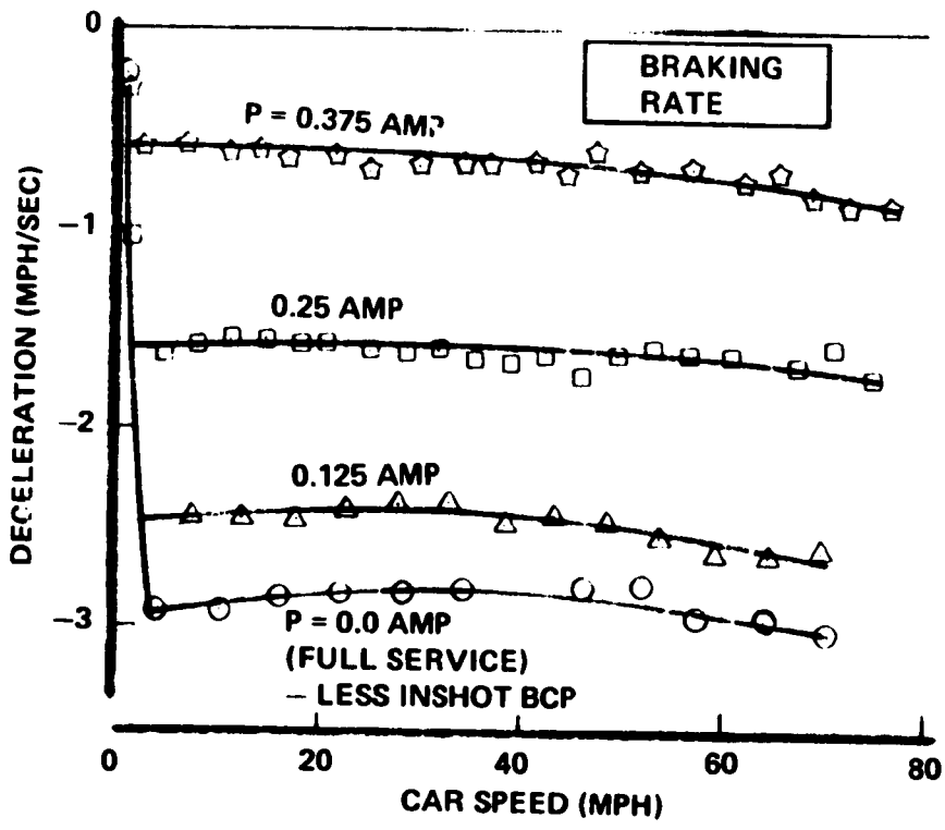
Figure 3-14. Dynamic Braking Only Control Characteristics (105,000-Pound Car)
