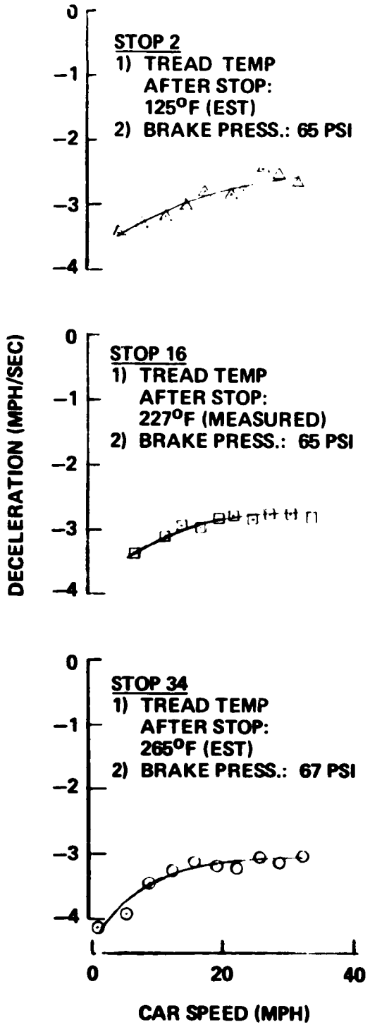
Figure 5-4. Duty Cycle I Friction Braking Deceleration (105,000-Pound Car Braking from 35 MPH)
