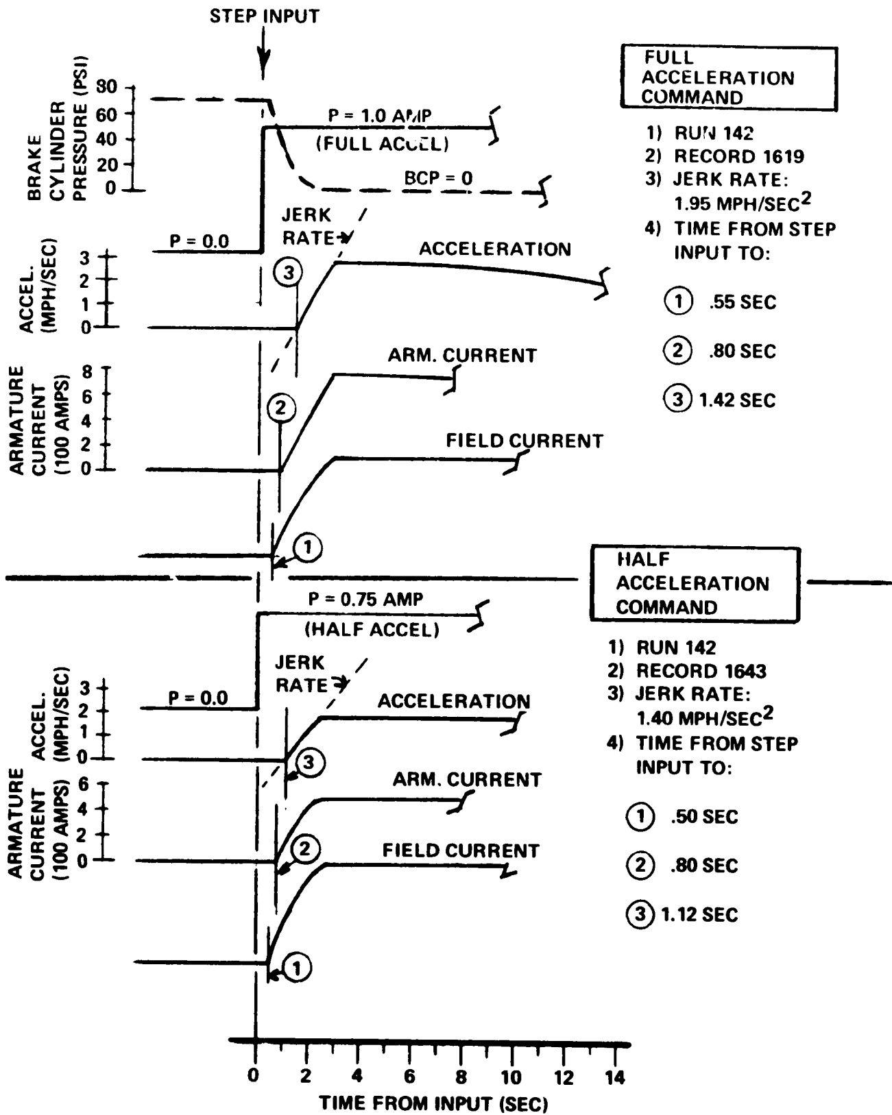
Figure 2-7. Acceleration Deadtime and Jerk Rates (105,000-Pound Car; 600 Volts)
