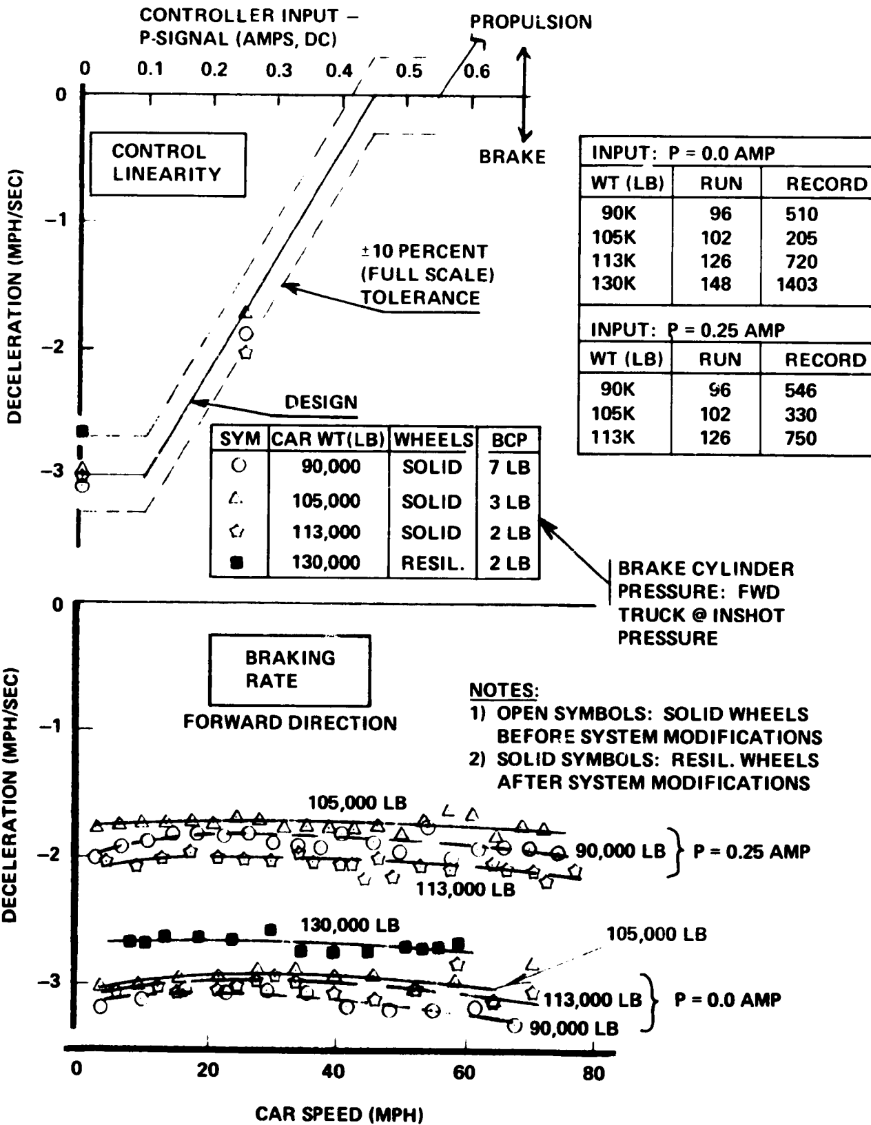
Figure 3-6. Blended Braking Load Weight Compensation
