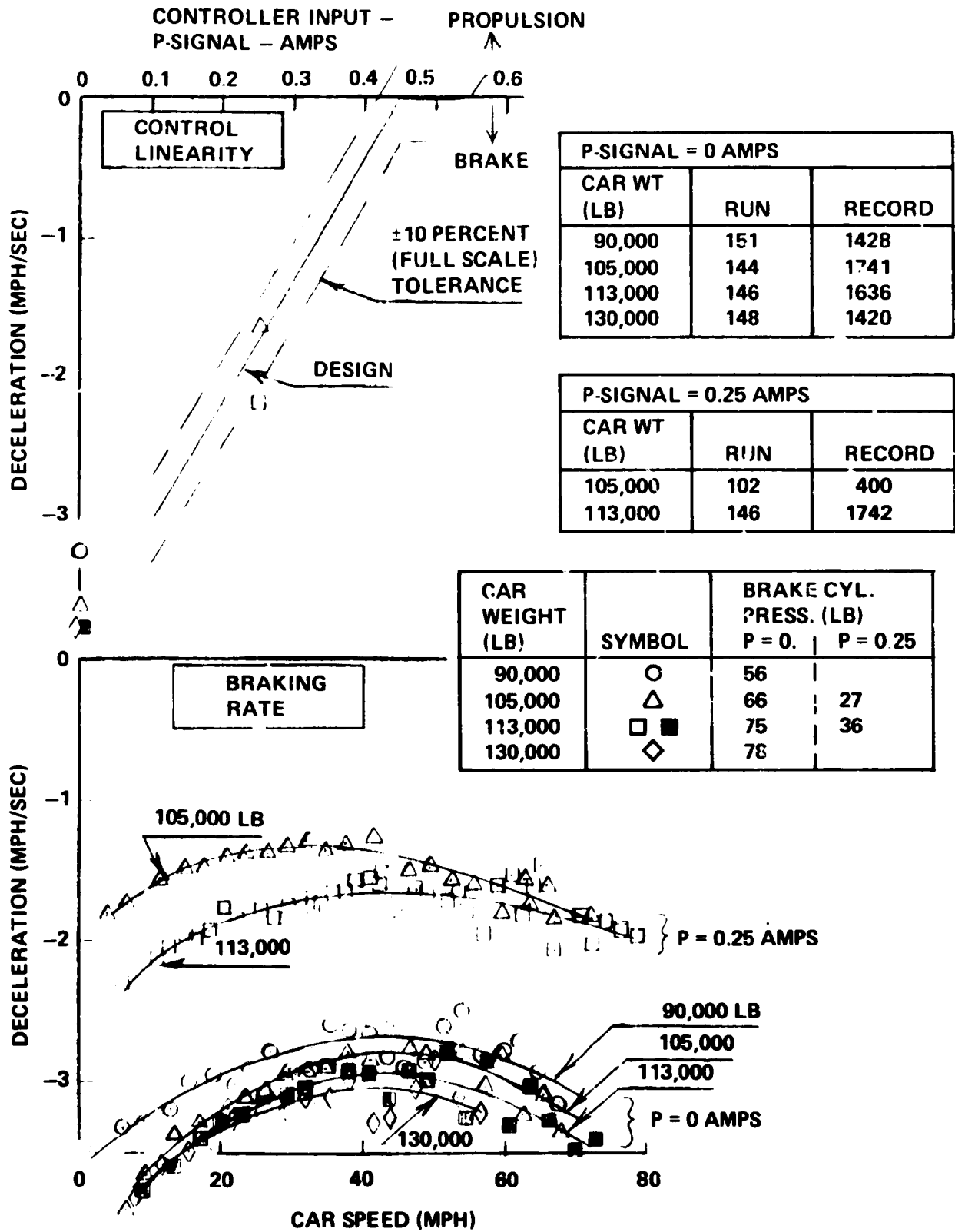
Figure 3-12. Friction-Braking-Only Load Weight Compensation
