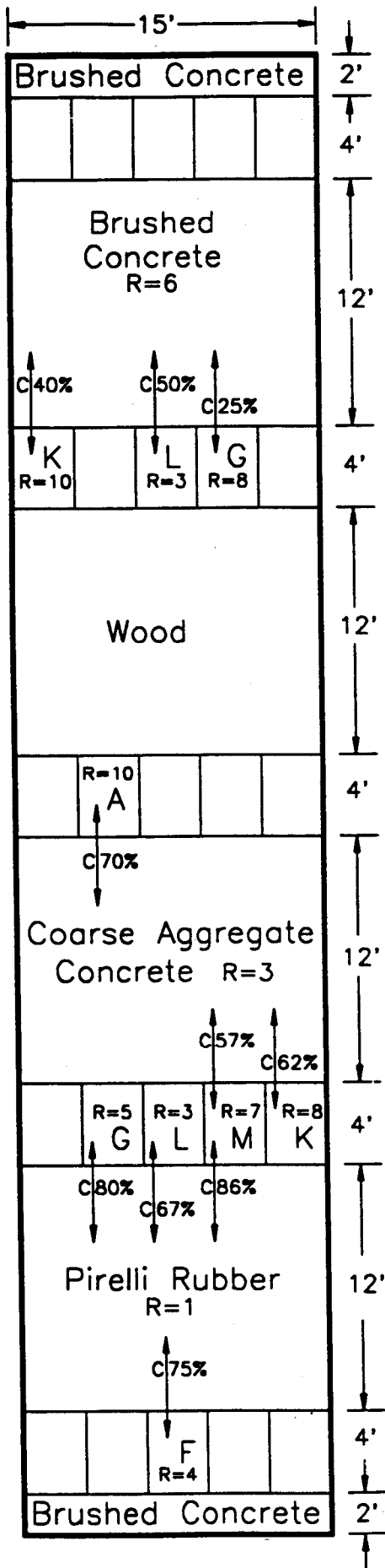
Figure 1-1. Laboratory platform for testing visual contrast of detectable warnings. (Platform originally constructed by Massachusetts Bay Transportation Authority, at old Broadway Station, Boston, for testing underfoot detectability of detectable warning surfaces.)
