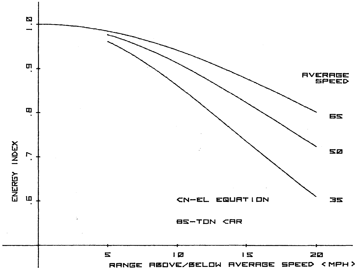
FIGURE 5-3. COMPARISON OF CONSTANT VELOCITY WITH CYCLING BETWEEN TWO VELOCITIES: 85-TON TTX CAR, CN-EL RESISTANCE EQUATION
