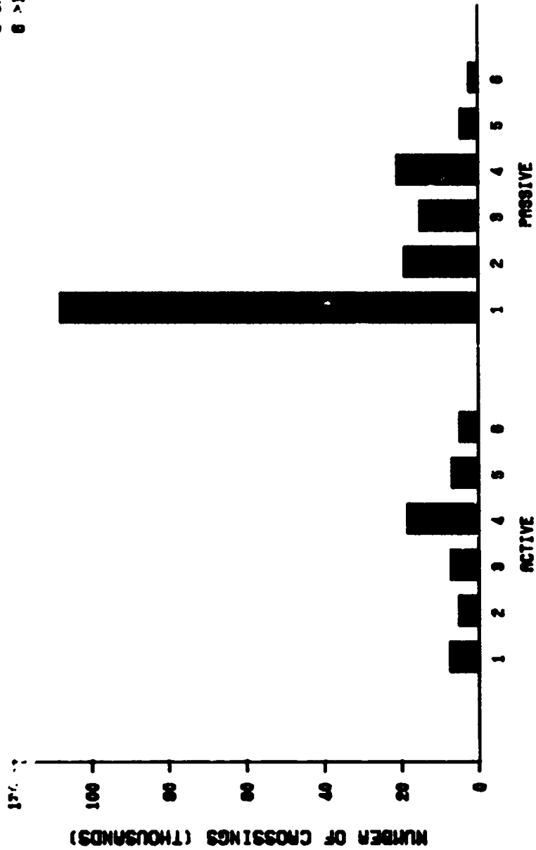
FIGURE 3-23. CROSSINGS BY WARNING DEVICE GROUP (ACTIVE/PASSIVE) VS. ANNUAL AVERAGE DAILY TRAFFIC
