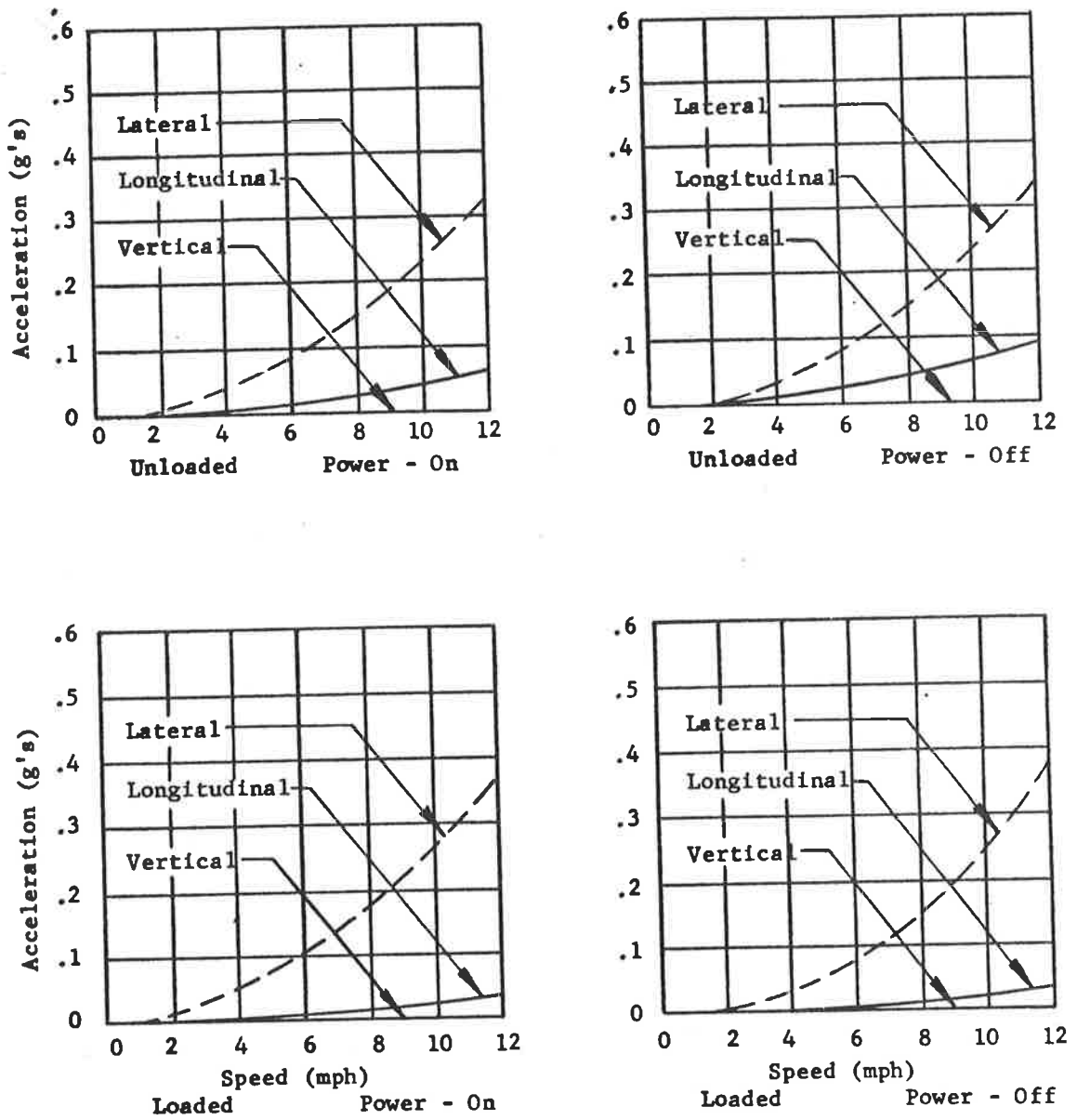
Maximum Accelerations at CG of Vehicle For Various Test Conditions - Zone 3
