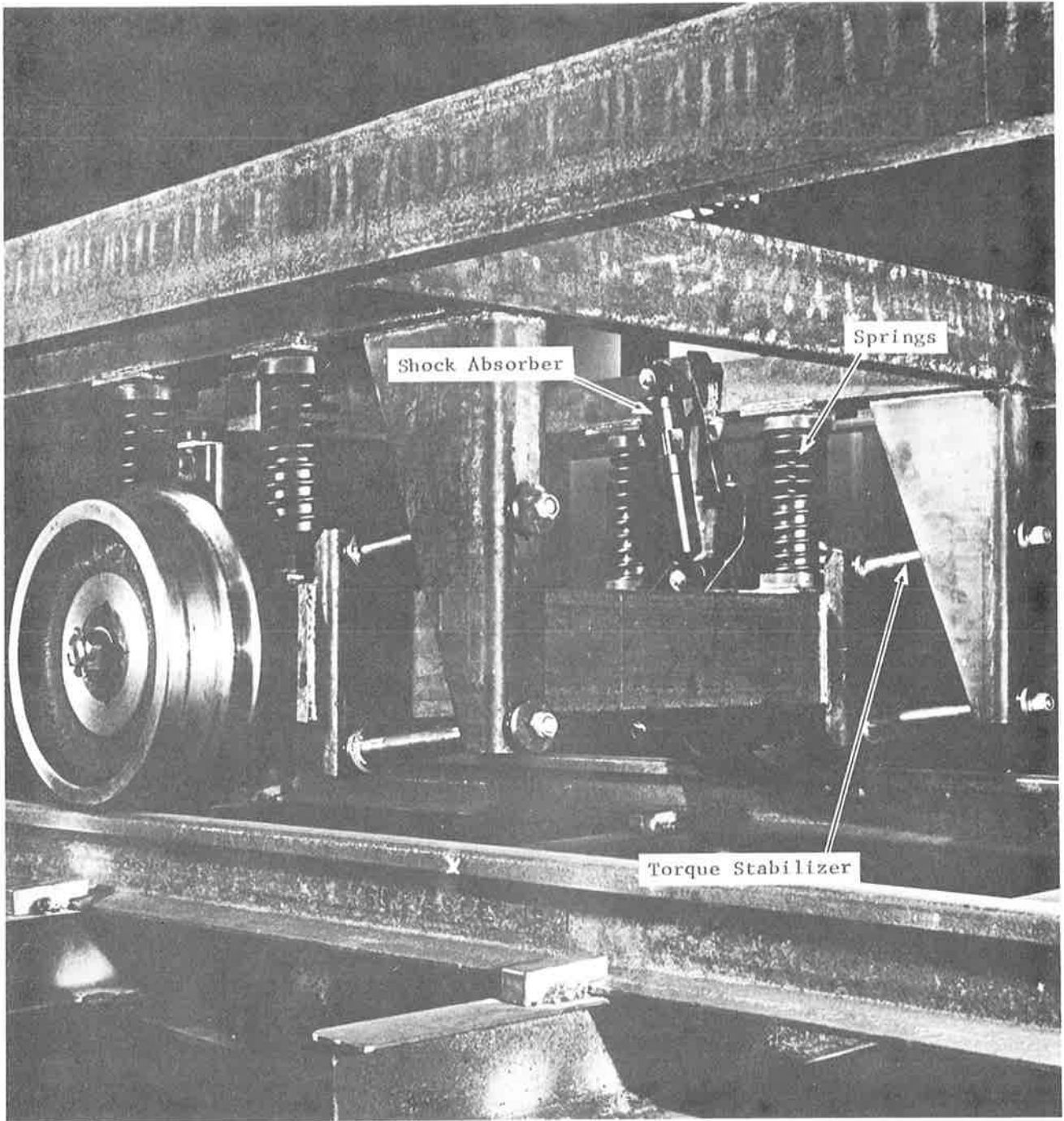
Vehicle Suspension System
