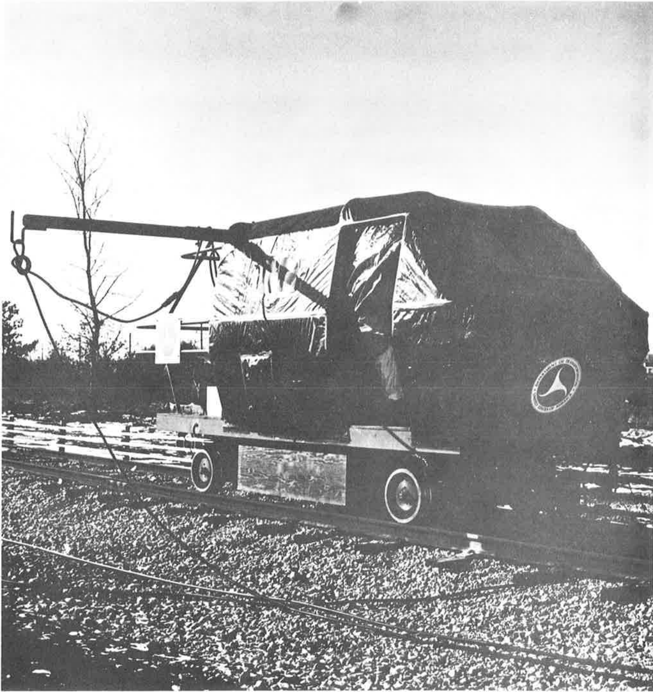
Umbilical Cord Arrangement for Power Off Mode Tests
