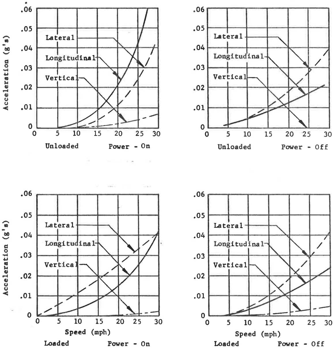
Maximum Accelerations at CG of Vehicle For Various Test Conditions - Zone 1
