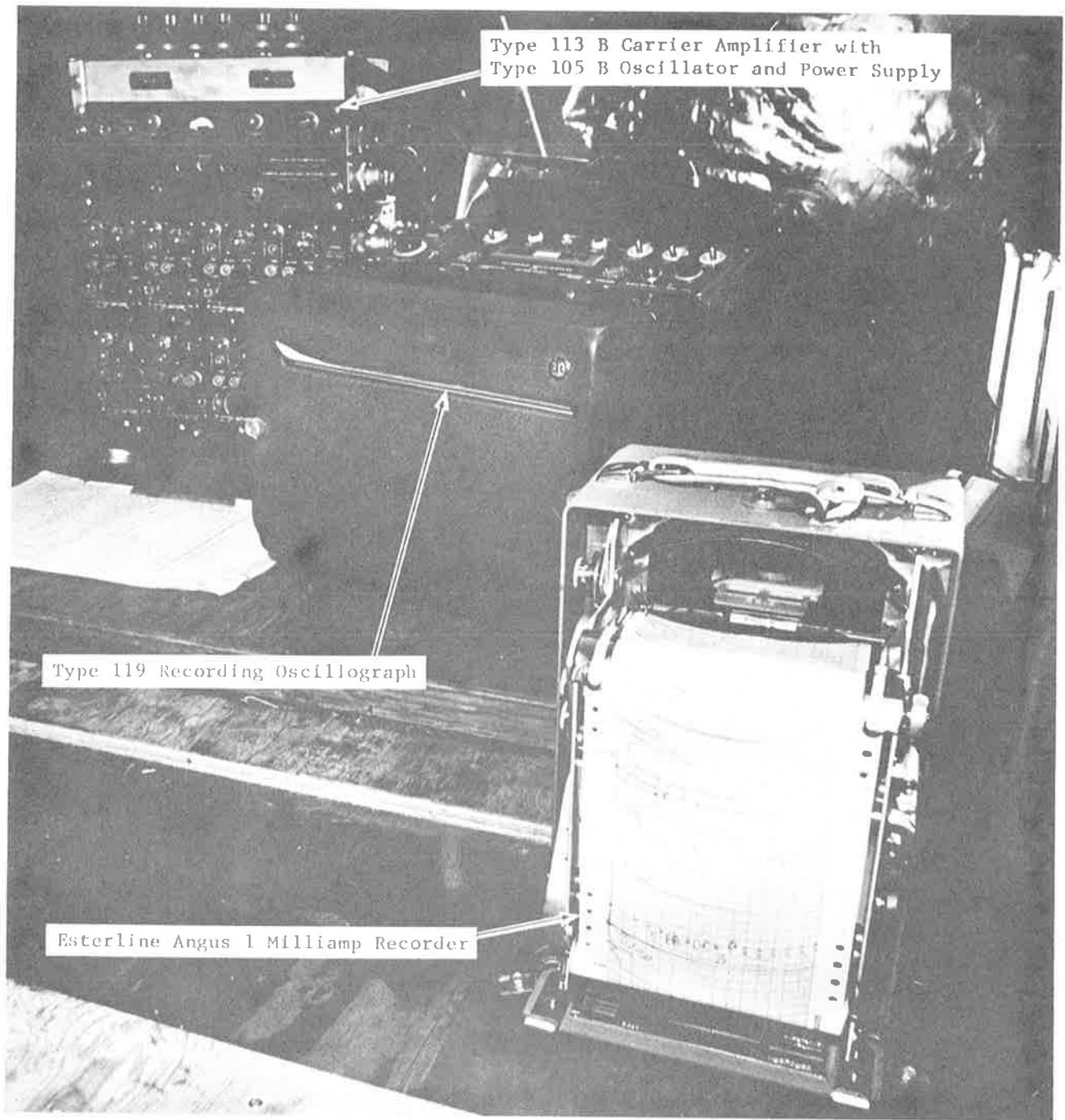
Instrumentation on Test Vehicle
