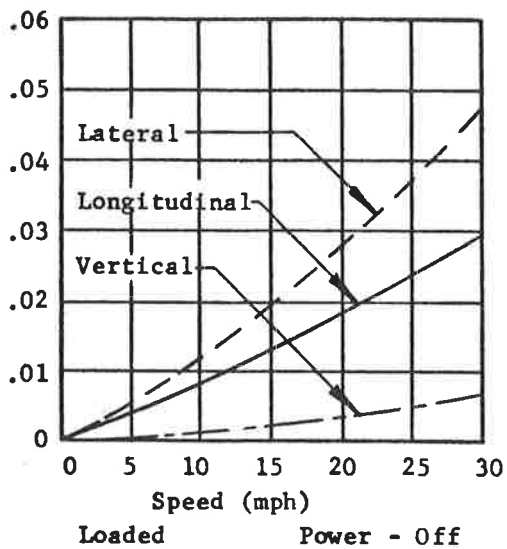
Maximum Accelerations at CG of Vehicle For Various Test Conditions - Zone 2
