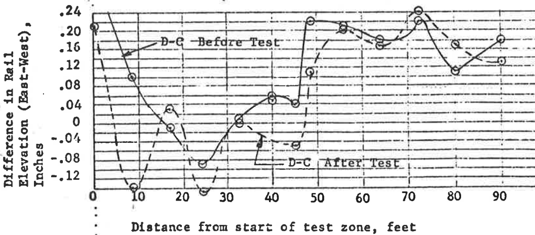
Track alignment, gage, level and cross elevation for test Zone 1 before and after testing
