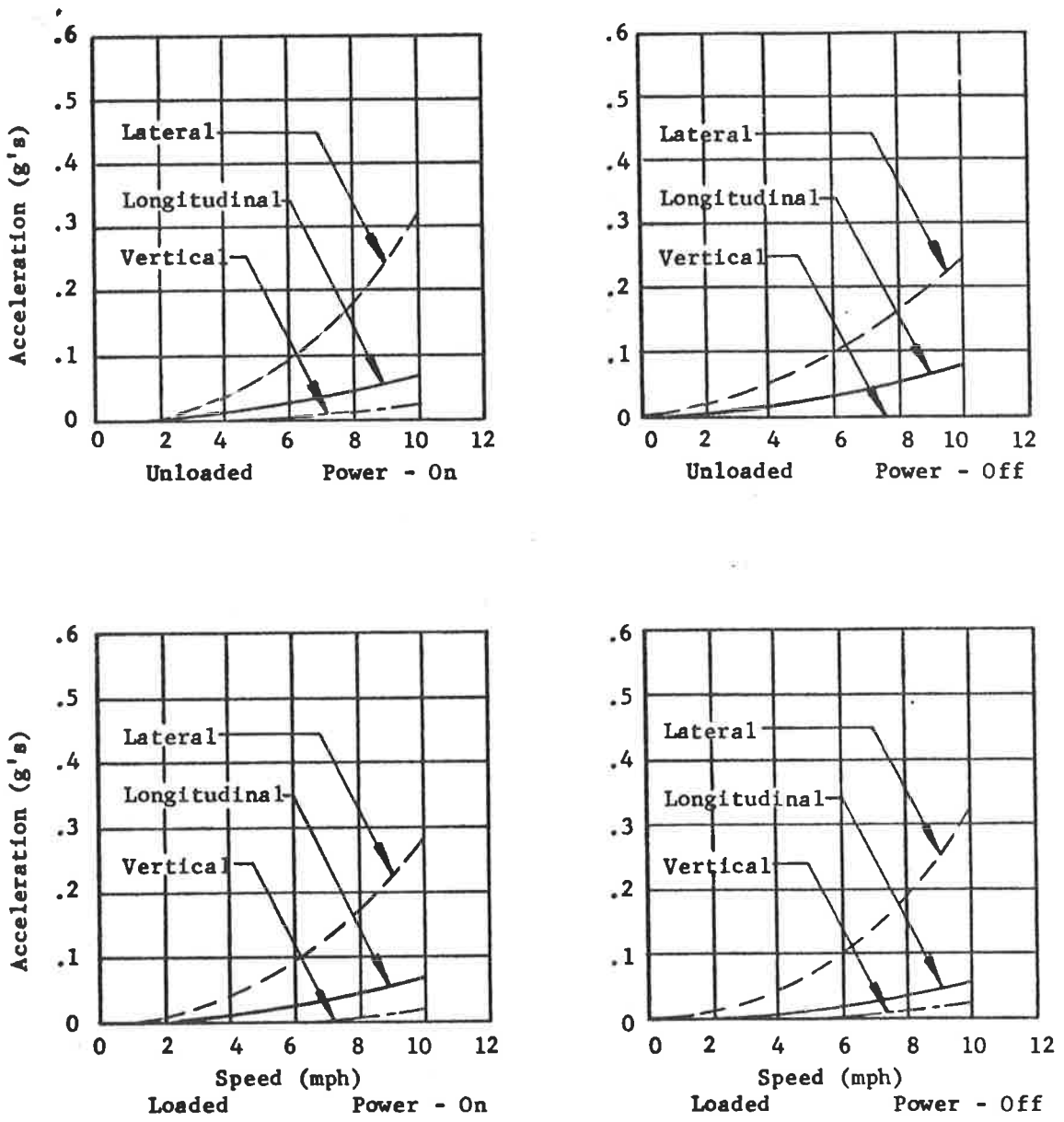
Maximum Accelerations at CG of Vehicle For Various Test Conditions - Zone 5
