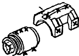
X - Typical thermocouple locations
