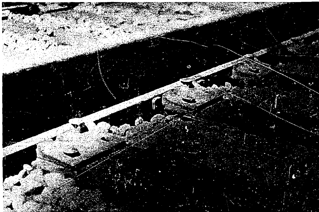
METAL SHIMS BETWEEN TIE AND TIE PLATE
