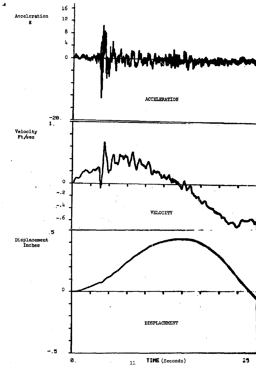
FIGURE D-9. LEADING END SILL MOTION DUE TO PASSING OVER 3/4" SHIMS AT 55 MPH
