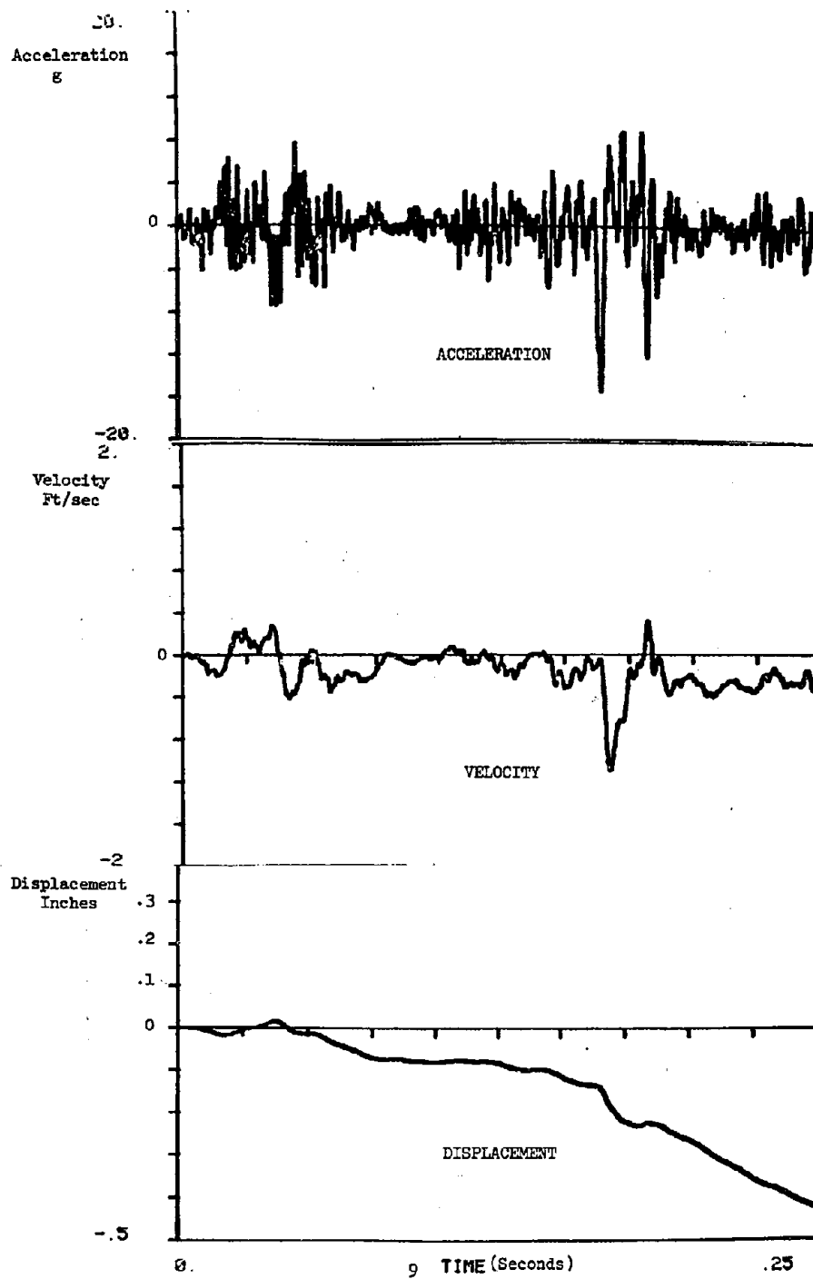
FIGURE D-7. SIDEFRAME MOTION DUE TO PASSING OVER A SWITCH AT 55 MPH
