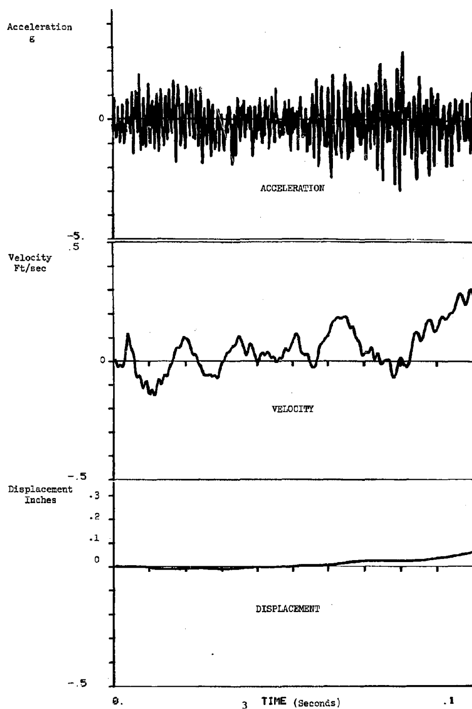
FIGURE D-1. SIDEFRAME MOTION RIDING OVER SMOOTH TRACK
