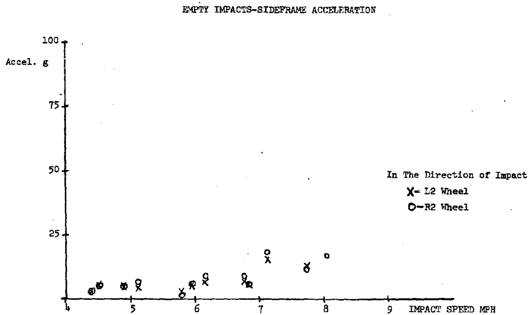
FIGURE A-3 COUPLING IMPACT SUMMARY PLOTS
