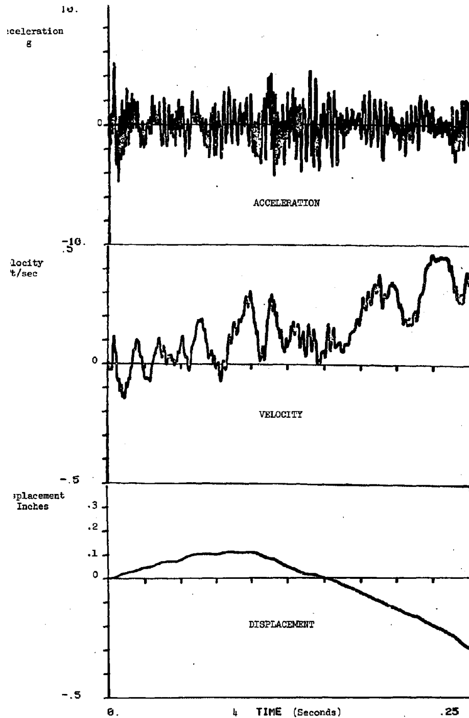
FIGURE D-2. SIDEFRAME MOTION DUE TO TRACK IRREGULARITY
