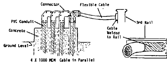
FIGURE 2-3 TYPICAL TUNNEL INSTALLATION FIGURE 2-4 THIRD RAIL CONNECTION DETAILS
