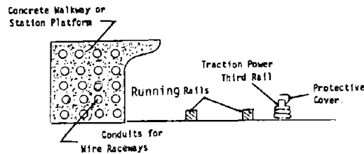
FIGURE 2-6. TYPICAL UNDERGROUND INSTALLATION OF WIRE AND CABLE
