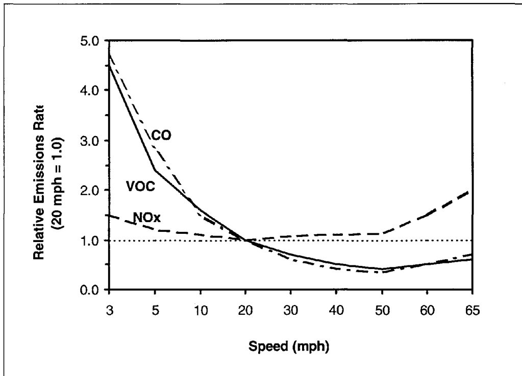
Figure F-2. Relationship of Emissions Rates to Average Speed (Gasoline Automobiles)
