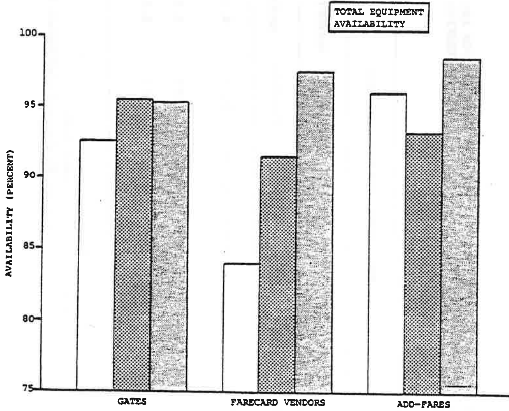
FIGURE 5-2. COMPARISON OF AFC EQUIPMENT AVAILABILITIES: 1978-1979 SURVEY (PRE-RETROFIT) AND 1980 SURVEY (RETROFIT A & B)
