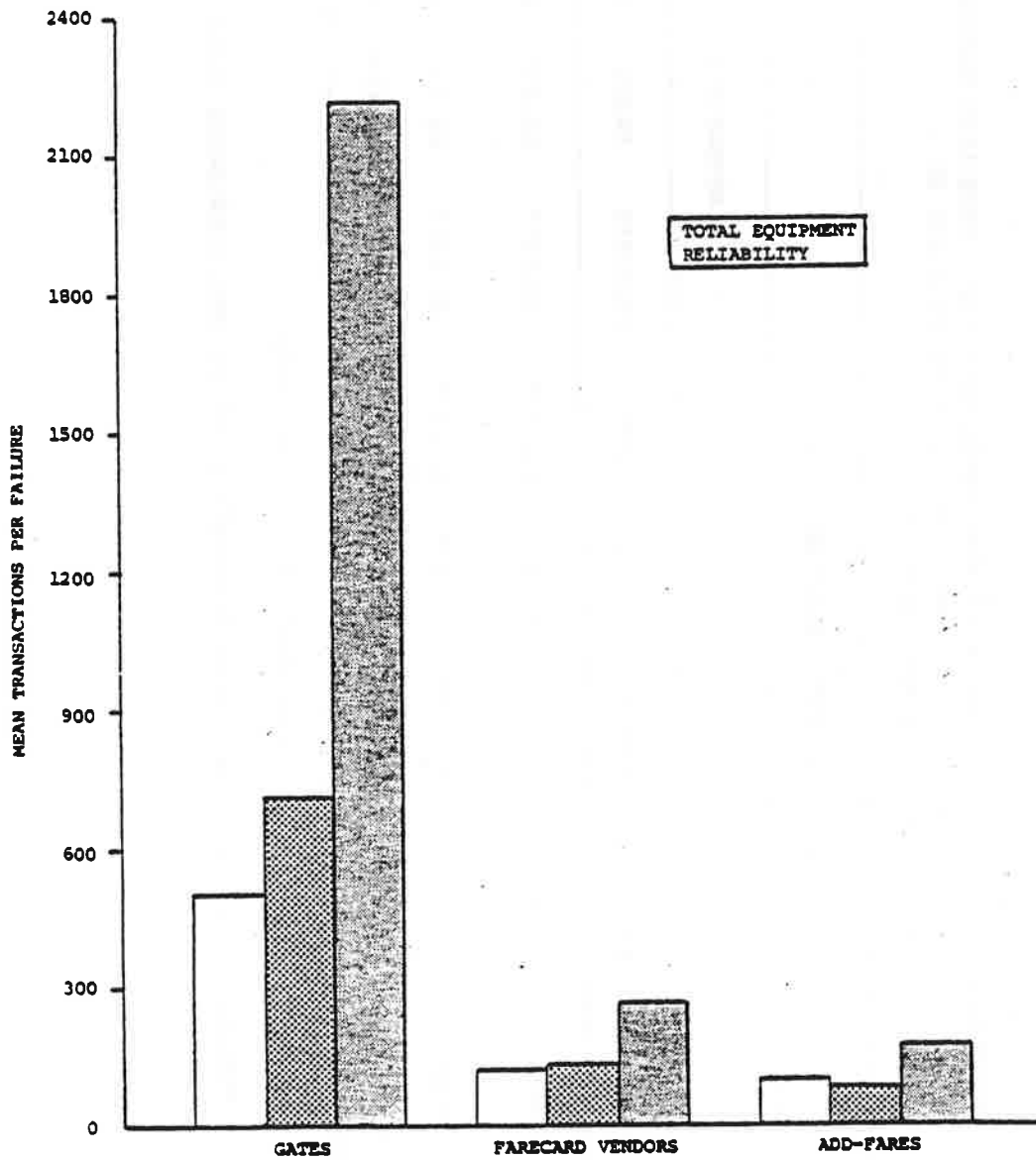
FIGURE 5-1. COMPARISON OF MEAN TRANSACTIONS PER FAILURE FOR AFC EQUIPMENT: 1978-1979 SURVEY (PRE-RETROFIT) AND 1980 SURVEY (RETROFITS A & B)
