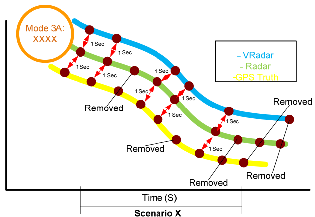
Figure 15. Matching Time Elements in a Flight Test
