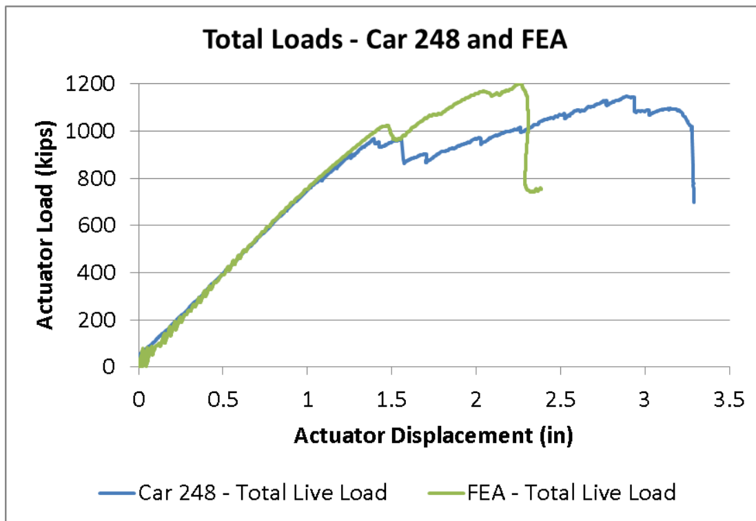
Figure 73. Total Live Loads for Test of Car 248 and FE Model
