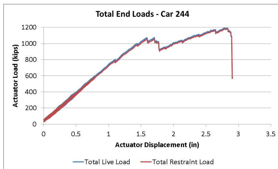
Figure 57. Total End Loads for Car 244 Crippling Test
