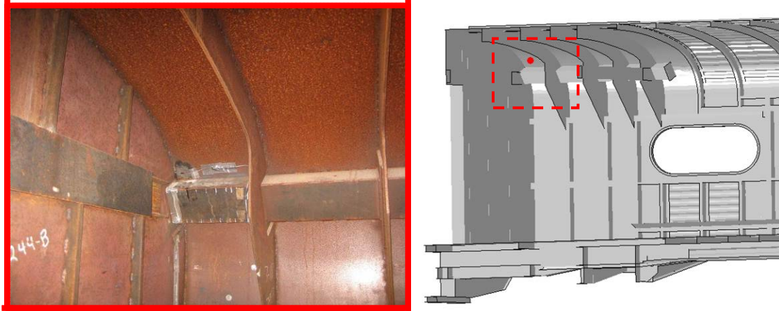
Figure 39. Strain Gage at Roof-Level Energy Absorber Support
