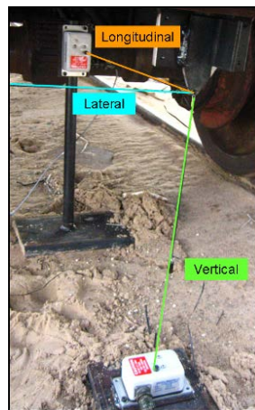
Figure A 3. VLL Array of String Pots
