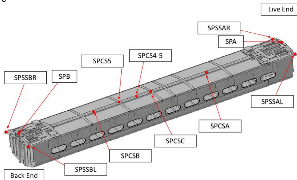
Figure 37. String Pot VLL Arrays on Car 244 (Underside View)
