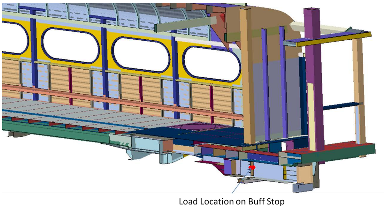
Figure 16. Loading Location on Live End Buff Stop, 800-kip FE Model
