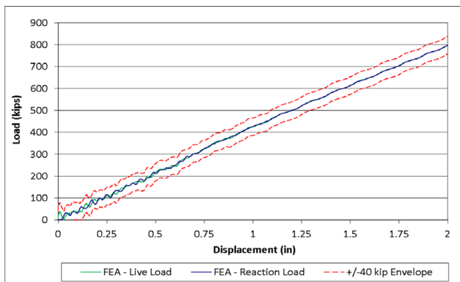
Figure 18. Live Load and Reaction Load with \pm 40 kip Envelope, 800-kip Elastic FEA
