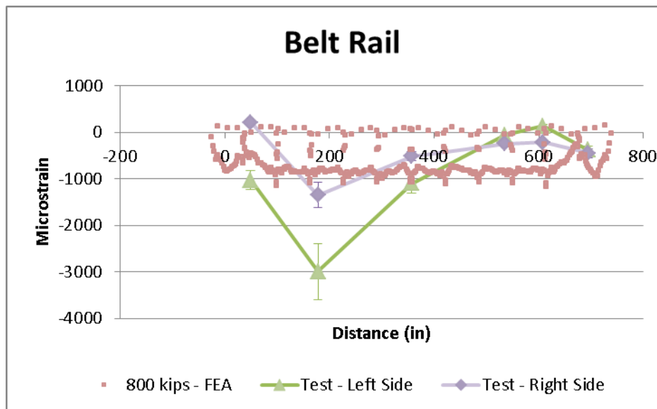
Figure 28. Strain Results in Belt Rail at 800 kips, 800-kip Test and FEA
