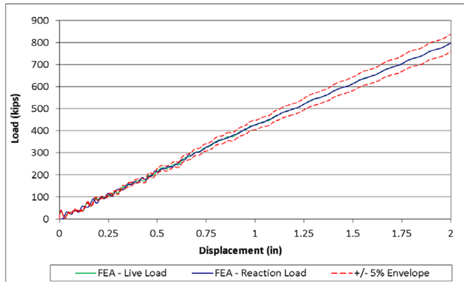
Figure 17. Live Load and Reaction Load with \pm 5\% Envelope, 800-kip Elastic FEA
