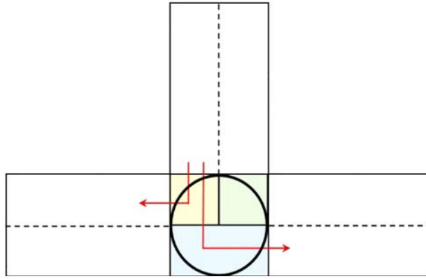
Figure 4.8: Illustration of Radial Division on a Three-Approach Intersection
