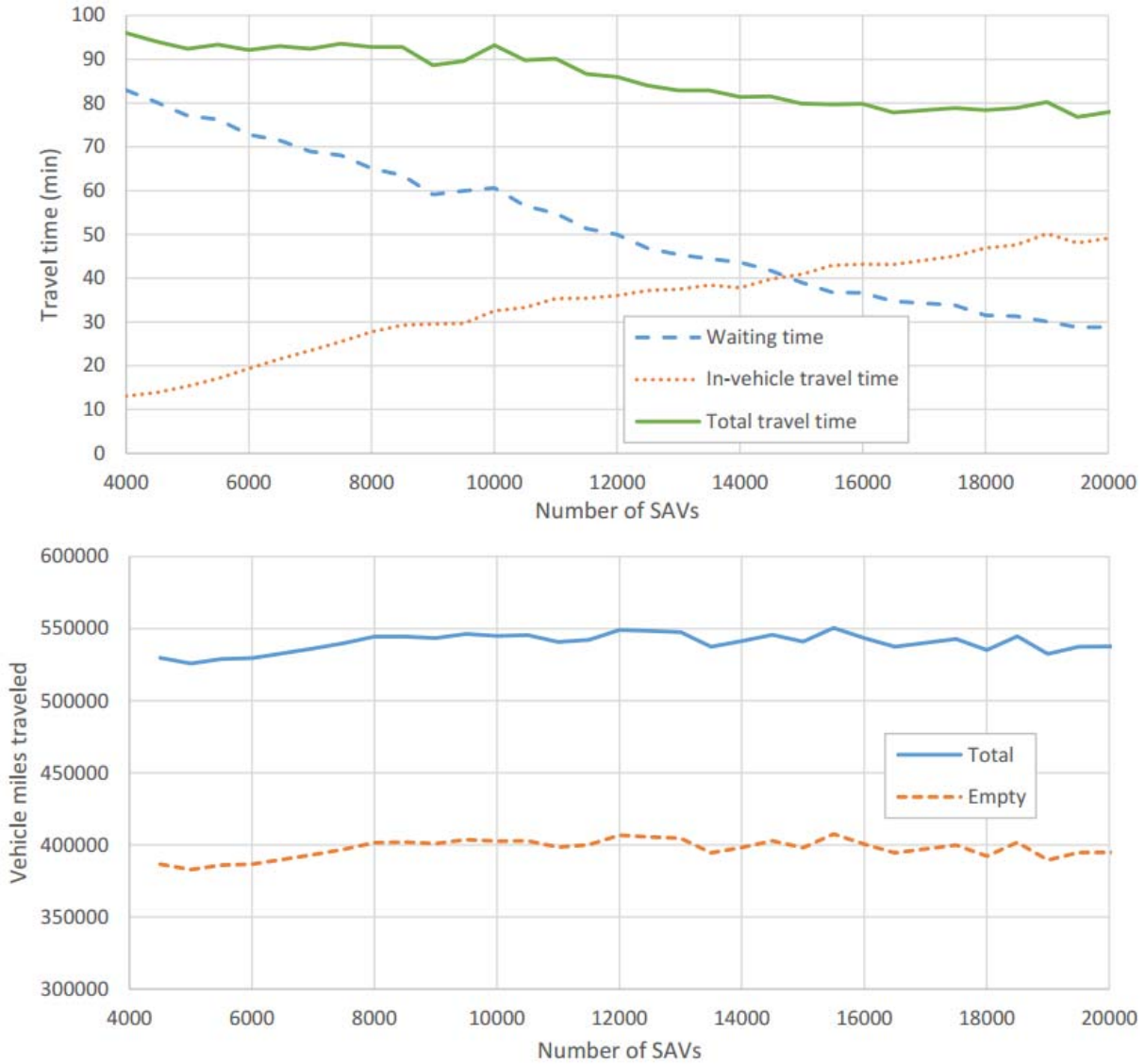
Figure 4.20: Travel Time and VMT for the Preemptive Relocation Scenario
